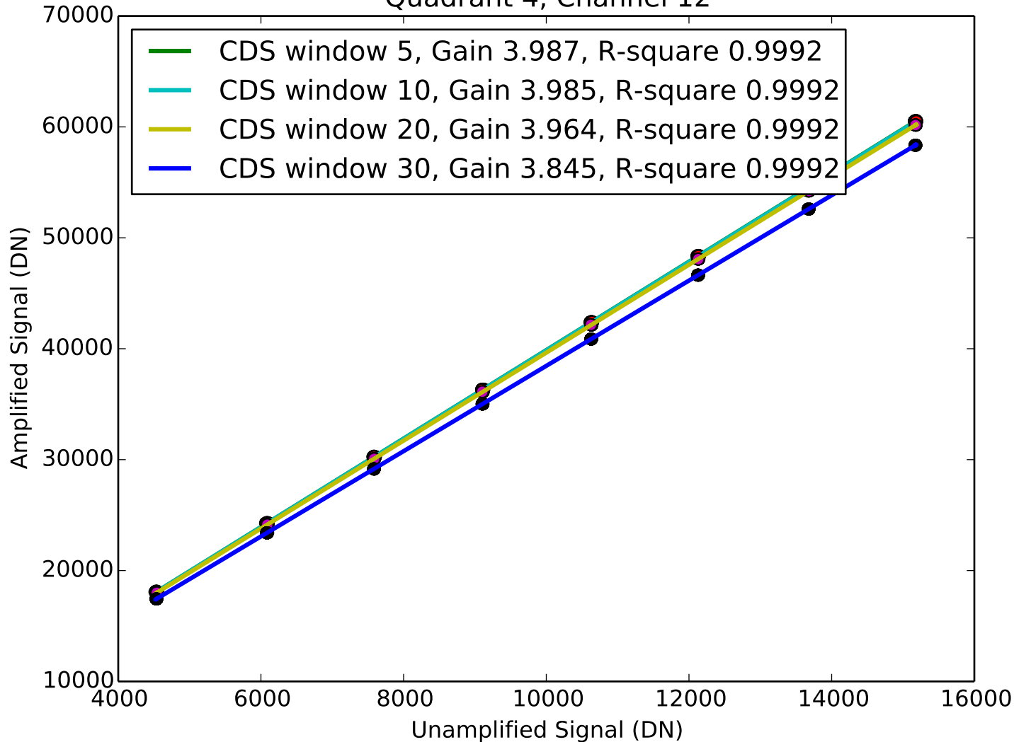
Signal vs Amplified Signal Quadrant 4, Channel 12
