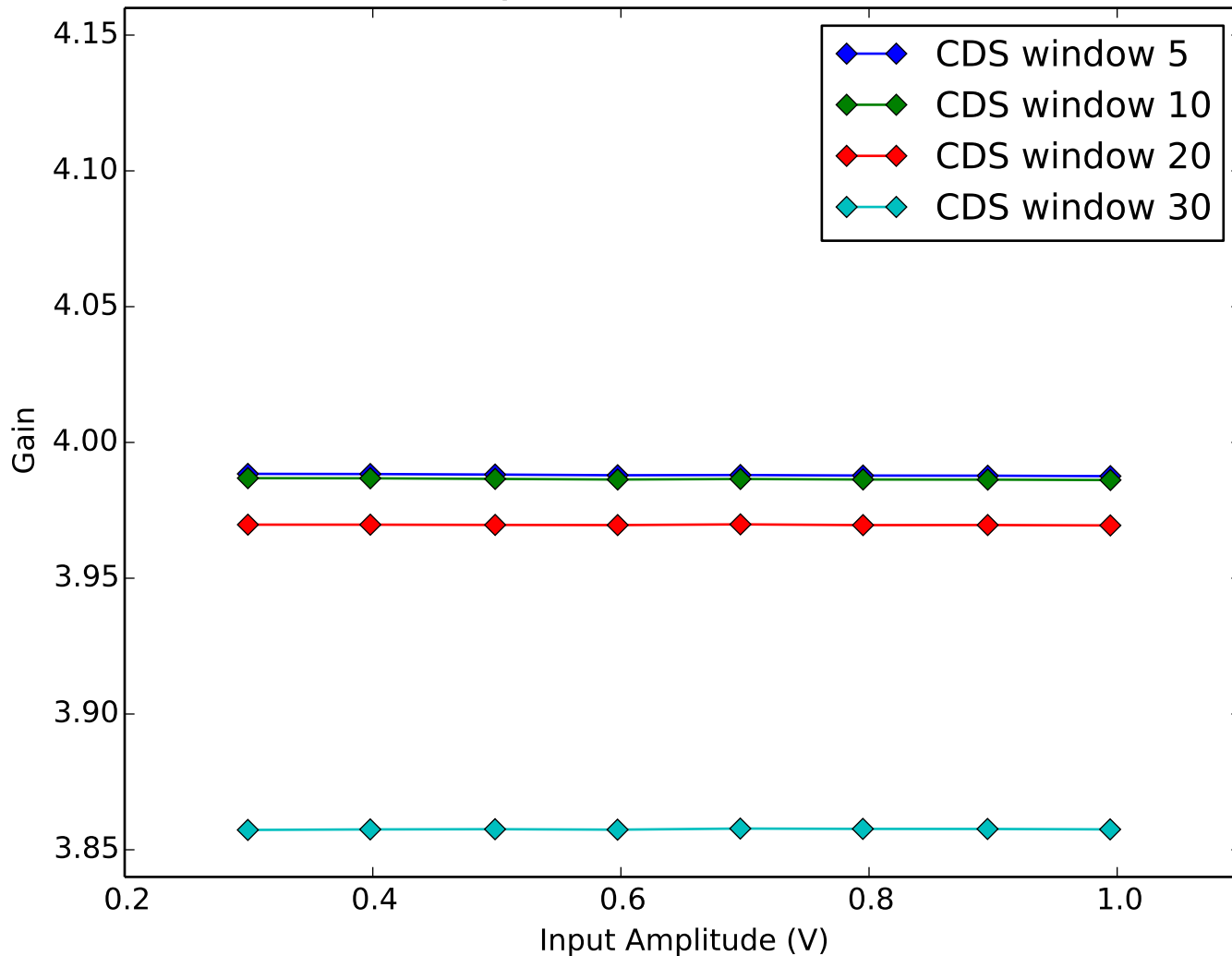
Average Amplifier Gain vs Amplifier Input Amplitude Quadrant 4, Channel 2
