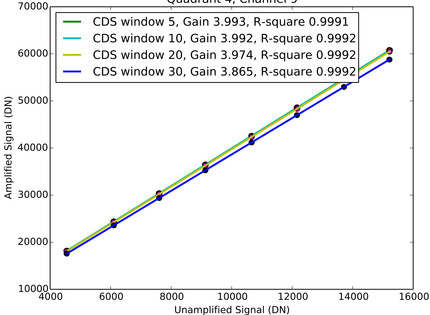
Signal vs Amplified Signal Quadrant 4, Channel 9
