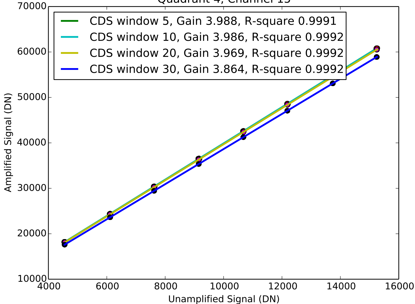
Signal vs Amplified Signal Quadrant 4, Channel 15
