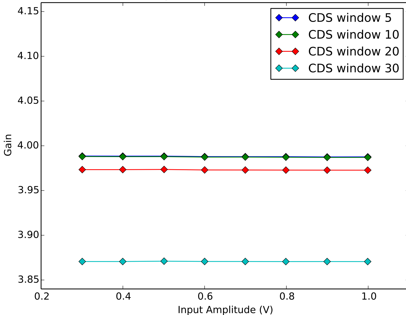
Average Amplifier Gain vs Amplifier Input Amplitude Quadrant 4, Channel 7
