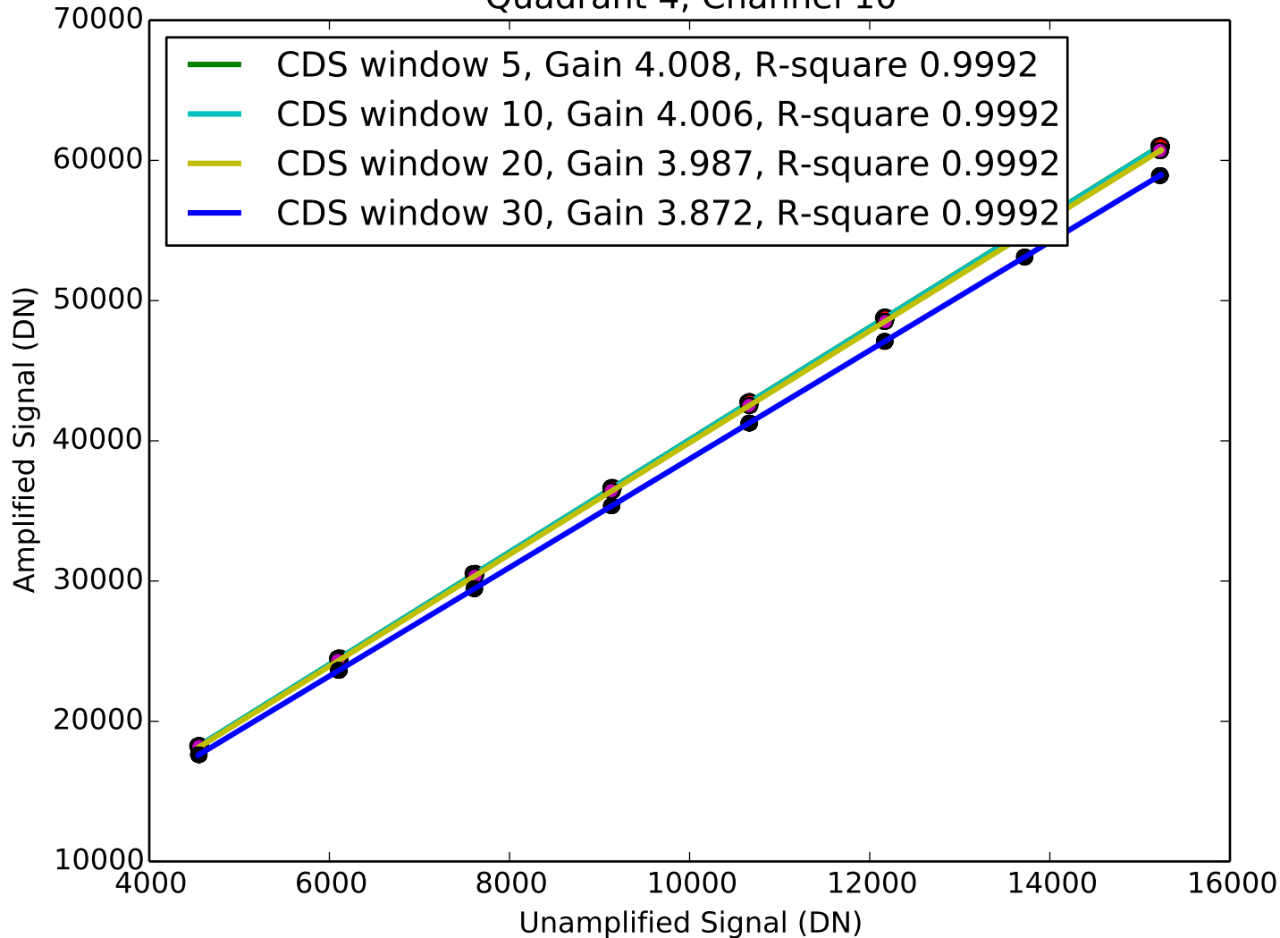
Signal vs Amplified Signal Quadrant 4, Channel 10
