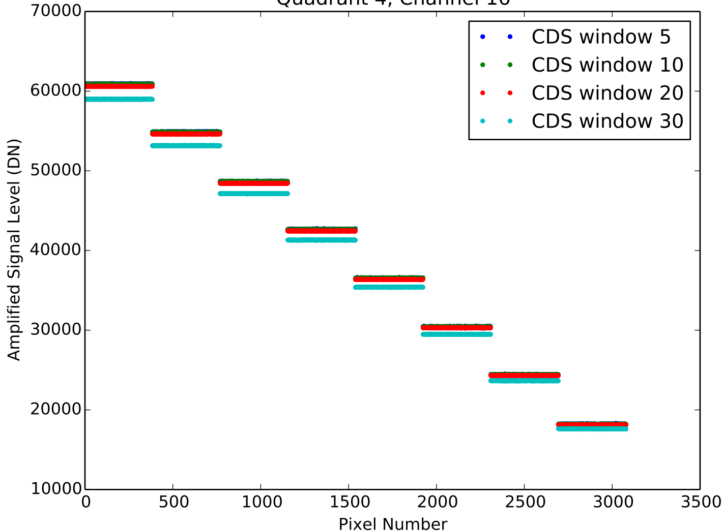
Amplified Signal Level from CDS Quadrant 4, Channel 16
