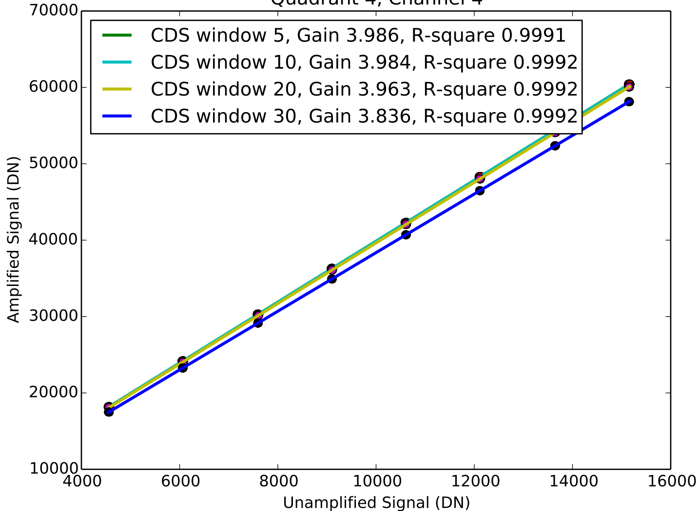
Signal vs Amplified Signal Quadrant 4, Channel 4
