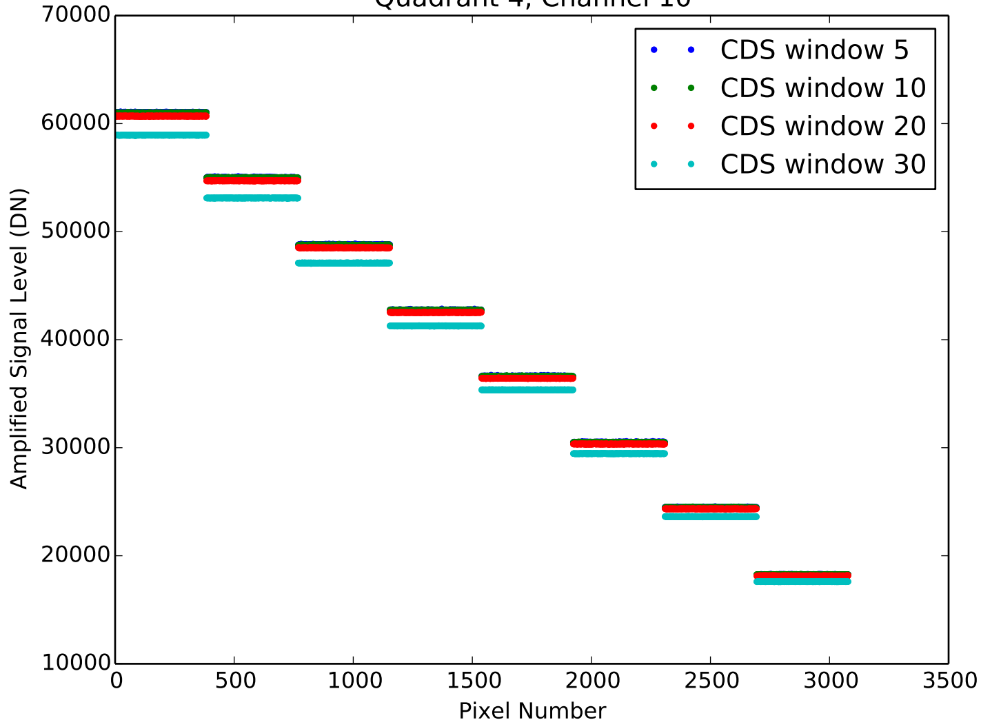
Amplified Signal Level from CDS Quadrant 4, Channel 10
