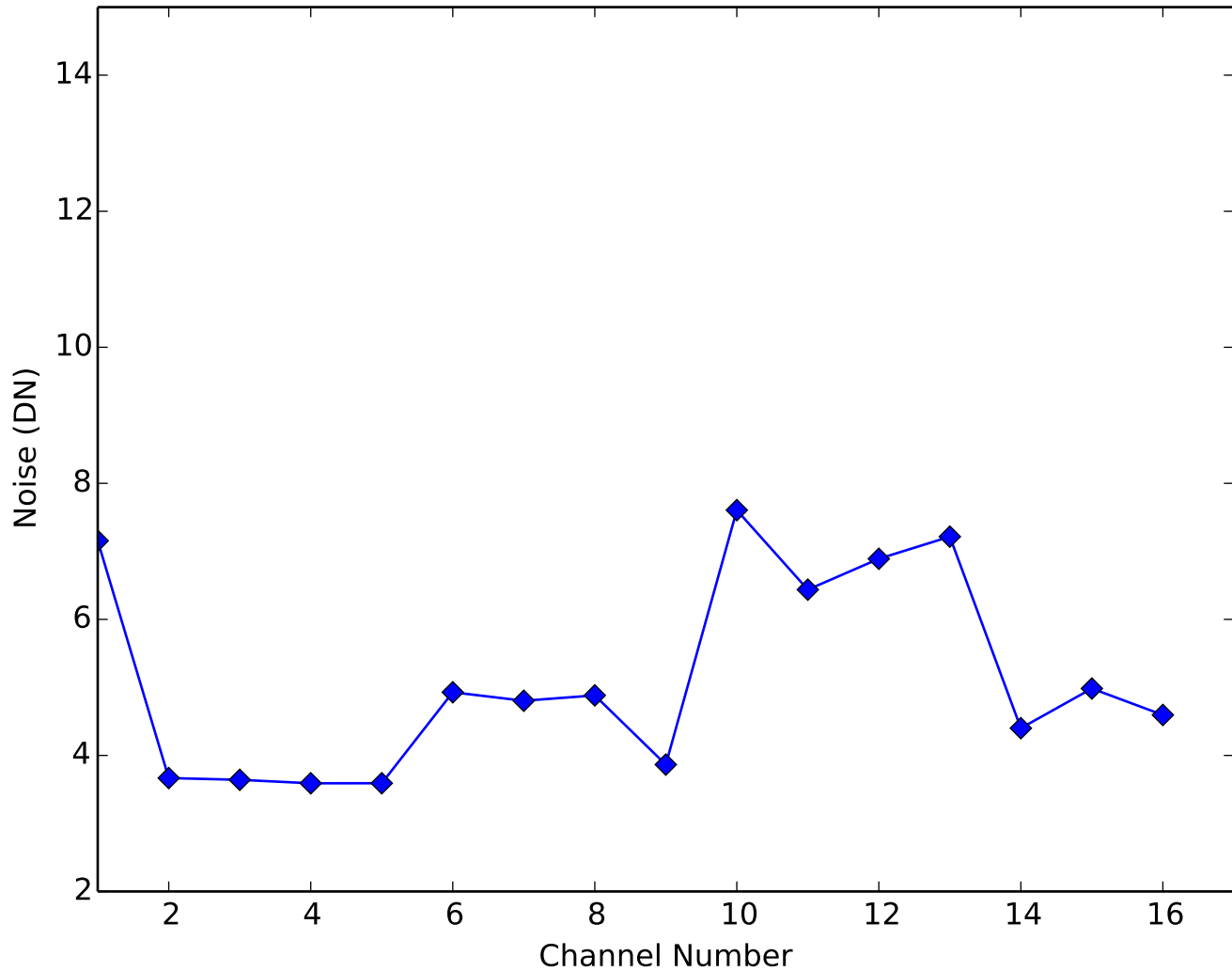
Shorted Input Noise for VIB Amplifiers Quadrant4
