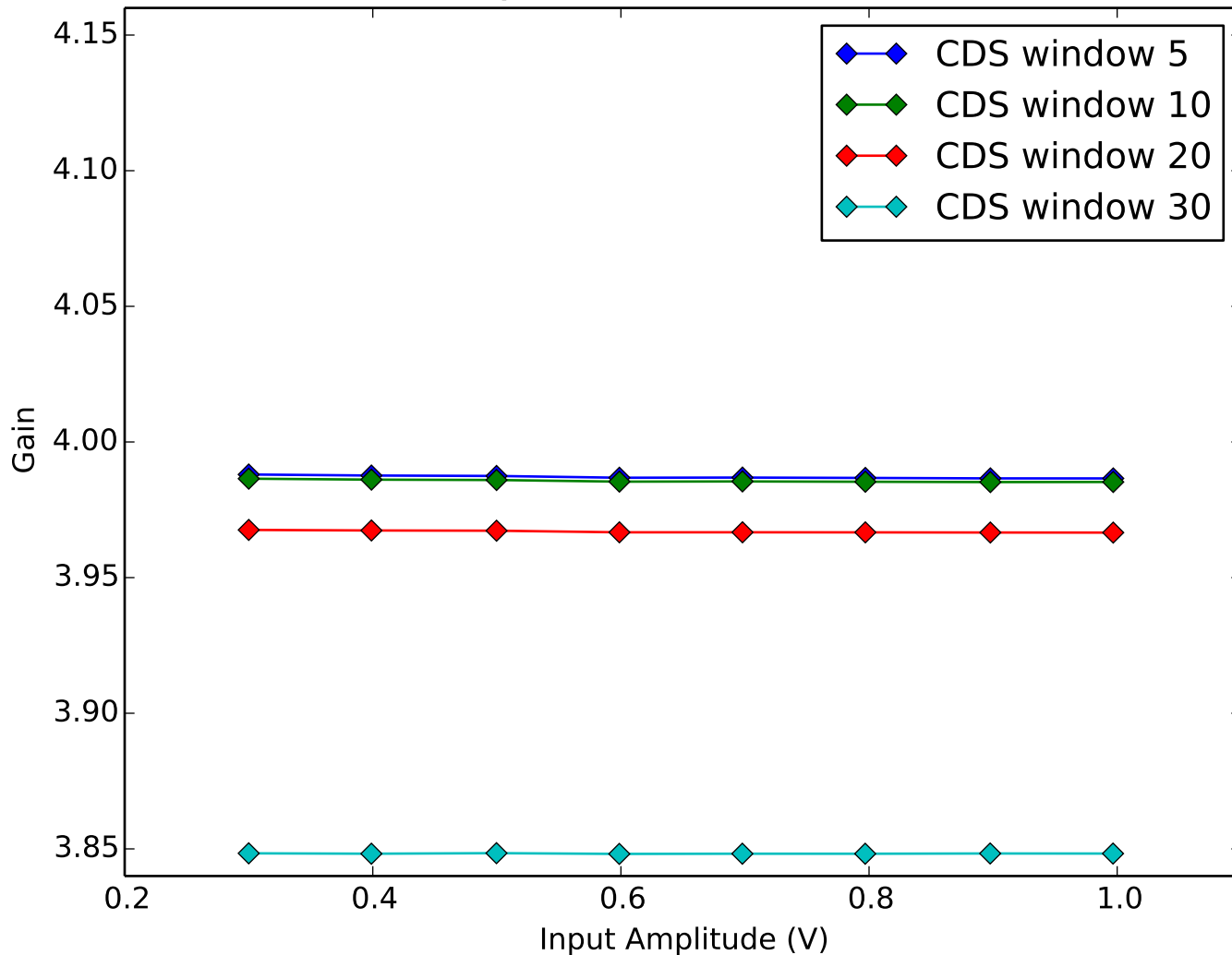
Average Amplifier Gain vs Amplifier Input Amplitude Quadrant 4, Channel 8
