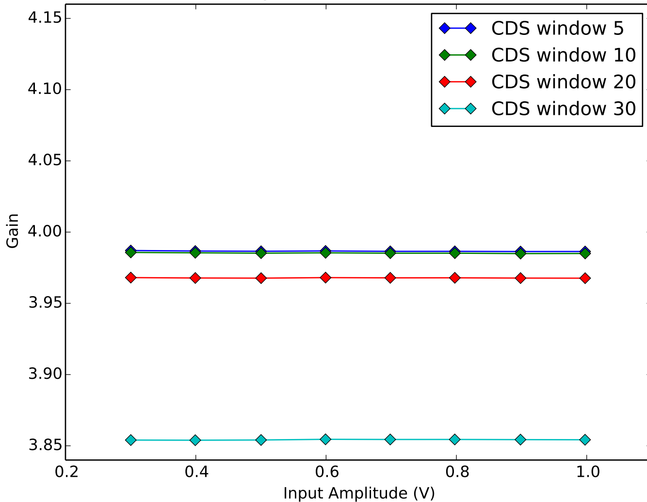
Average Amplifier Gain vs Amplifier Input Amplitude Quadrant 4, Channel 5
