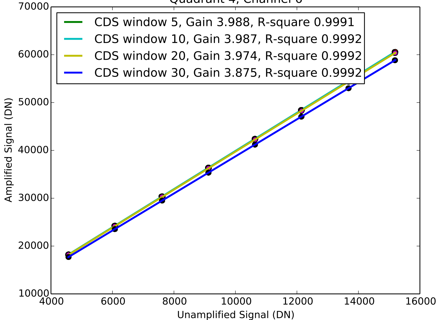
Signal vs Amplified Signal Quadrant 4, Channel 6
