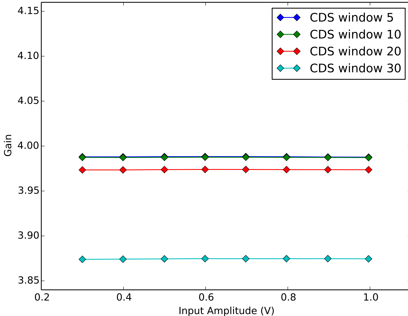
Average Amplifier Gain vs Amplifier Input Amplitude Quadrant 4, Channel 6
