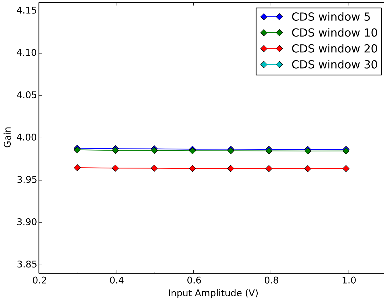
Average Amplifier Gain vs Amplifier Input Amplitude Quadrant 4, Channel 4
