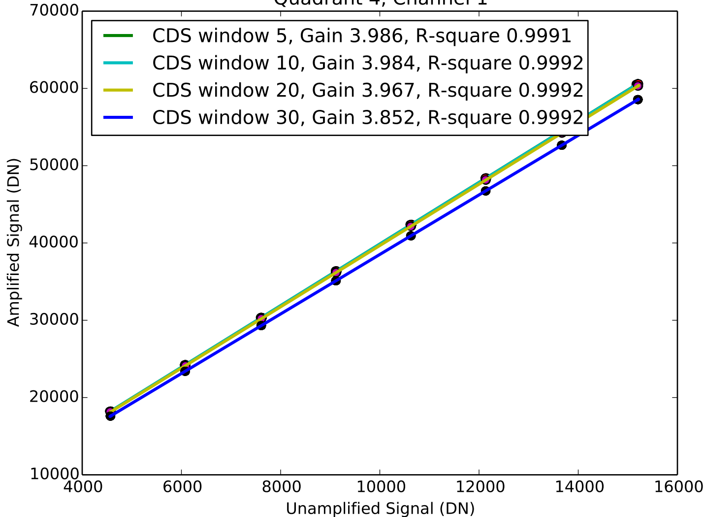
Signal vs Amplified Signal Quadrant 4, Channel 1
