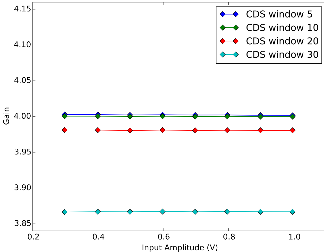
Average Amplifier Gain vs Amplifier Input Amplitude Quadrant 4, Channel 11
