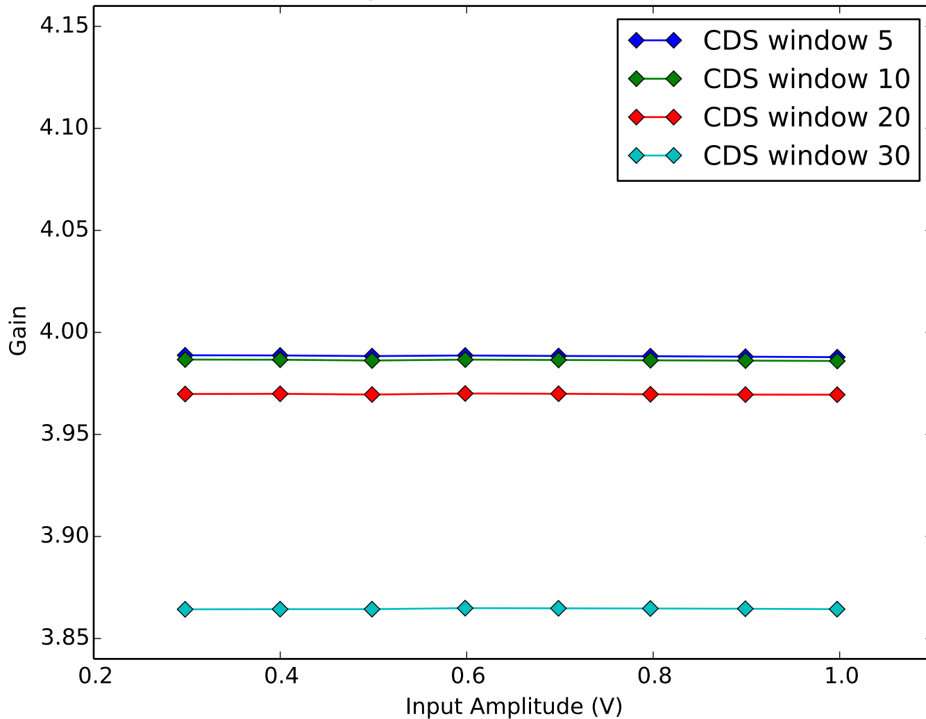
Average Amplifier Gain vs Amplifier Input Amplitude Quadrant 4, Channel 13
