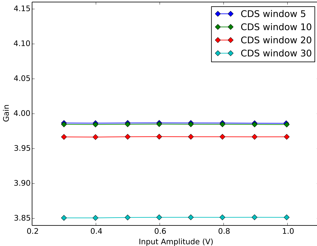
Average Amplifier Gain vs Amplifier Input Amplitude Quadrant 4, Channel 1
