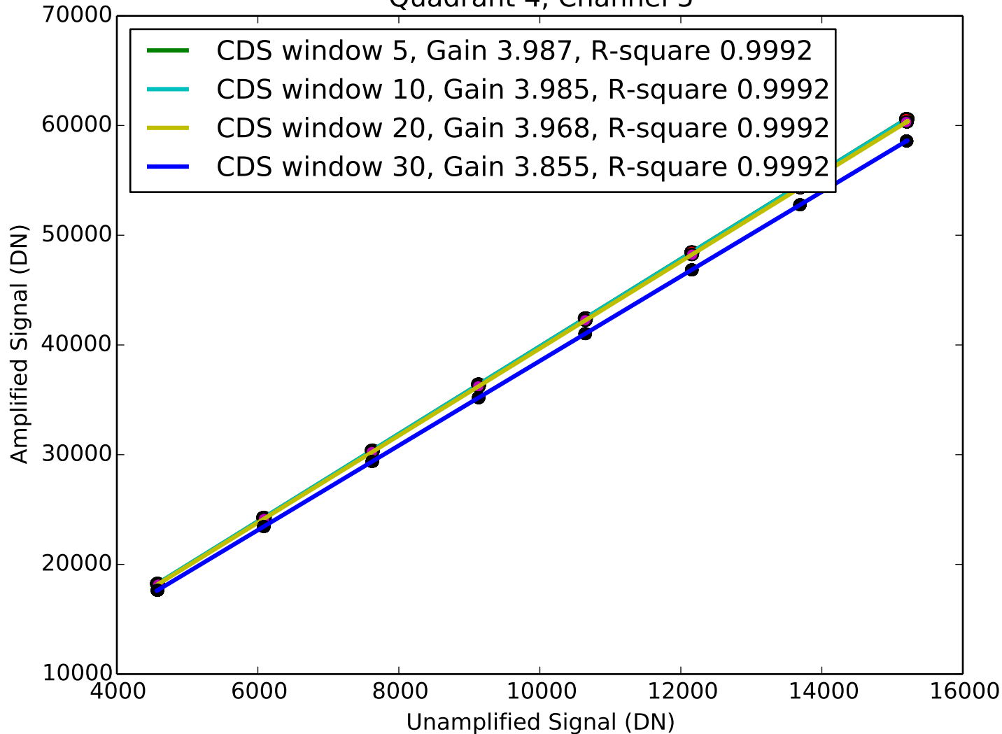
Signal vs Amplified Signal Quadrant 4, Channel 5
