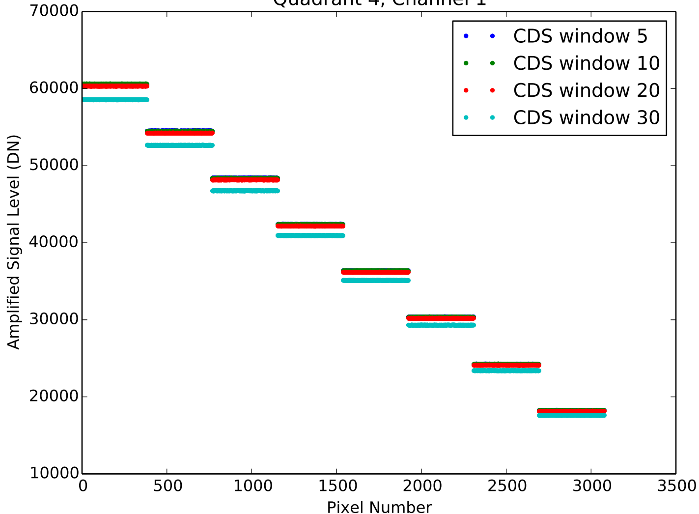
Amplified Signal Level from CDS Quadrant 4, Channel 1
