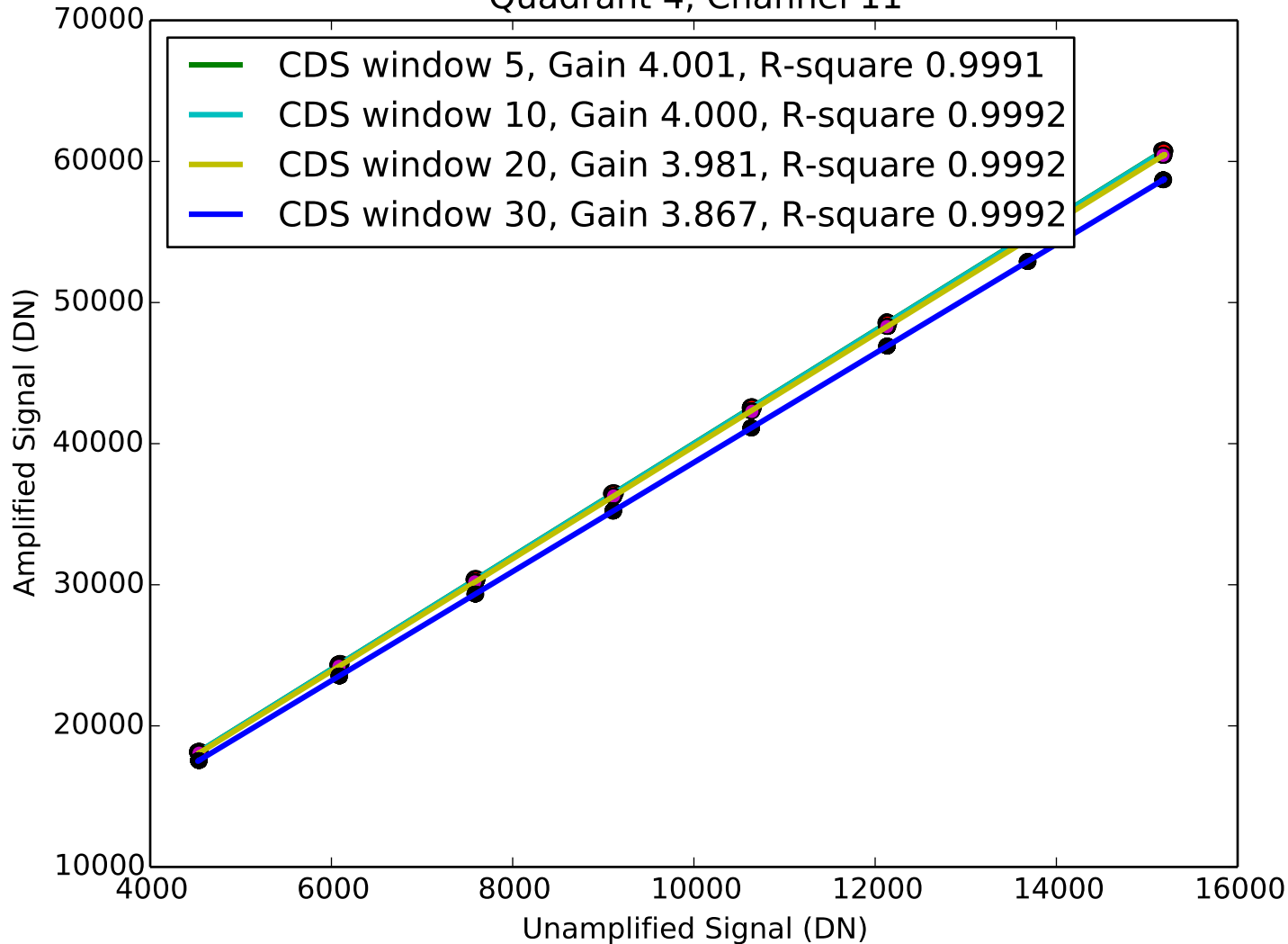
Signal vs Amplified Signal Quadrant 4, Channel 11
