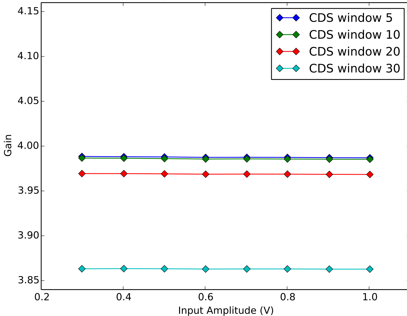
Average Amplifier Gain vs Amplifier Input Amplitude Quadrant 4, Channel 16
