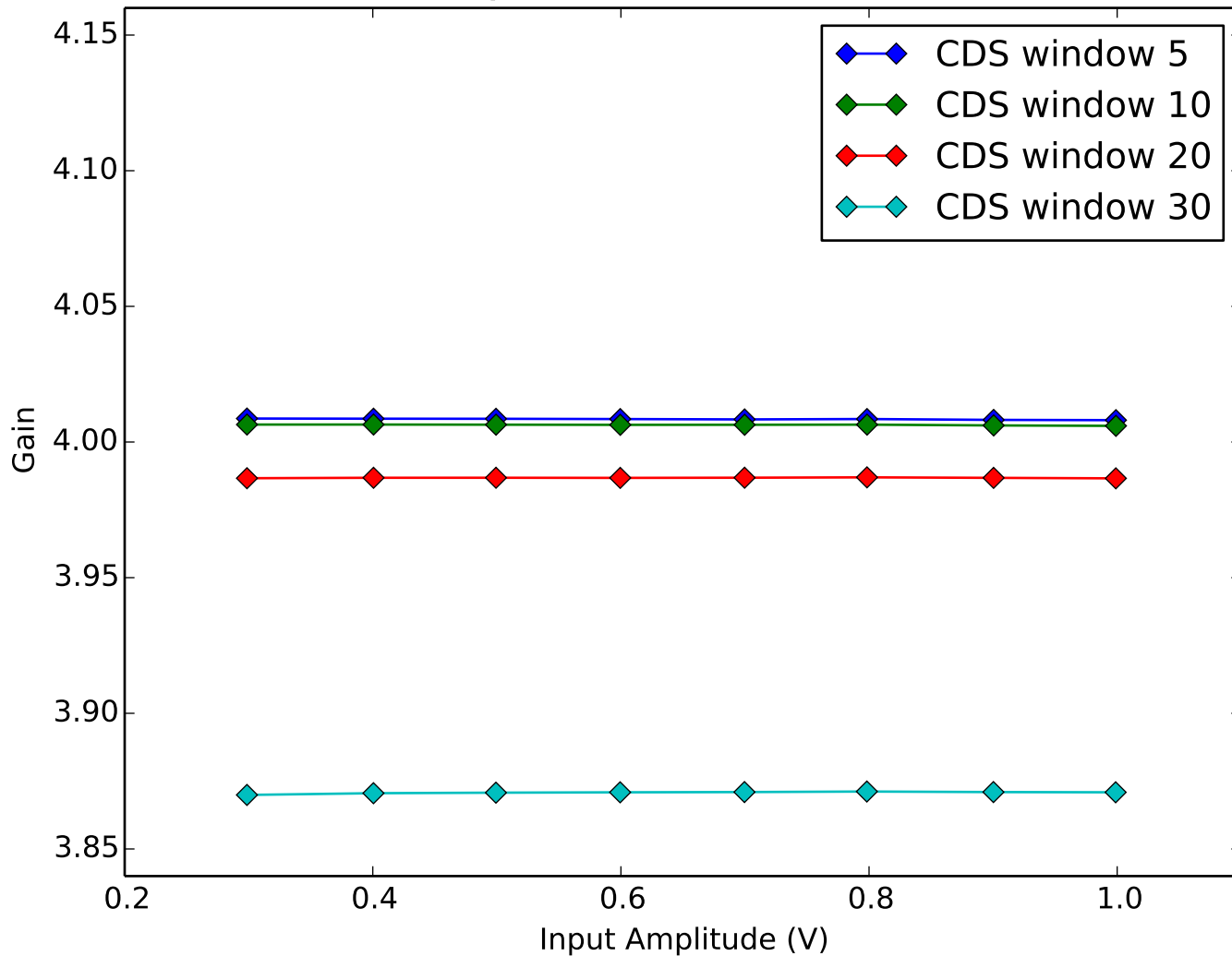
Average Amplifier Gain vs Amplifier Input Amplitude Quadrant 4, Channel 10
