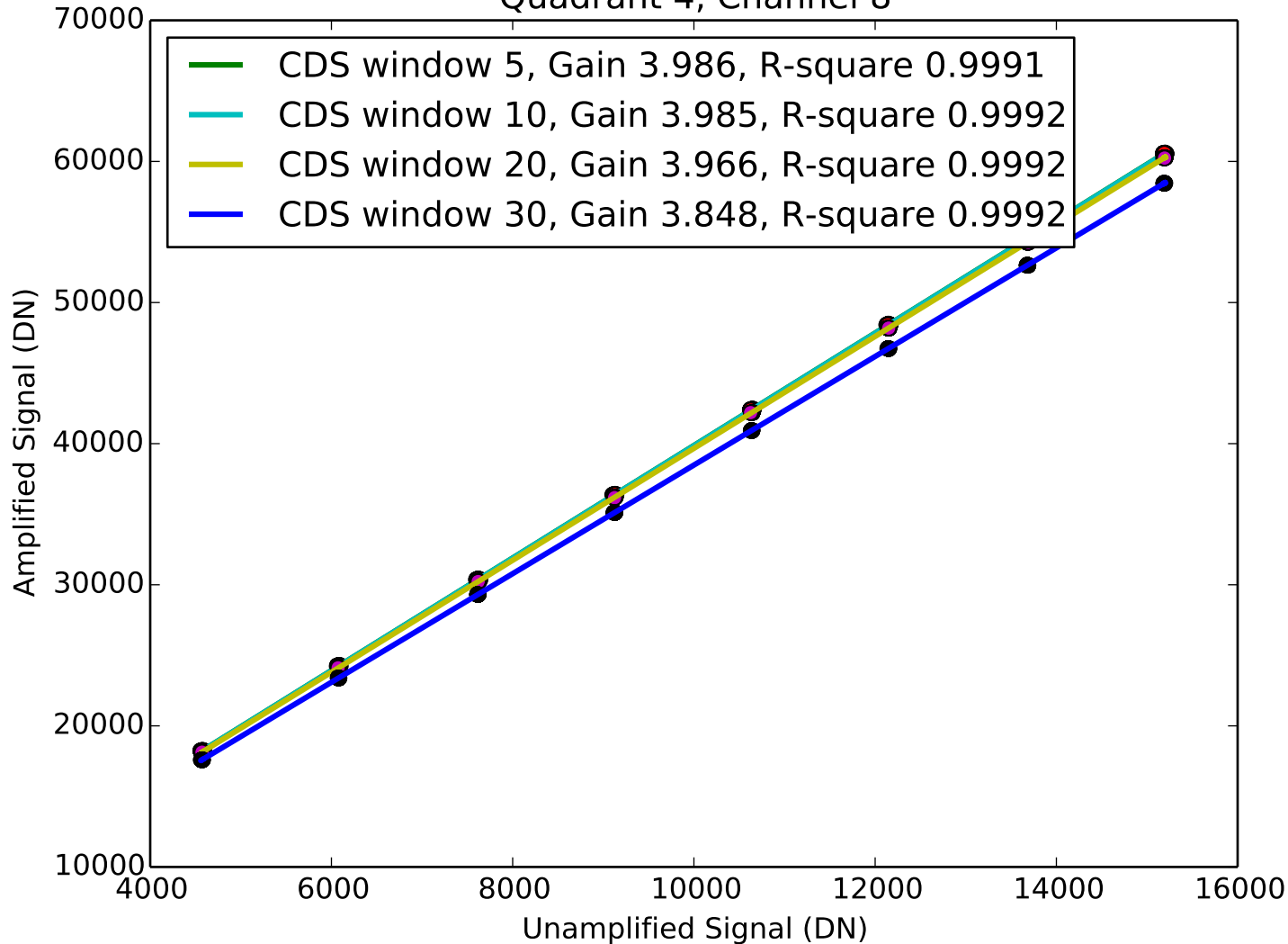
Signal vs Amplified Signal Quadrant 4, Channel 8
