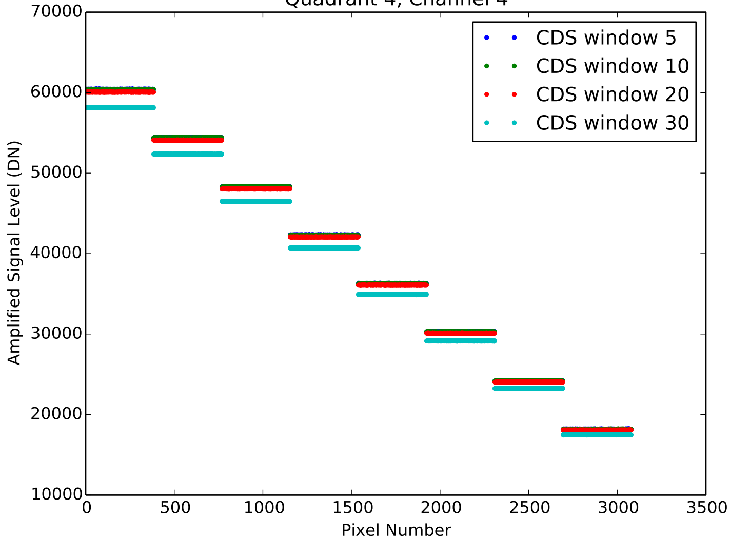
Amplified Signal Level from CDS Quadrant 4, Channel 4
