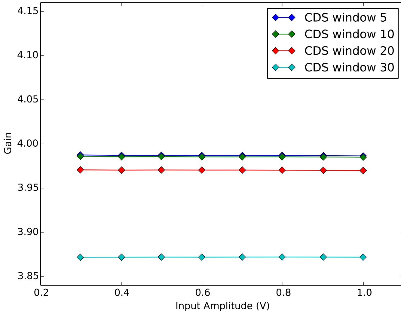
Average Amplifier Gain vs Amplifier Input Amplitude Quadrant 4, Channel 14
