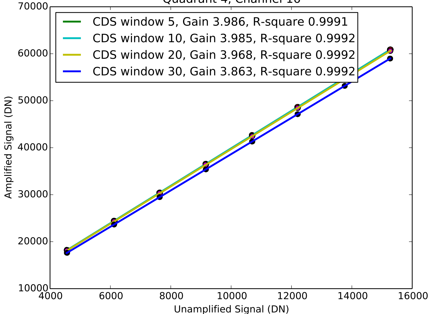
Signal vs Amplified Signal Quadrant 4, Channel 16
