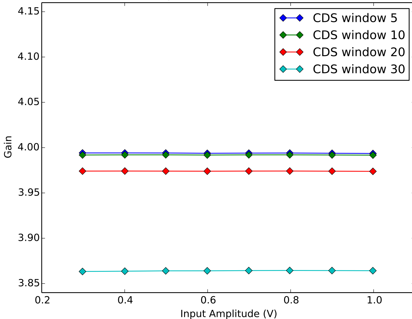
Average Amplifier Gain vs Amplifier Input Amplitude Quadrant 4, Channel 9
