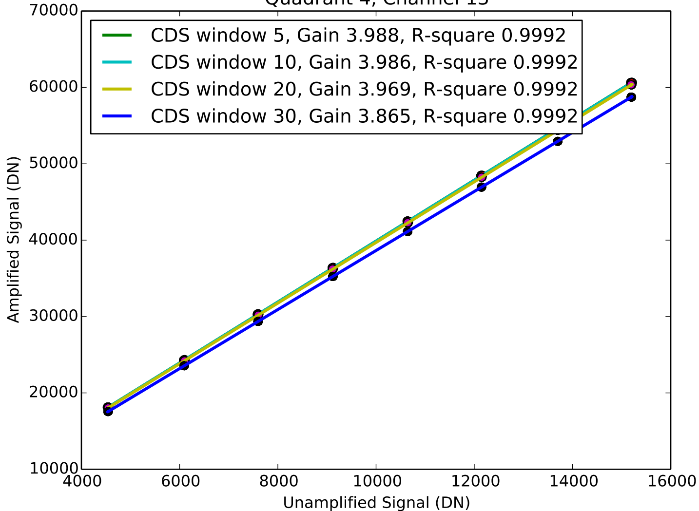
Signal vs Amplified Signal Quadrant 4, Channel 13
