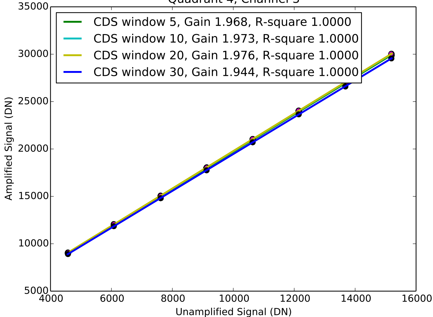
Signal vs Amplified Signal Quadrant 4, Channel 3
