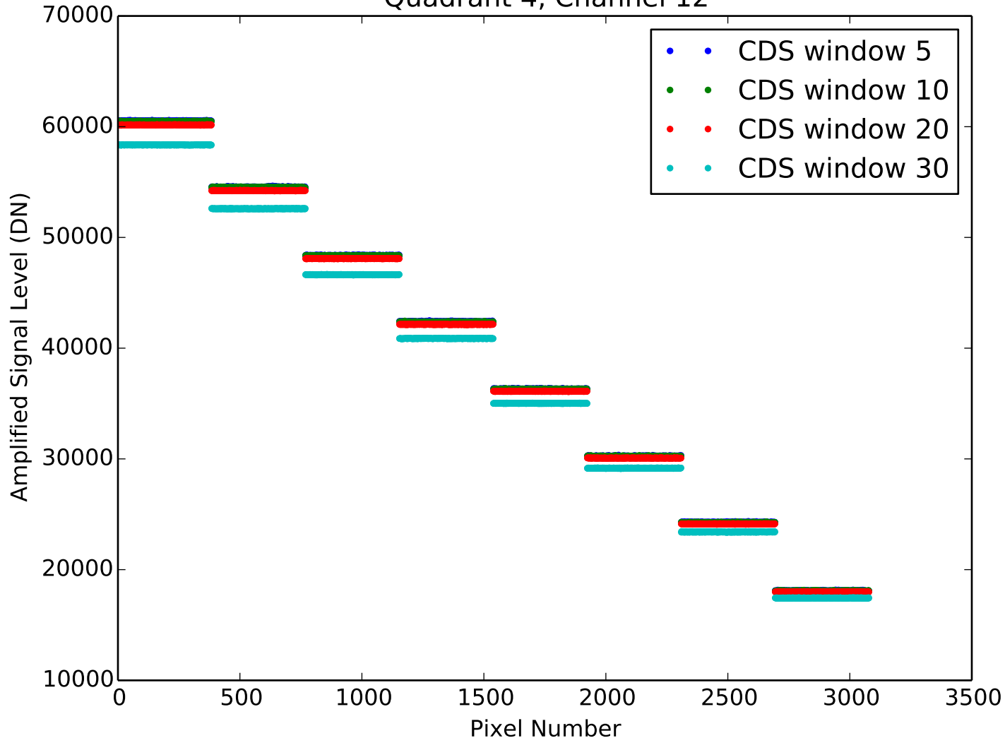
Amplified Signal Level from CDS Quadrant 4, Channel 12
