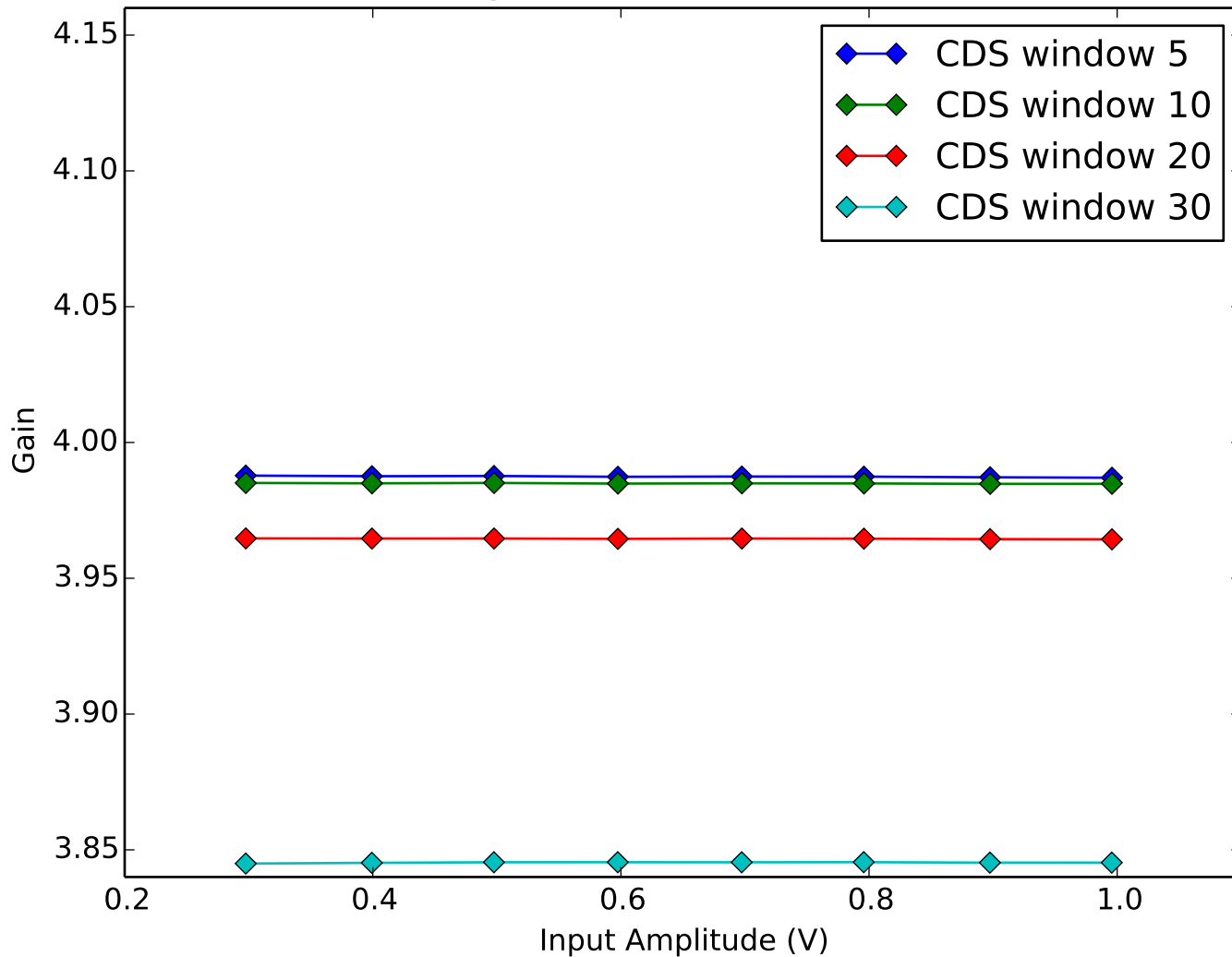
Average Amplifier Gain vs Amplifier Input Amplitude Quadrant 4, Channel 12
