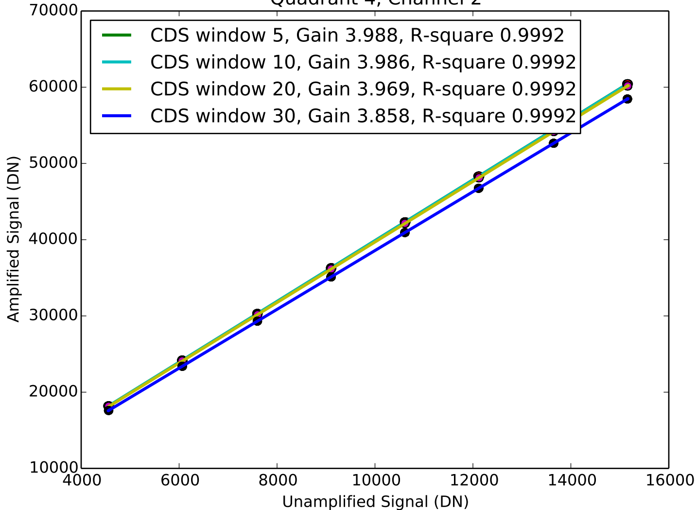
Signal vs Amplified Signal Quadrant 4, Channel 2
