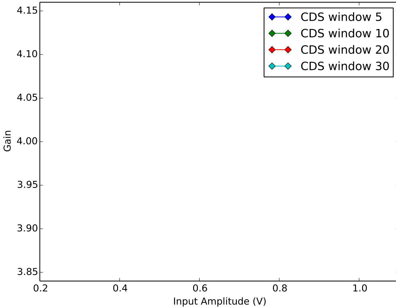
Average Amplifier Gain vs Amplifier Input Amplitude Quadrant 4, Channel 3
