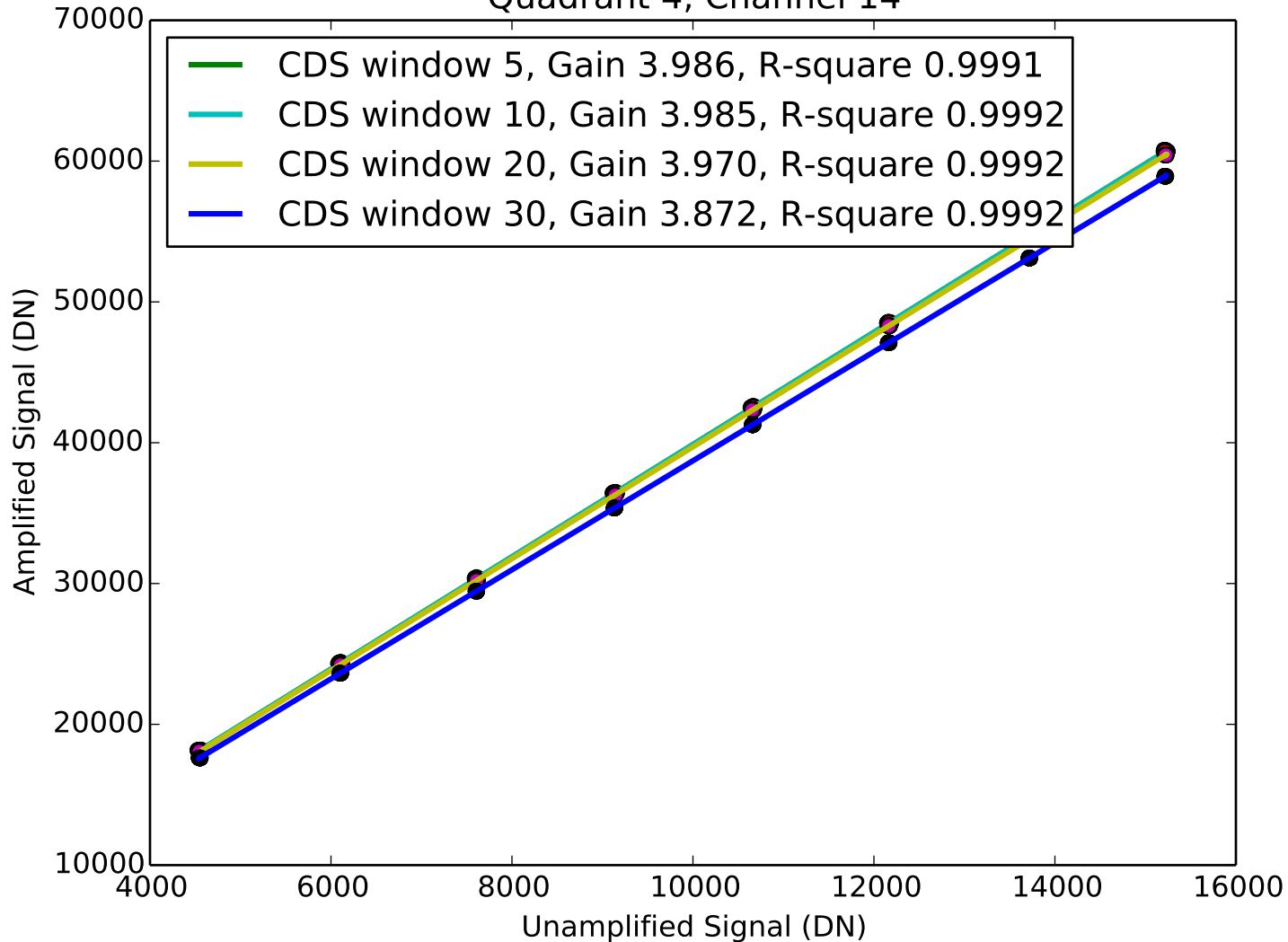
Signal vs Amplified Signal Quadrant 4, Channel 14
