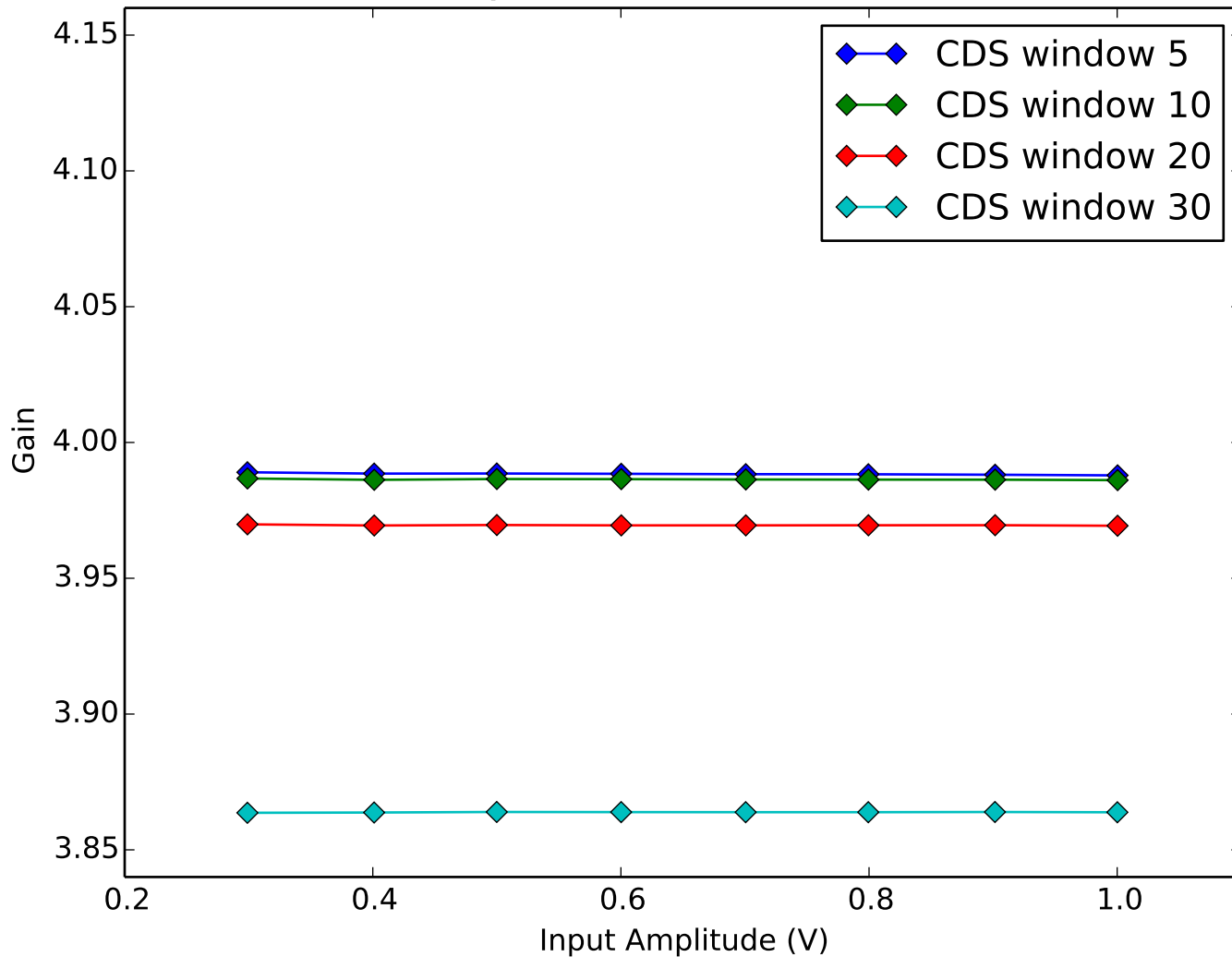
Average Amplifier Gain vs Amplifier Input Amplitude Quadrant 4, Channel 15
