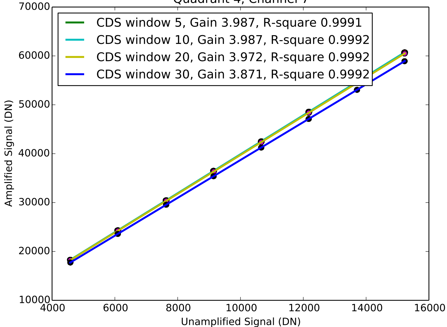
Signal vs Amplified Signal Quadrant 4, Channel 7
