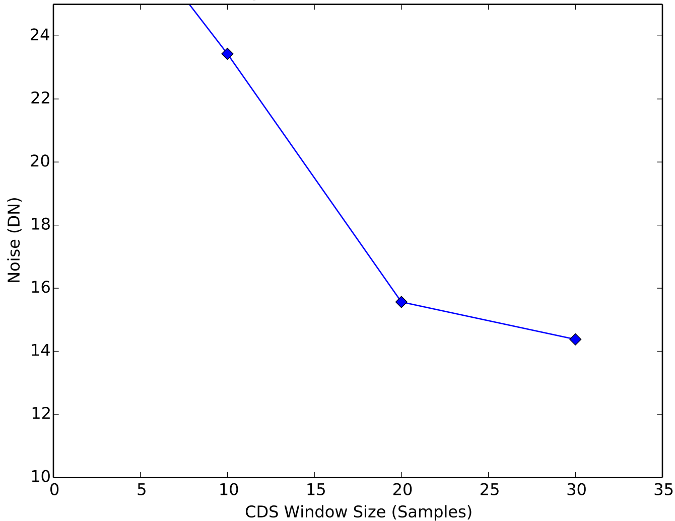
Amplifier Noise vs CDS Window Quadrant 4, Channel 16
