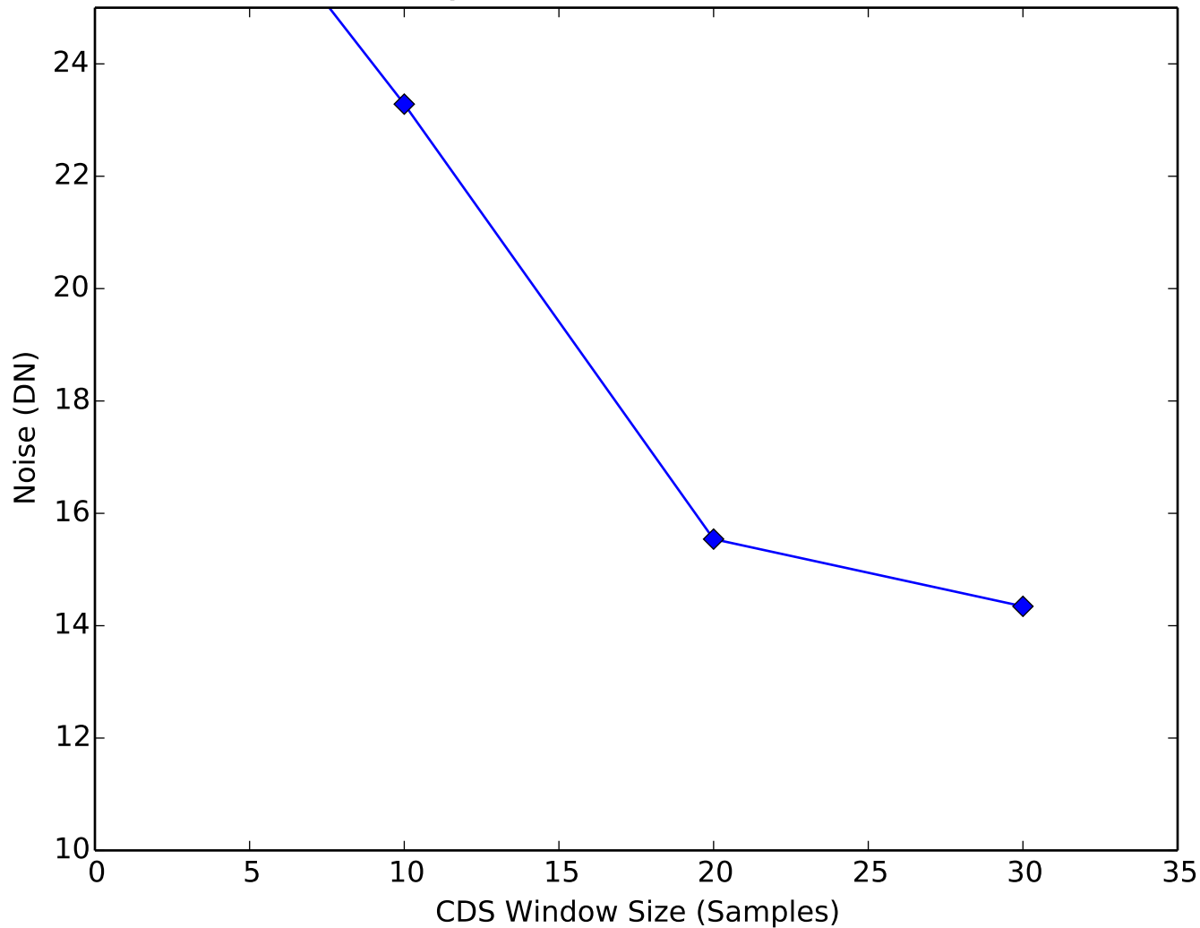
Amplifier Noise vs CDS Window Quadrant 4, Channel 15
