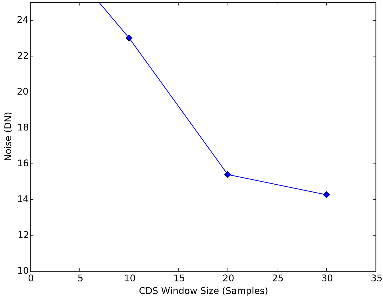
Amplifier Noise vs CDS Window Quadrant 4, Channel 12
