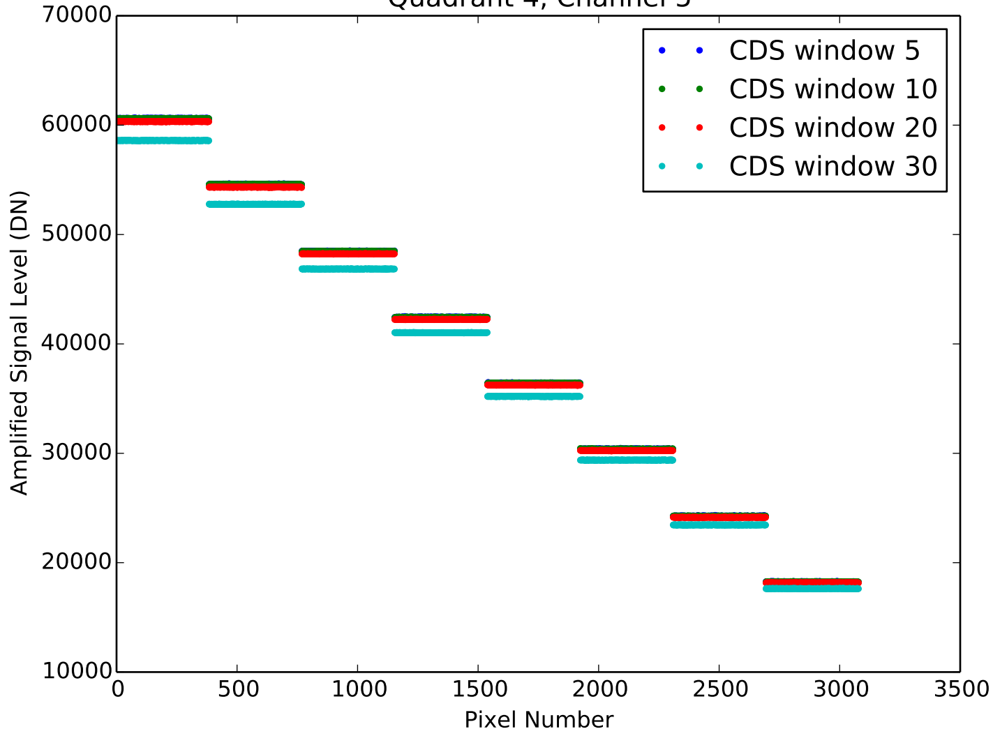
Amplified Signal Level from CDS Quadrant 4, Channel 5
