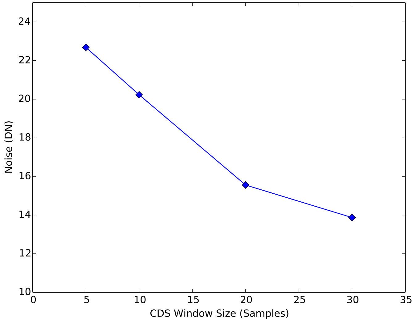
Amplifier Noise vs CDS Window Quadrant 4, Channel 6
