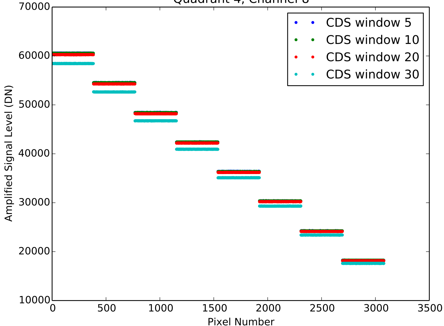
Amplified Signal Level from CDS Quadrant 4, Channel 8
