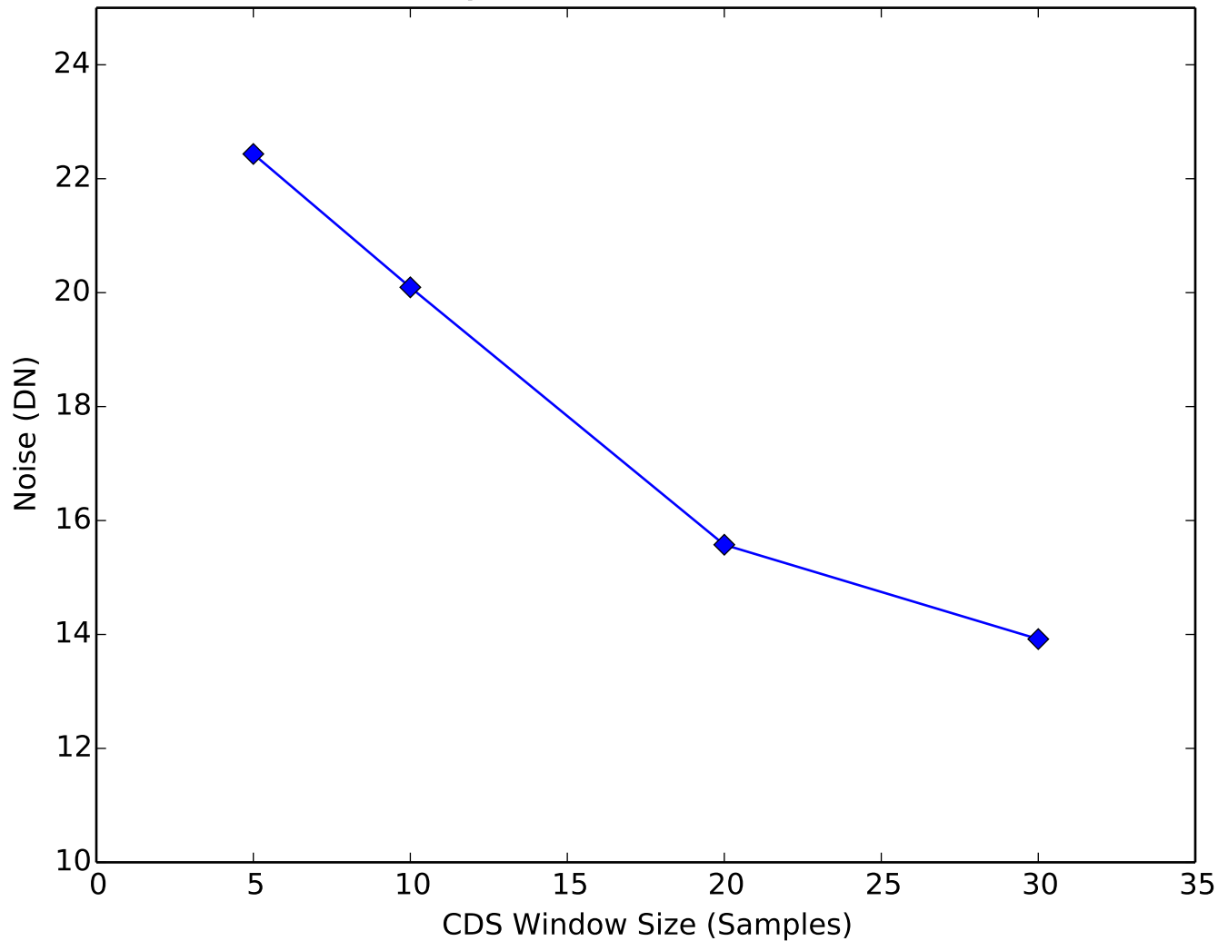
Amplifier Noise vs CDS Window Quadrant 4, Channel 7
