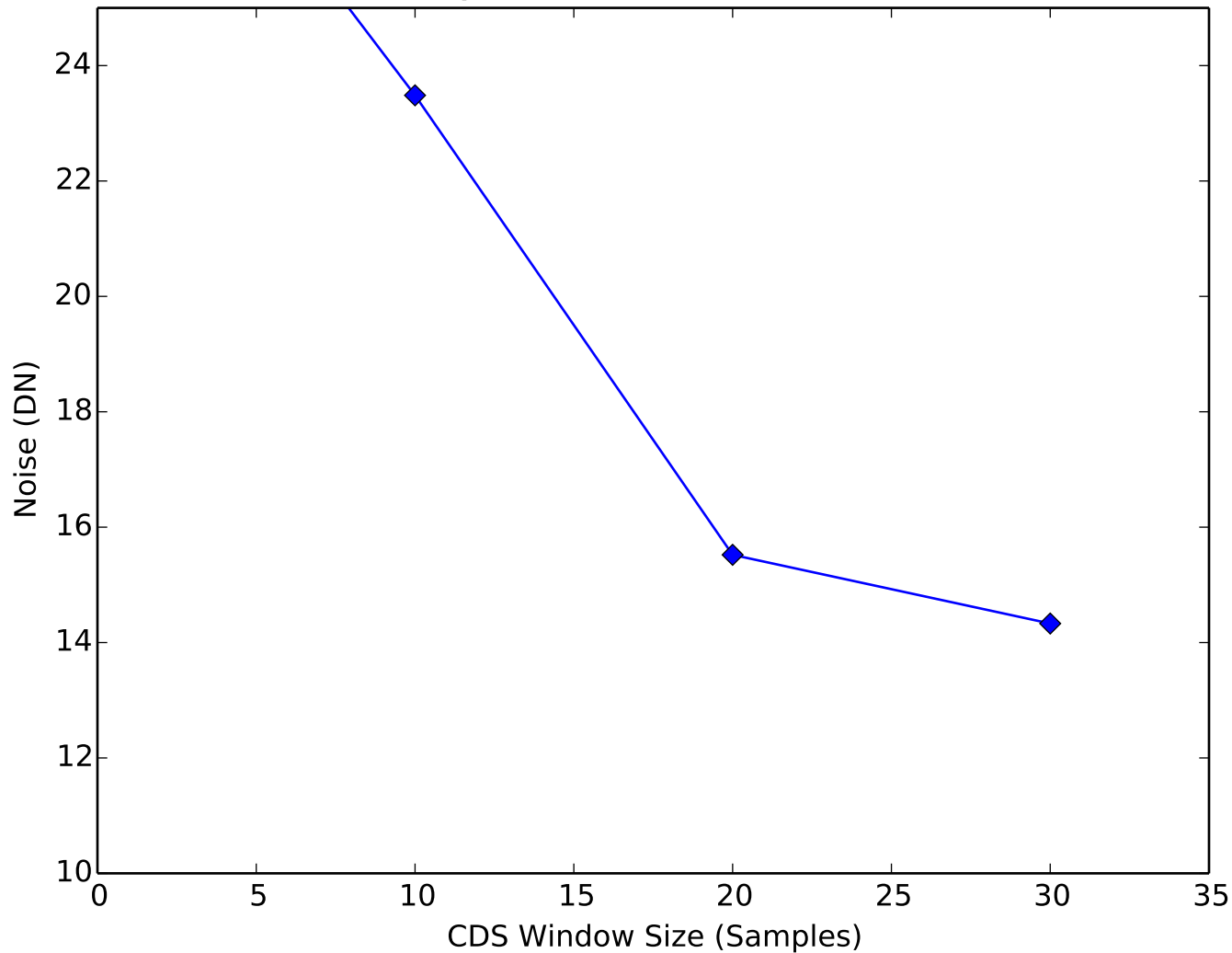
Amplifier Noise vs CDS Window Quadrant 4, Channel 13
