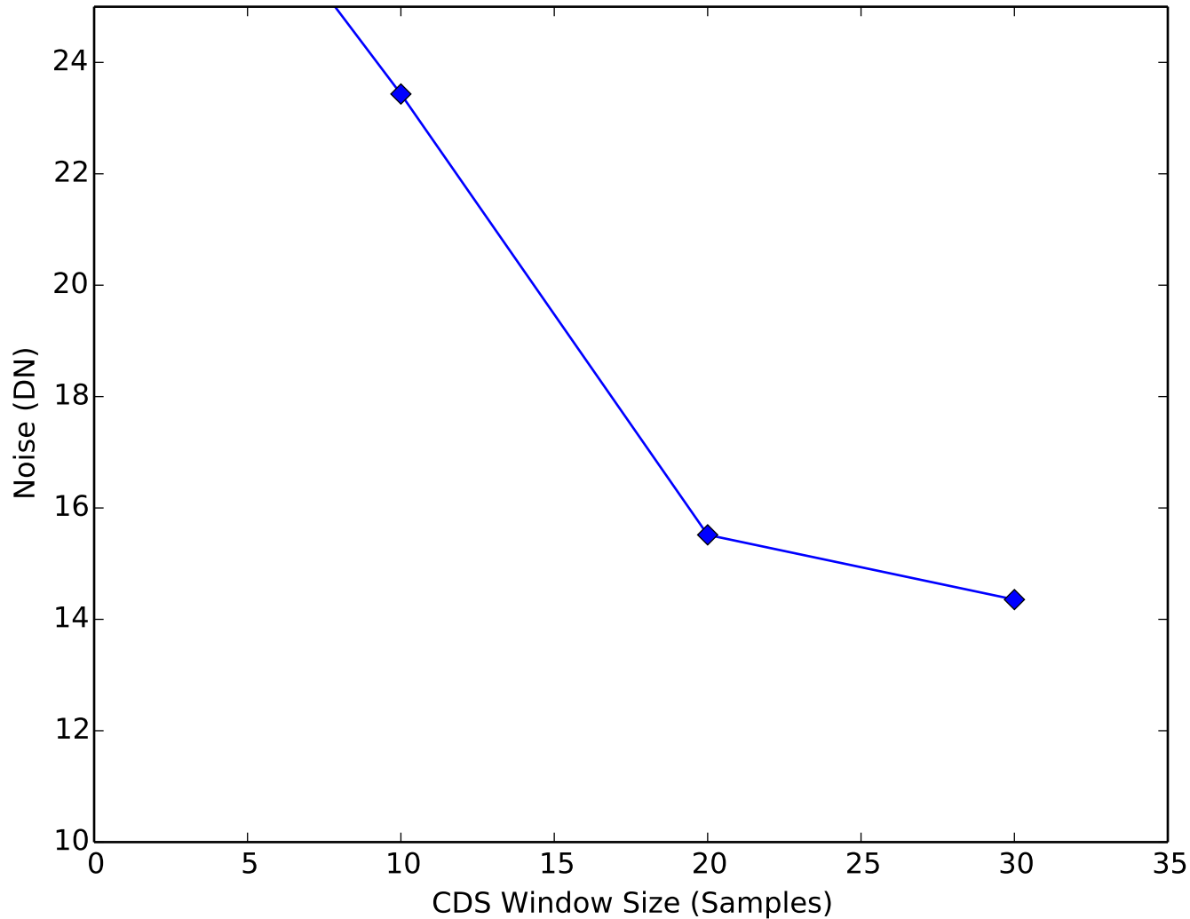
Amplifier Noise vs CDS Window Quadrant 4, Channel 9
