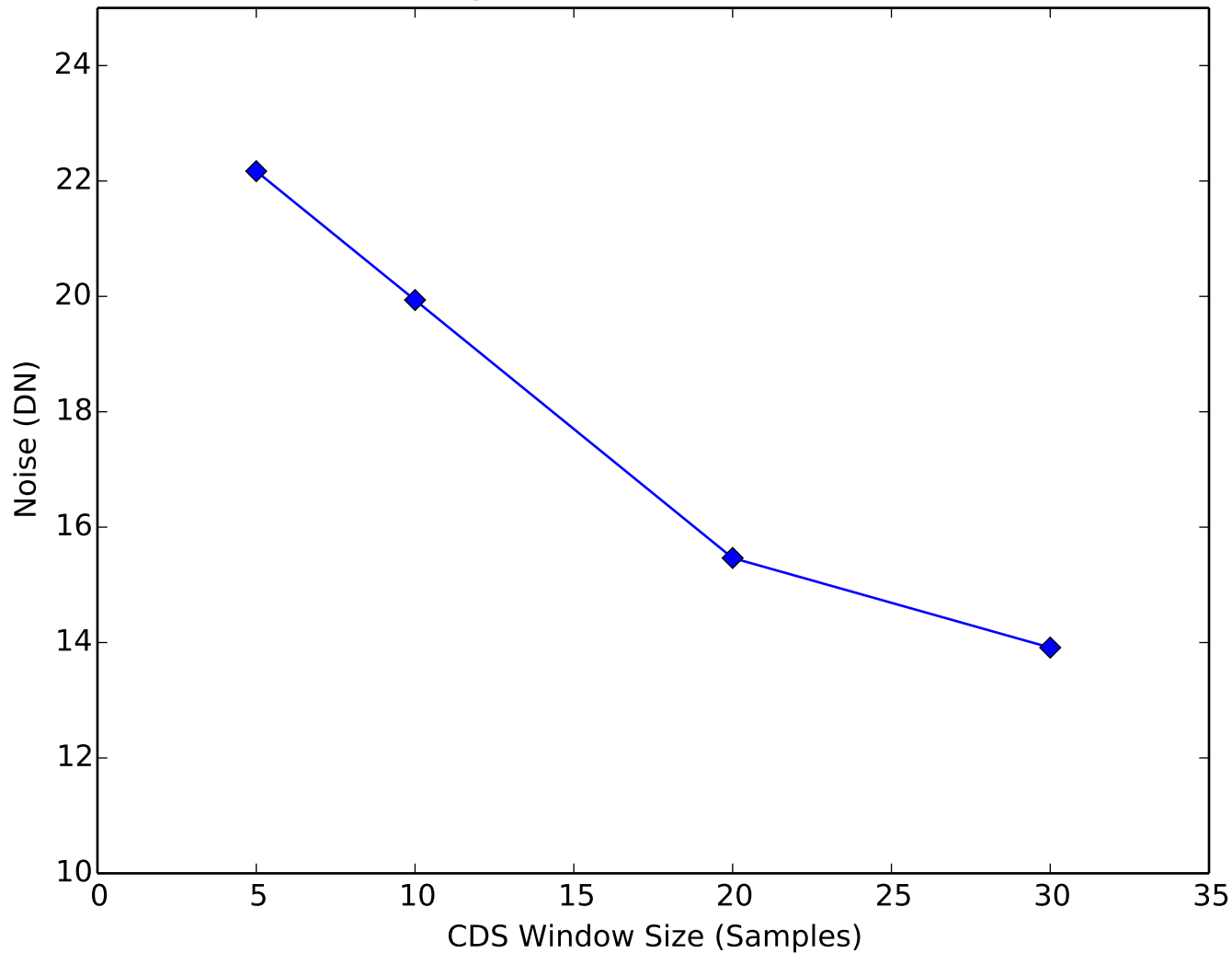
Amplifier Noise vs CDS Window Quadrant 4, Channel 5
