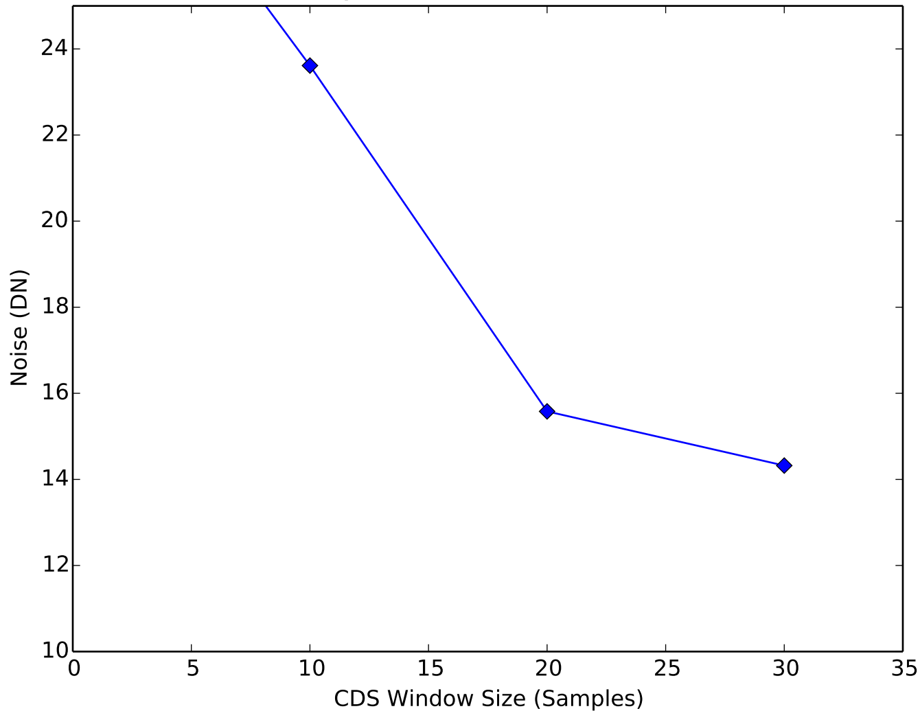
Amplifier Noise vs CDS Window Quadrant 4, Channel 14
