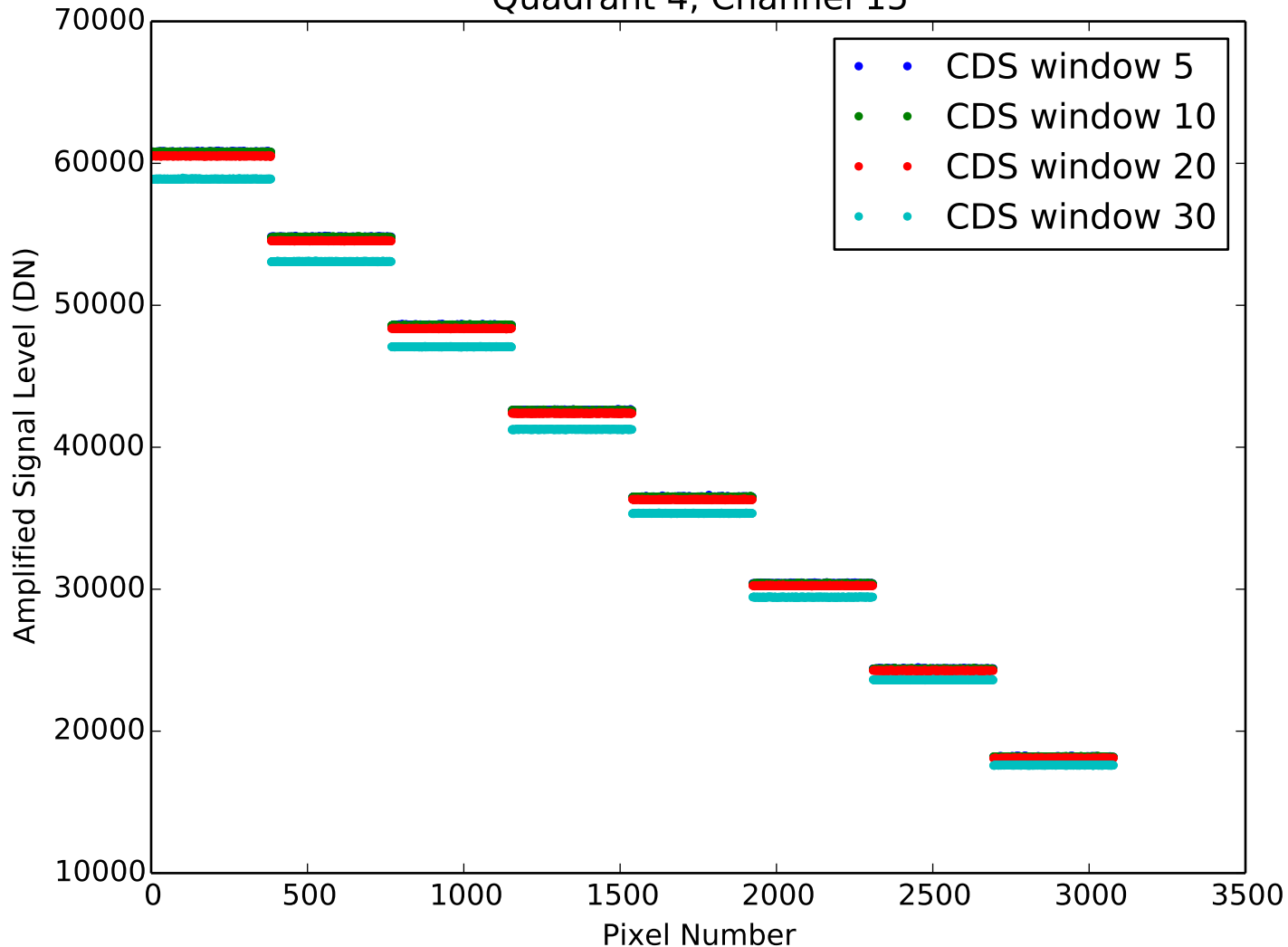
Amplified Signal Level from CDS Quadrant 4, Channel 15
