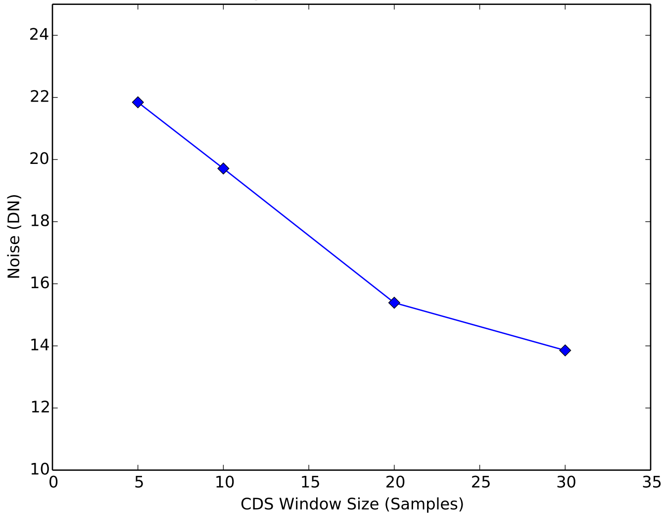
Amplifier Noise vs CDS Window Quadrant 4, Channel 2
