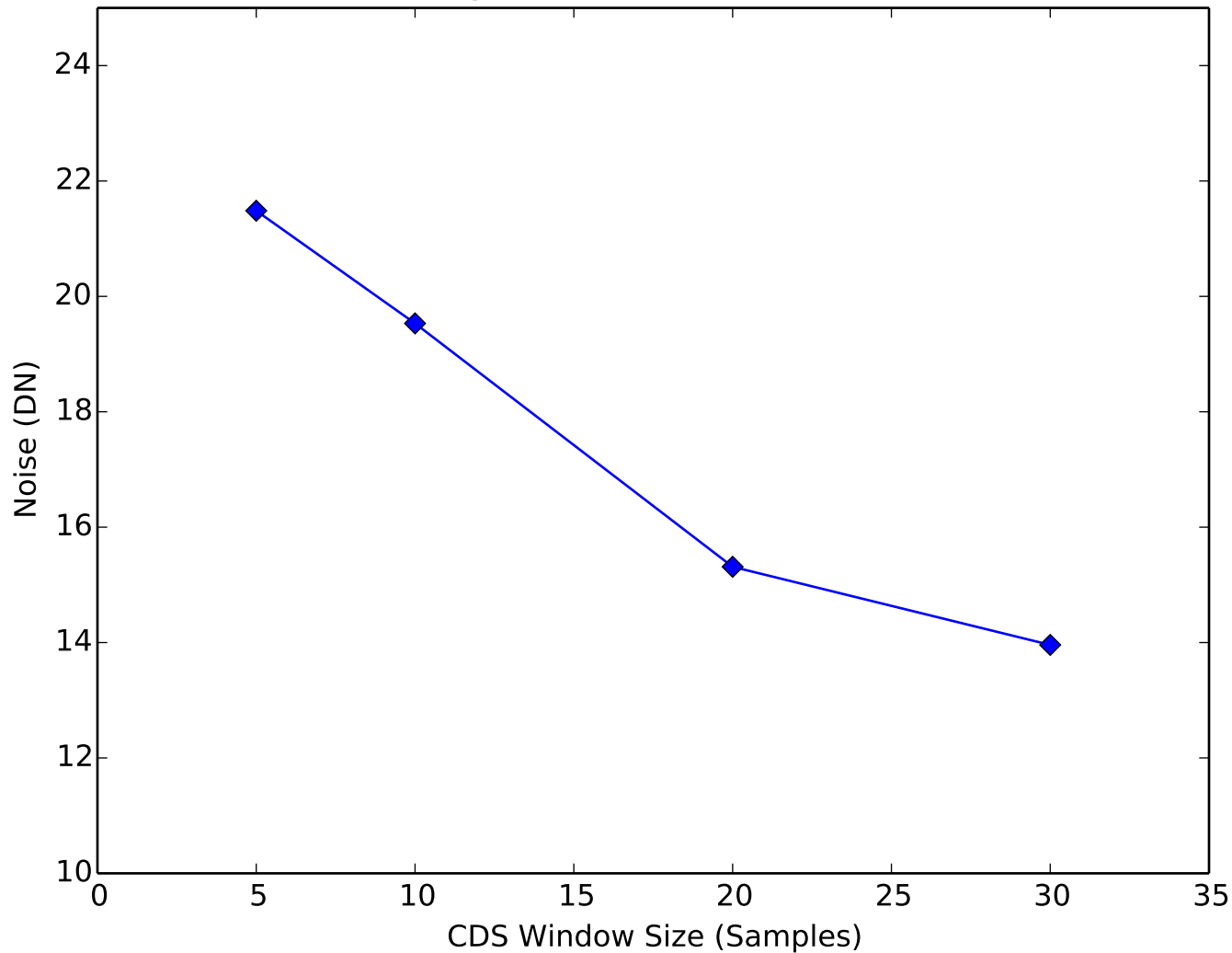
Amplifier Noise vs CDS Window Quadrant 4, Channel 4
