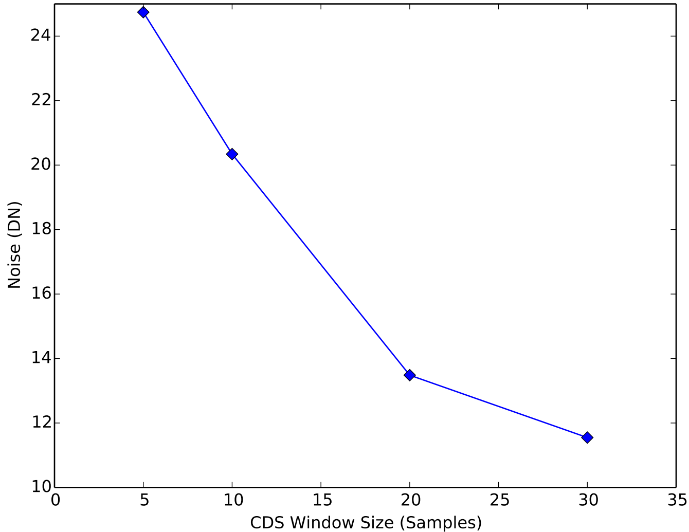
Amplifier Noise vs CDS Window Quadrant 4, Channel 3
