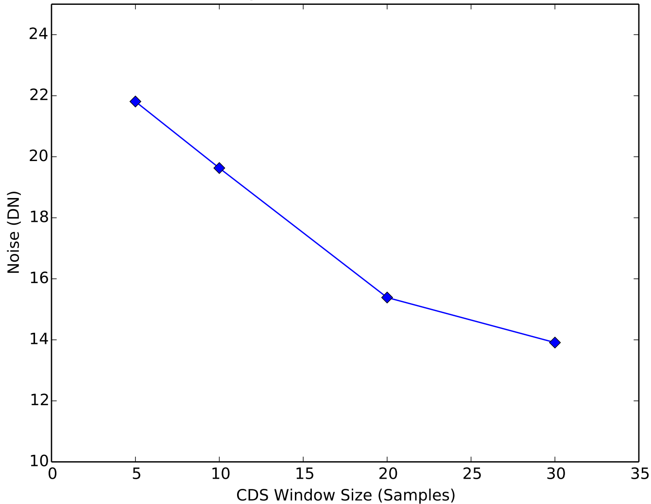
Amplifier Noise vs CDS Window Quadrant 4, Channel 1
