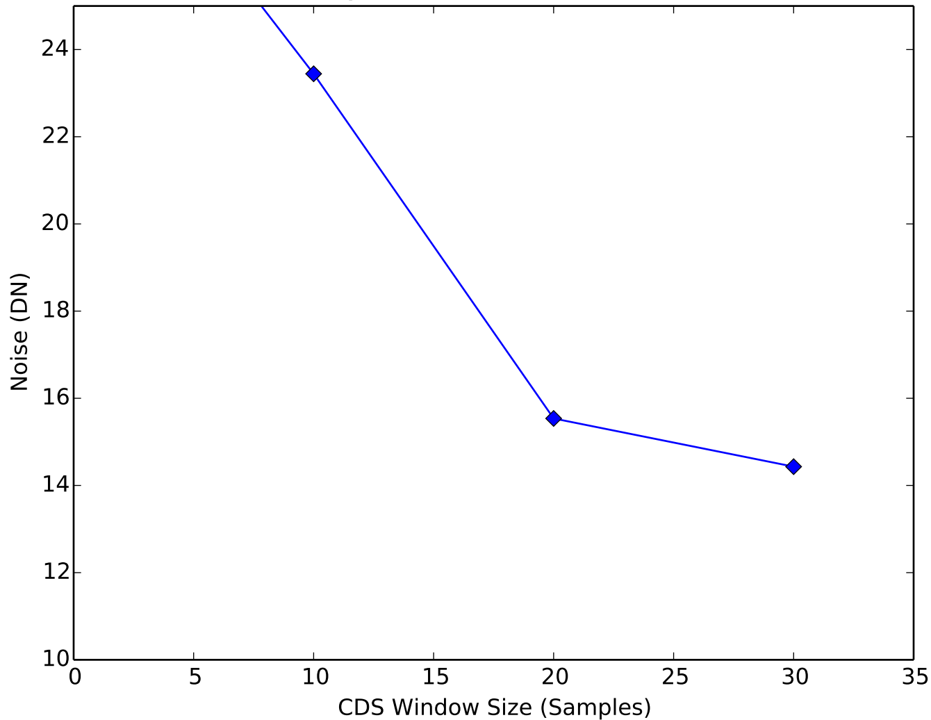
Amplifier Noise vs CDS Window Quadrant 4, Channel 10
