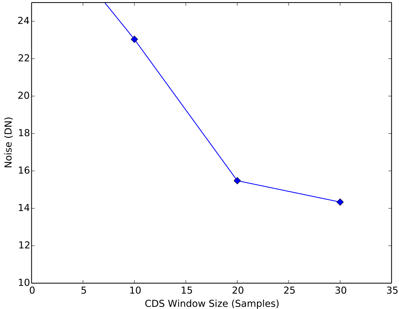
Amplifier Noise vs CDS Window Quadrant 4, Channel 11
