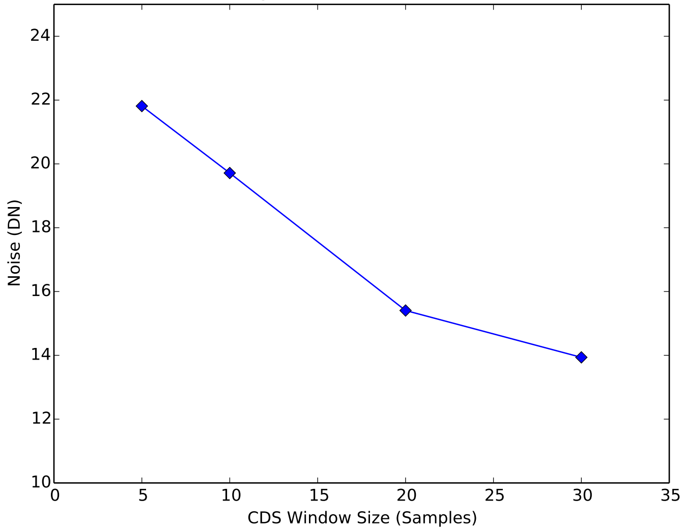
Amplifier Noise vs CDS Window Quadrant 4, Channel 8
