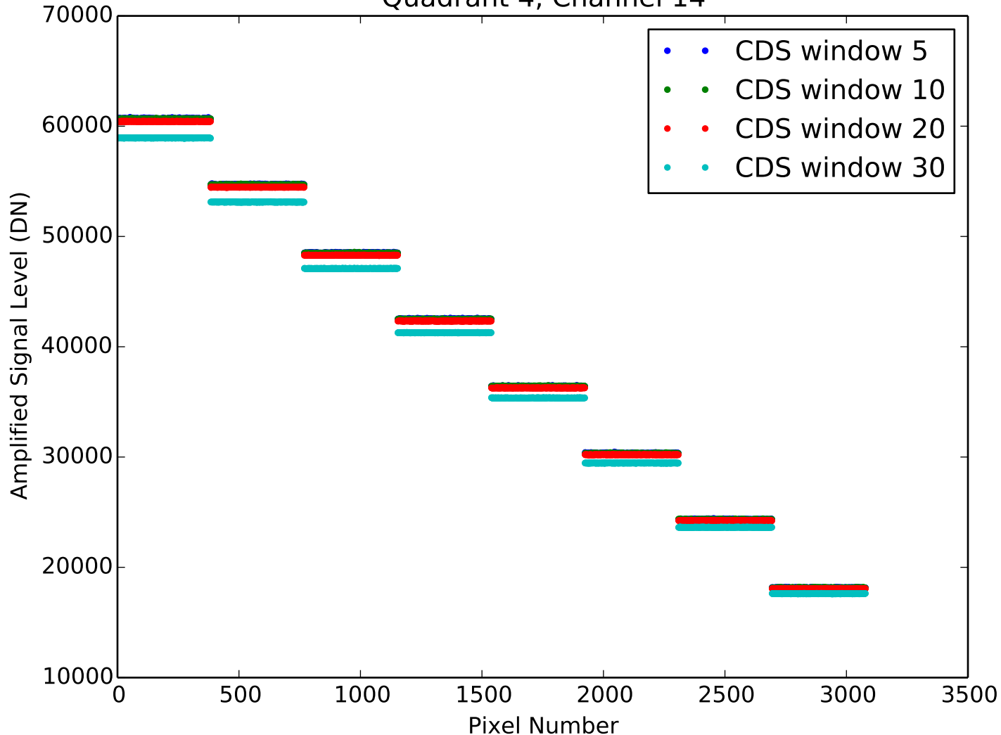
Amplified Signal Level from CDS Quadrant 4, Channel 14
