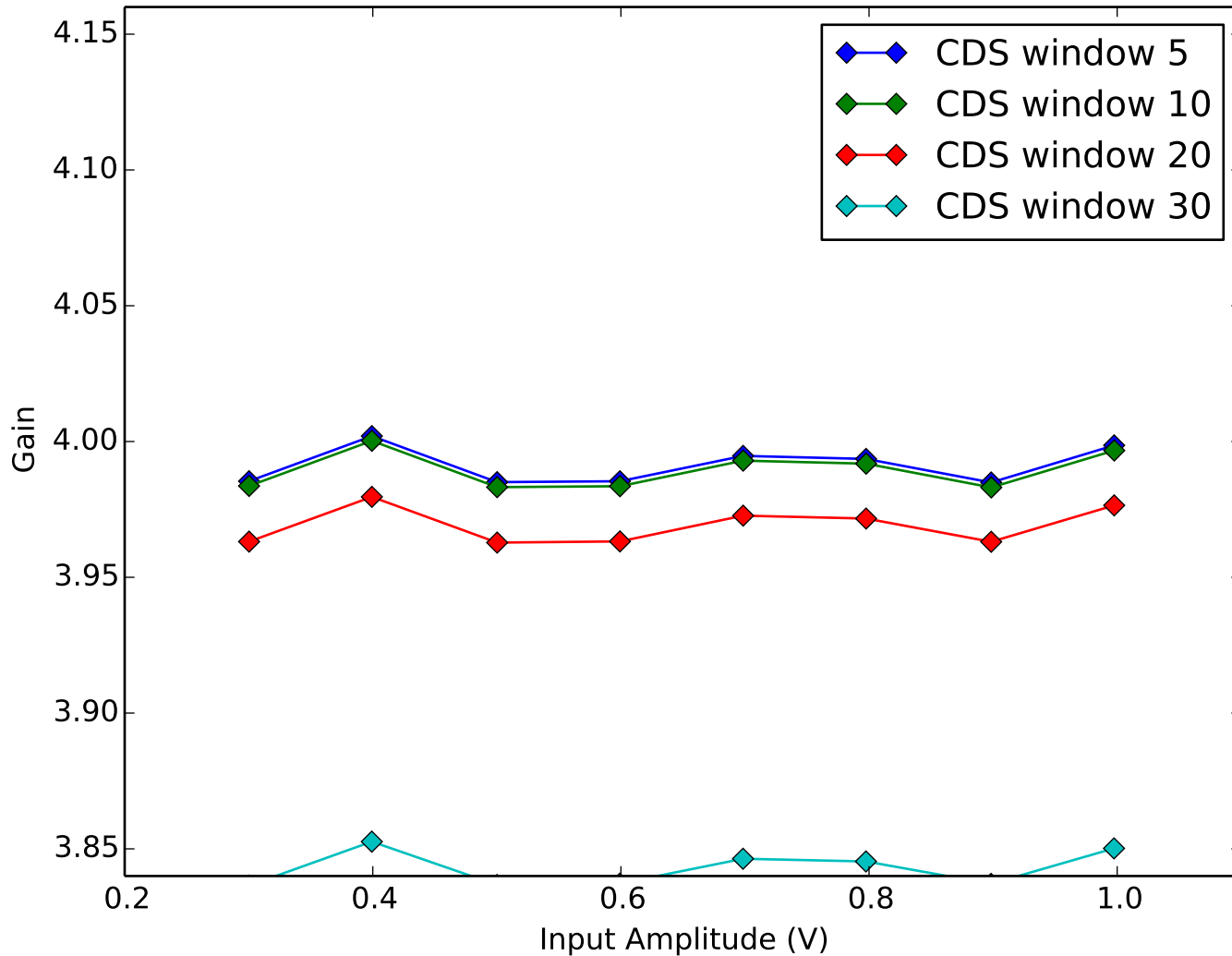
Average Amplifier Gain vs Amplifier Input Amplitude Quadrant 3, Channel 5
