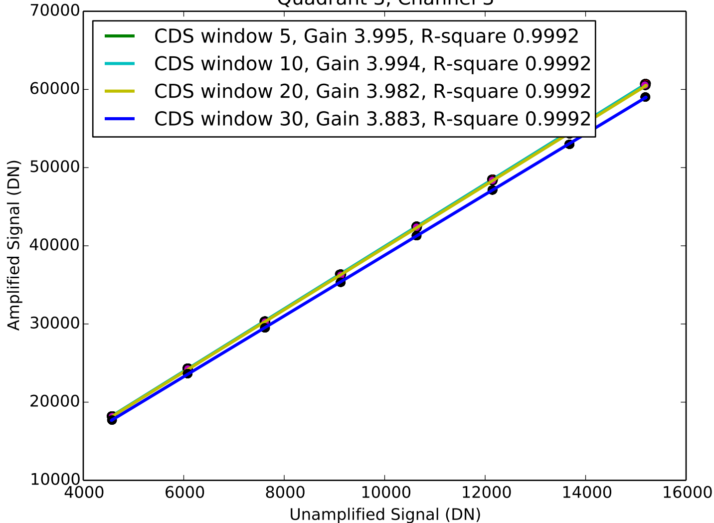
Signal vs Amplified Signal Quadrant 3, Channel 3
