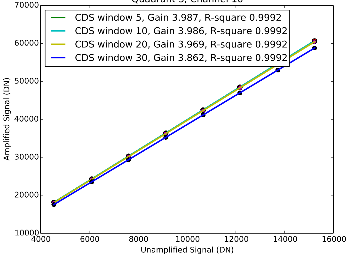
Signal vs Amplified Signal Quadrant 3, Channel 10
