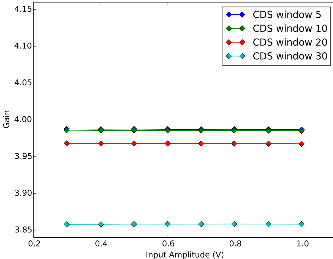
Average Amplifier Gain vs Amplifier Input Amplitude Quadrant 3, Channel 14
