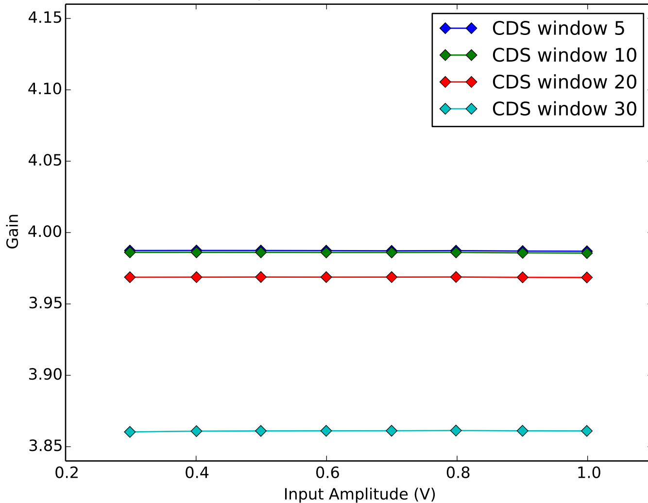
Average Amplifier Gain vs Amplifier Input Amplitude Quadrant 3, Channel 10
