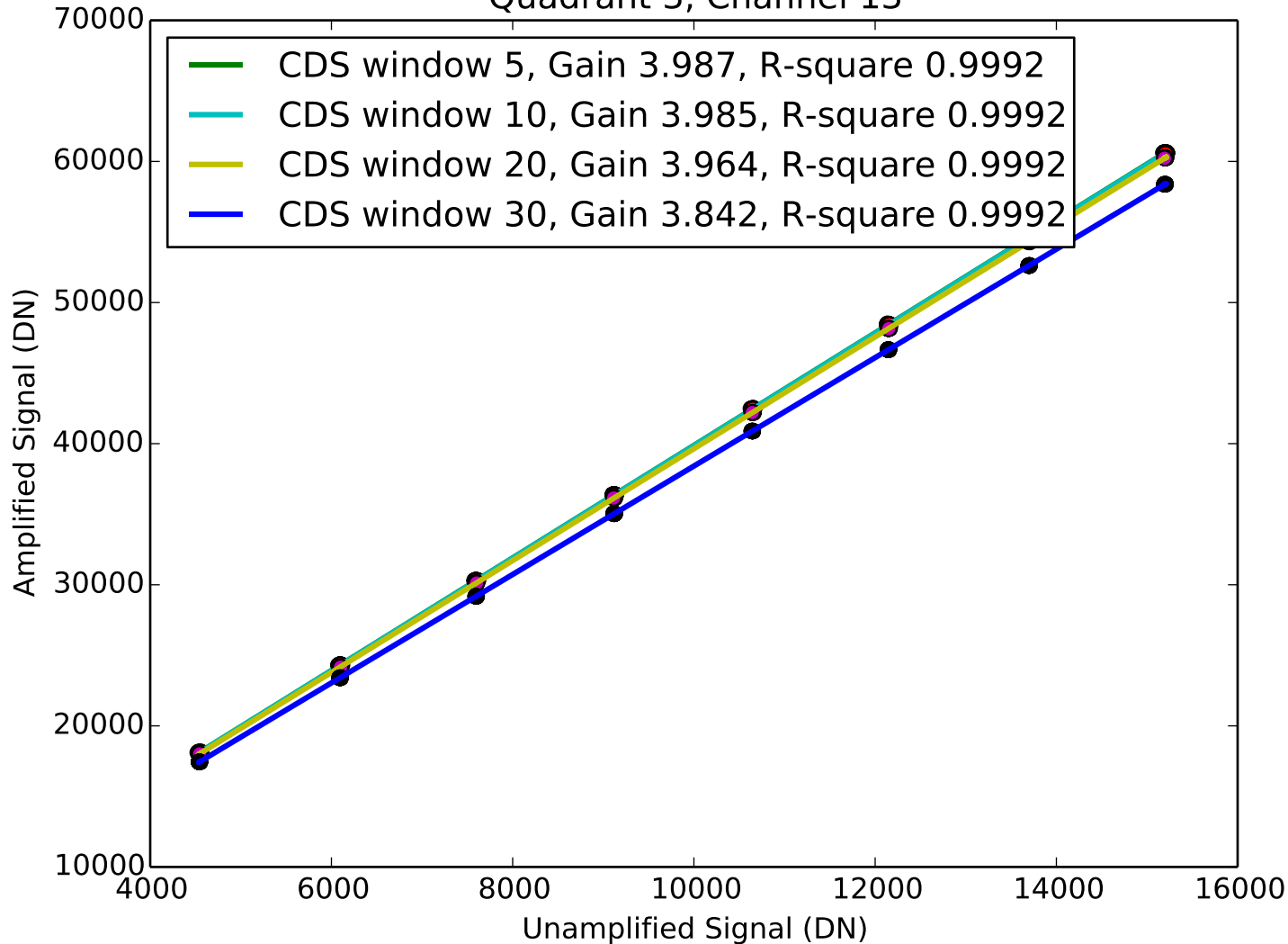
Signal vs Amplified Signal Quadrant 3, Channel 13
