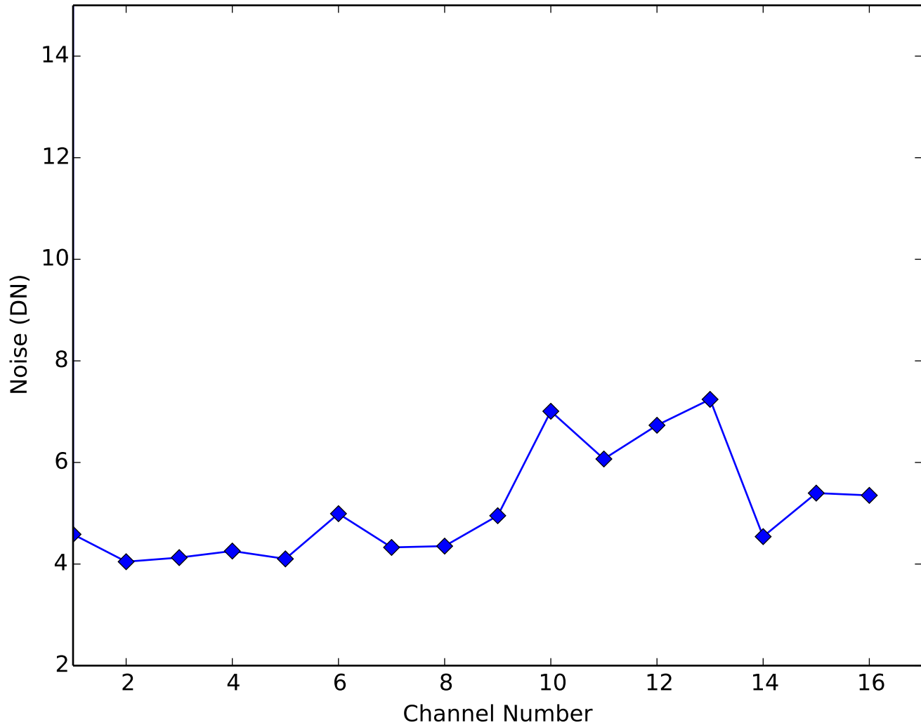
Shorted Input Noise for VIB Amplifiers Quadrant3
