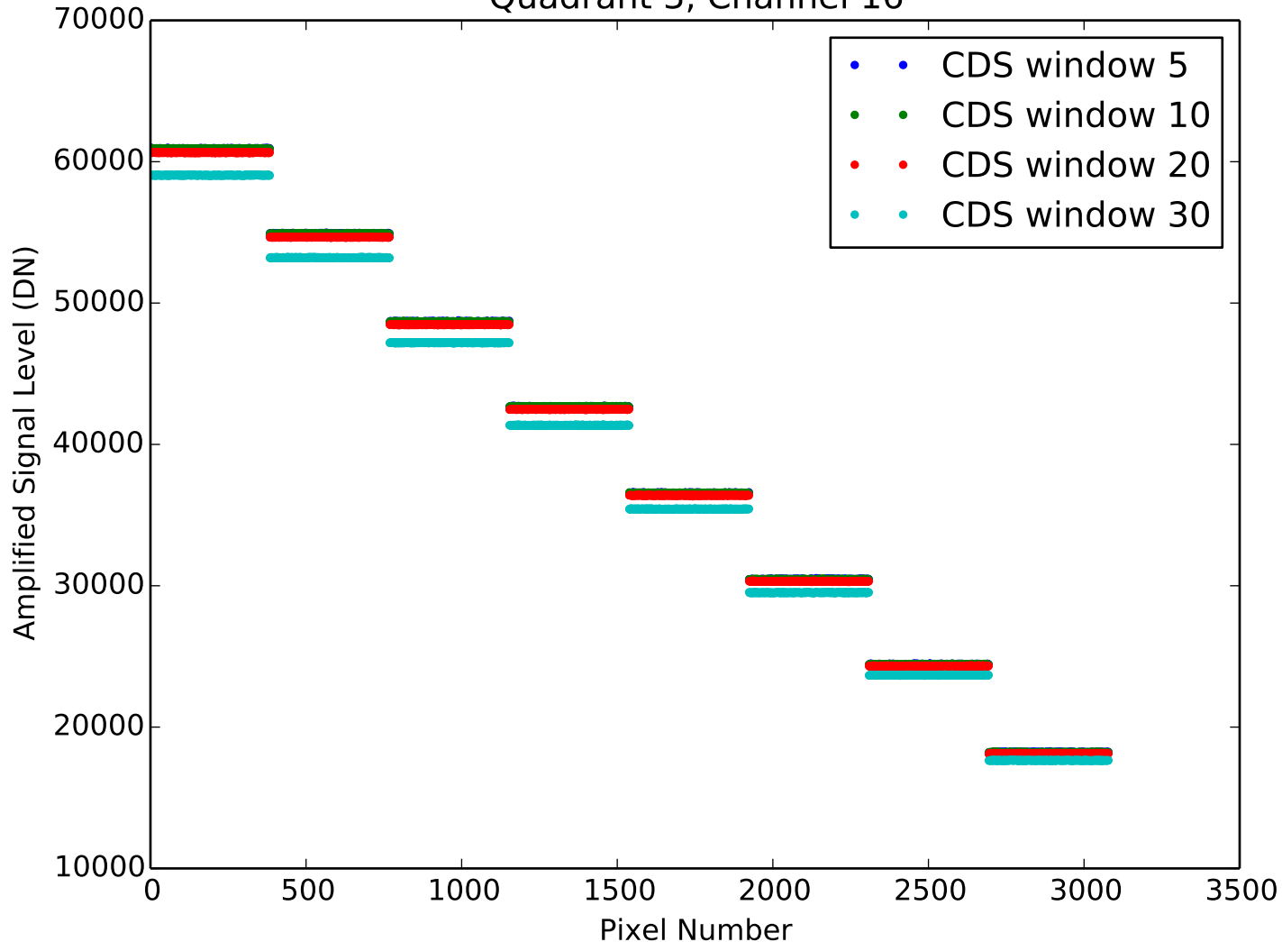
Amplified Signal Level from CDS Quadrant 3, Channel 16
