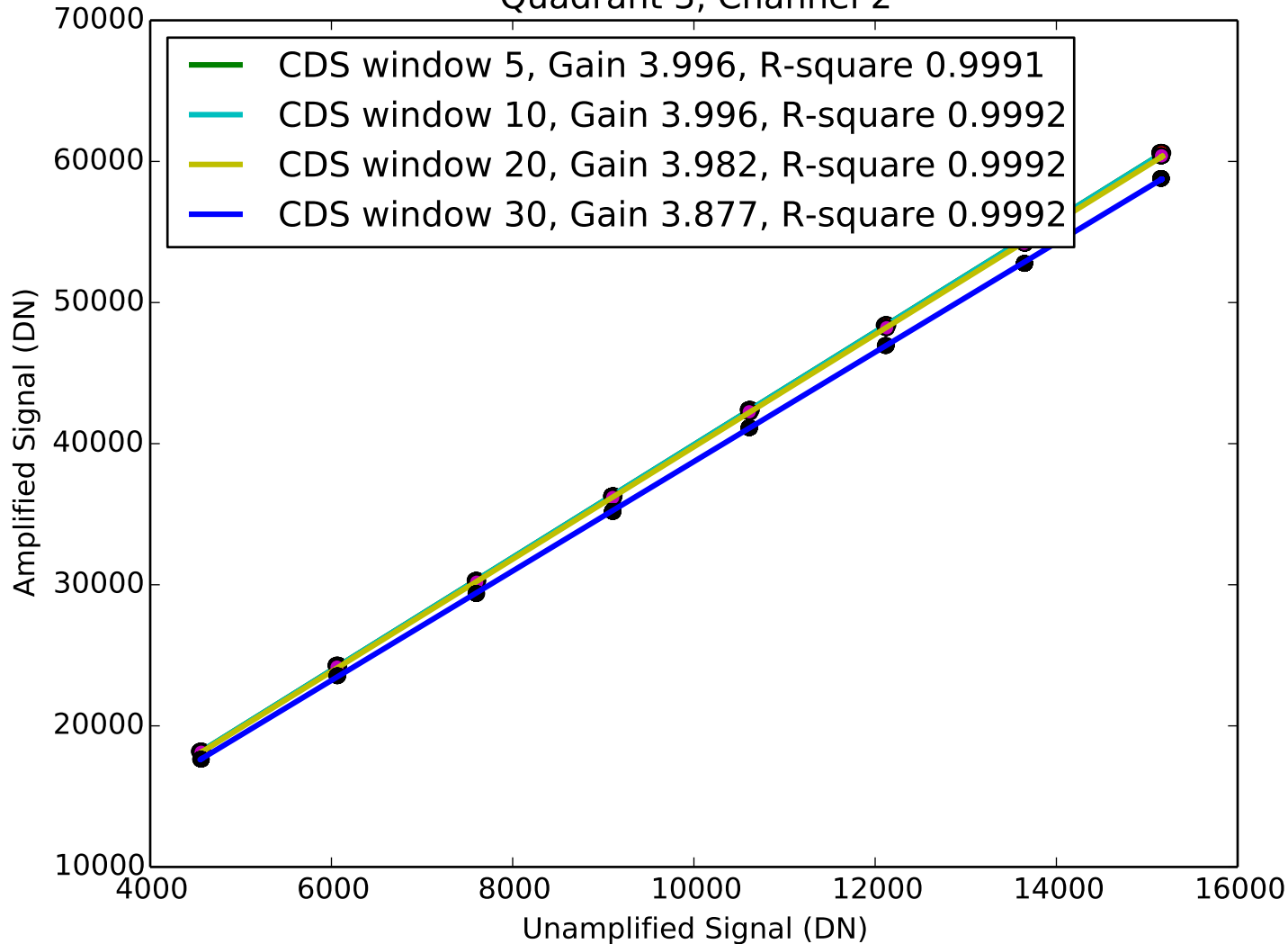
Signal vs Amplified Signal Quadrant 3, Channel 2
