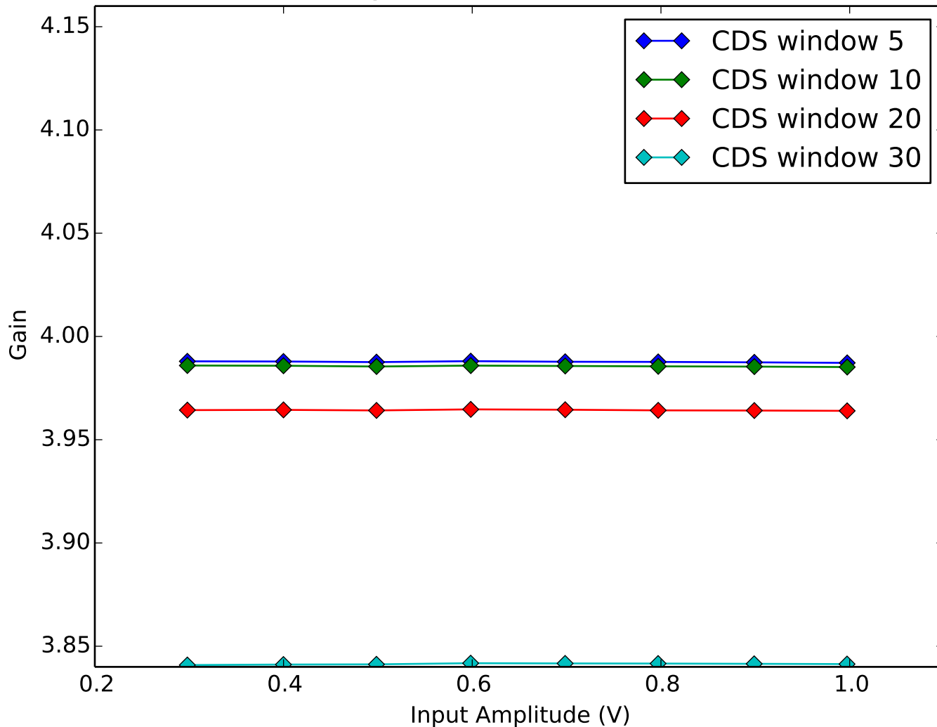
Average Amplifier Gain vs Amplifier Input Amplitude Quadrant 3, Channel 13
