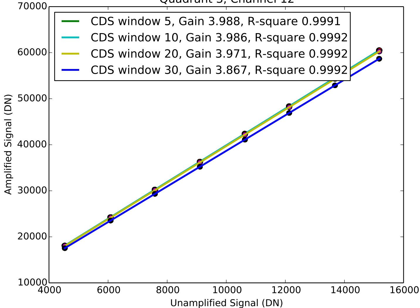
Signal vs Amplified Signal Quadrant 3, Channel 12
