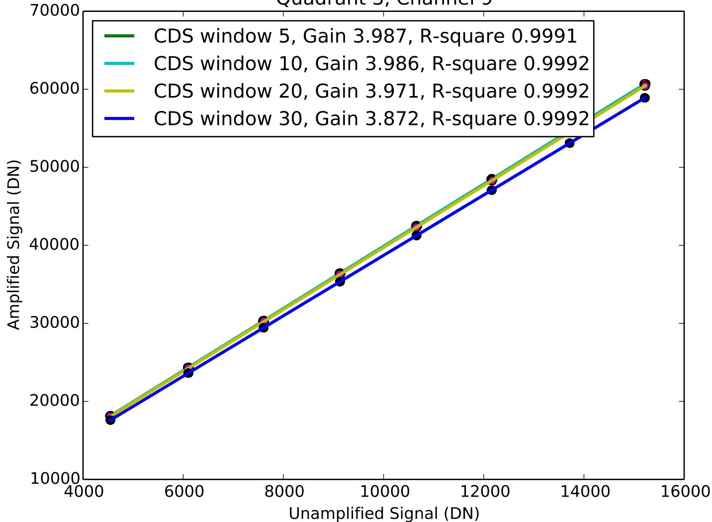
Signal vs Amplified Signal Quadrant 3, Channel 9
