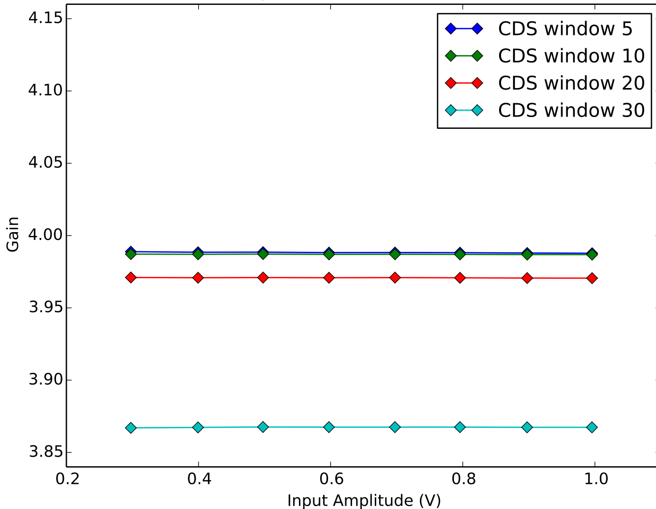
Average Amplifier Gain vs Amplifier Input Amplitude Quadrant 3, Channel 12
