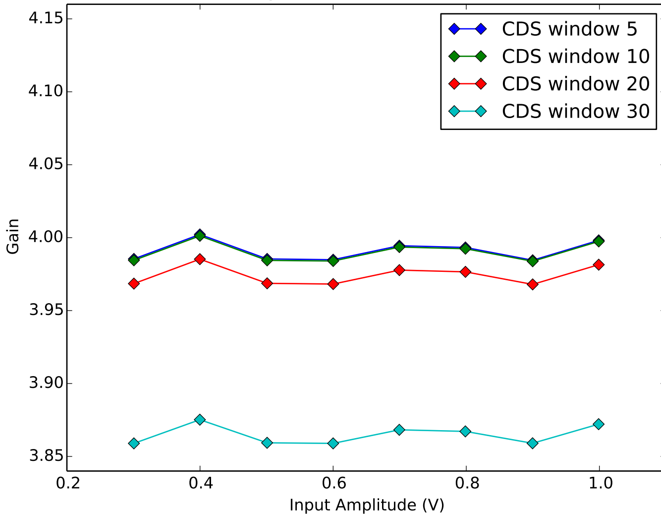
Average Amplifier Gain vs Amplifier Input Amplitude Quadrant 3, Channel 7
