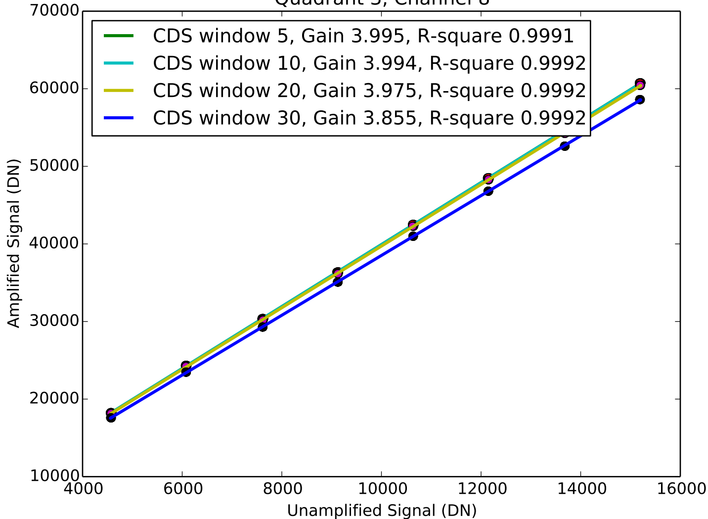
Signal vs Amplified Signal Quadrant 3, Channel 8
