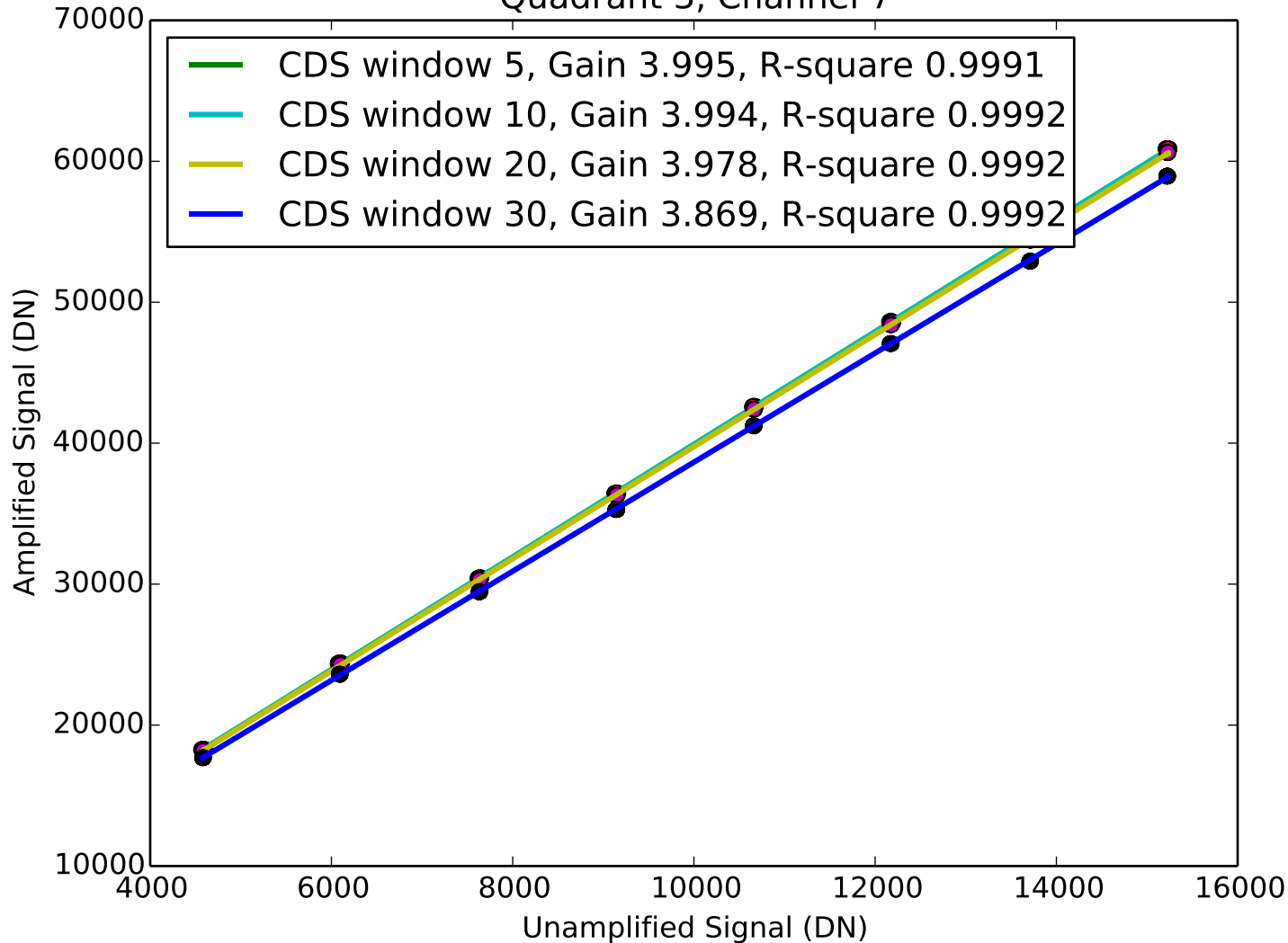
Signal vs Amplified Signal Quadrant 3, Channel 7
