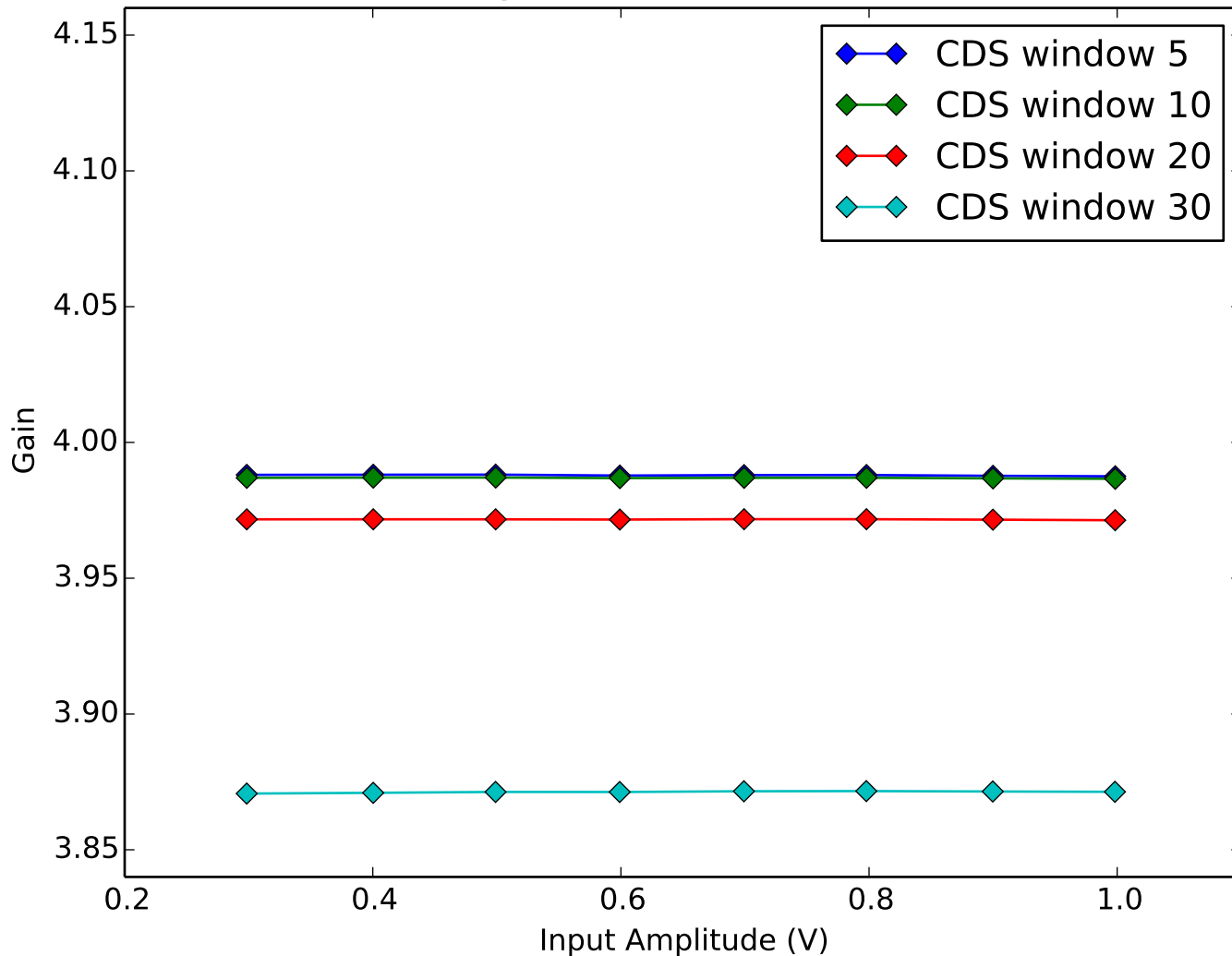
Average Amplifier Gain vs Amplifier Input Amplitude Quadrant 3, Channel 9
