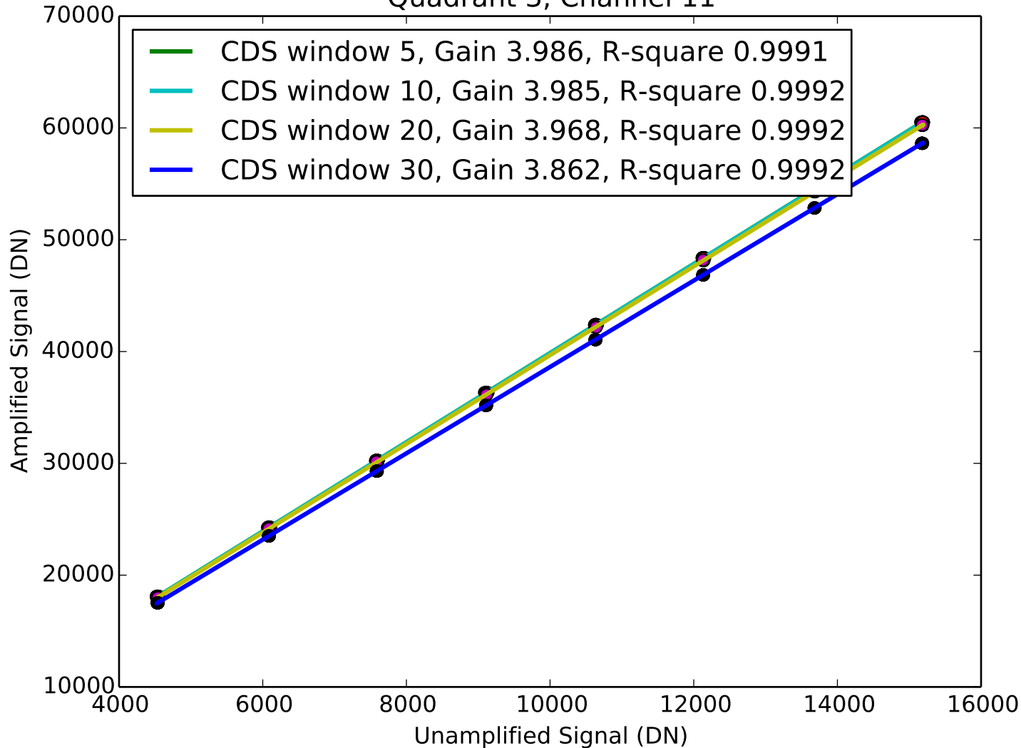
Signal vs Amplified Signal Quadrant 3, Channel 11
