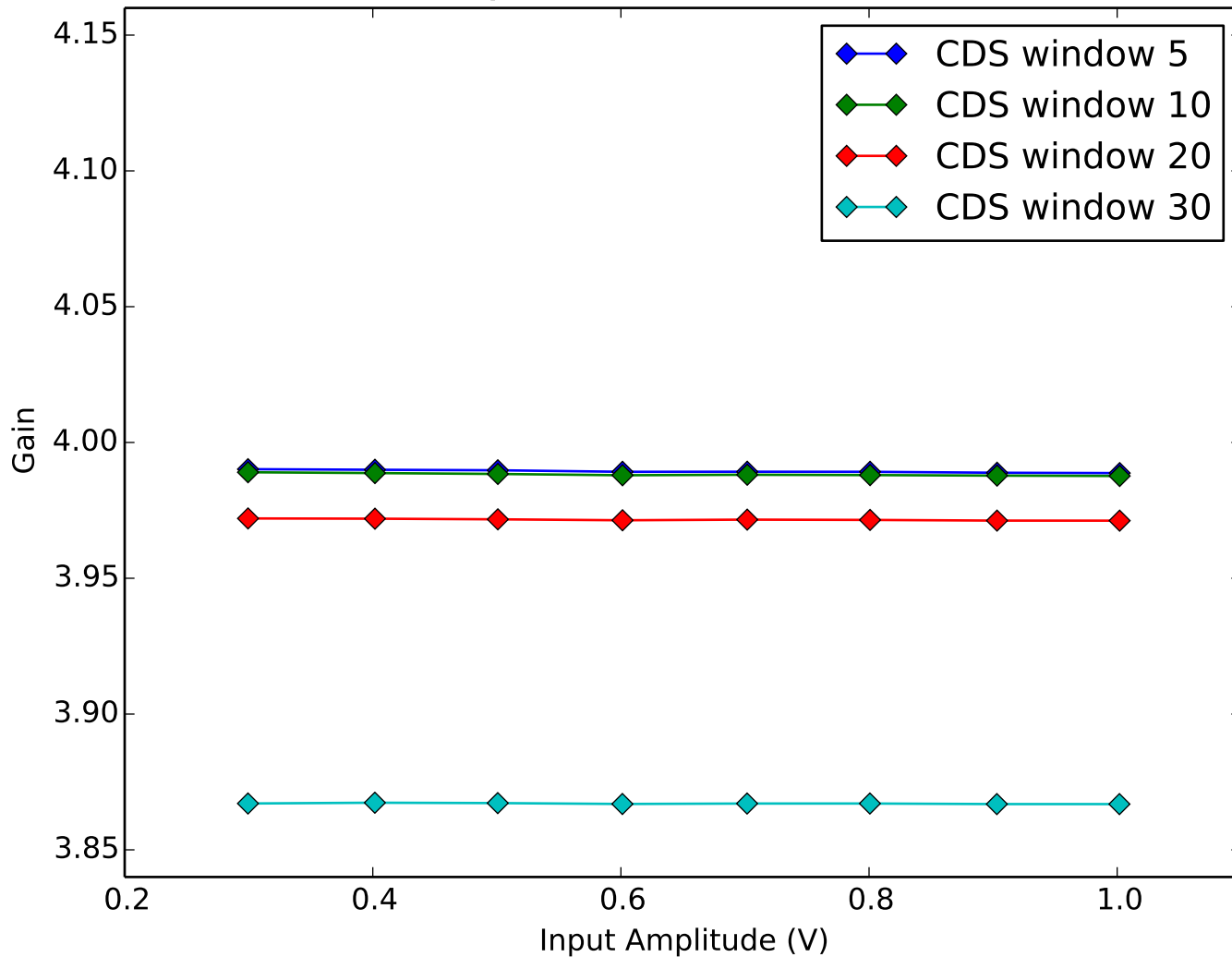
Average Amplifier Gain vs Amplifier Input Amplitude Quadrant 3, Channel 16
