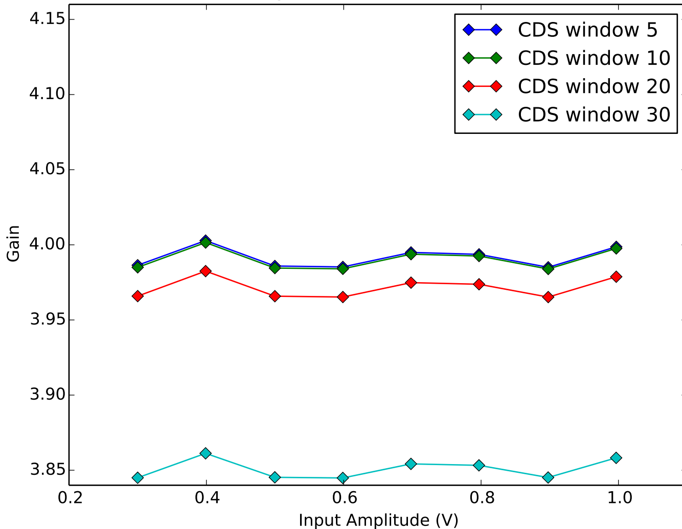
Average Amplifier Gain vs Amplifier Input Amplitude Quadrant 3, Channel 8
