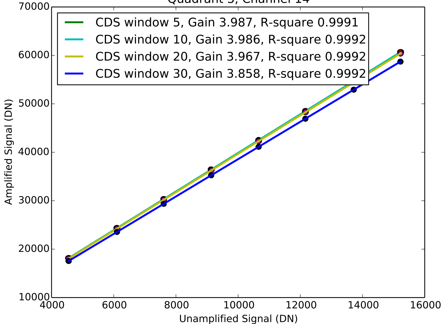
Signal vs Amplified Signal Quadrant 3, Channel 14
