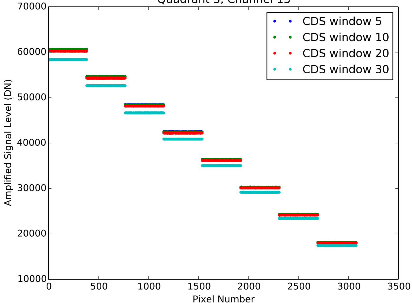
Amplified Signal Level from CDS Quadrant 3, Channel 13
