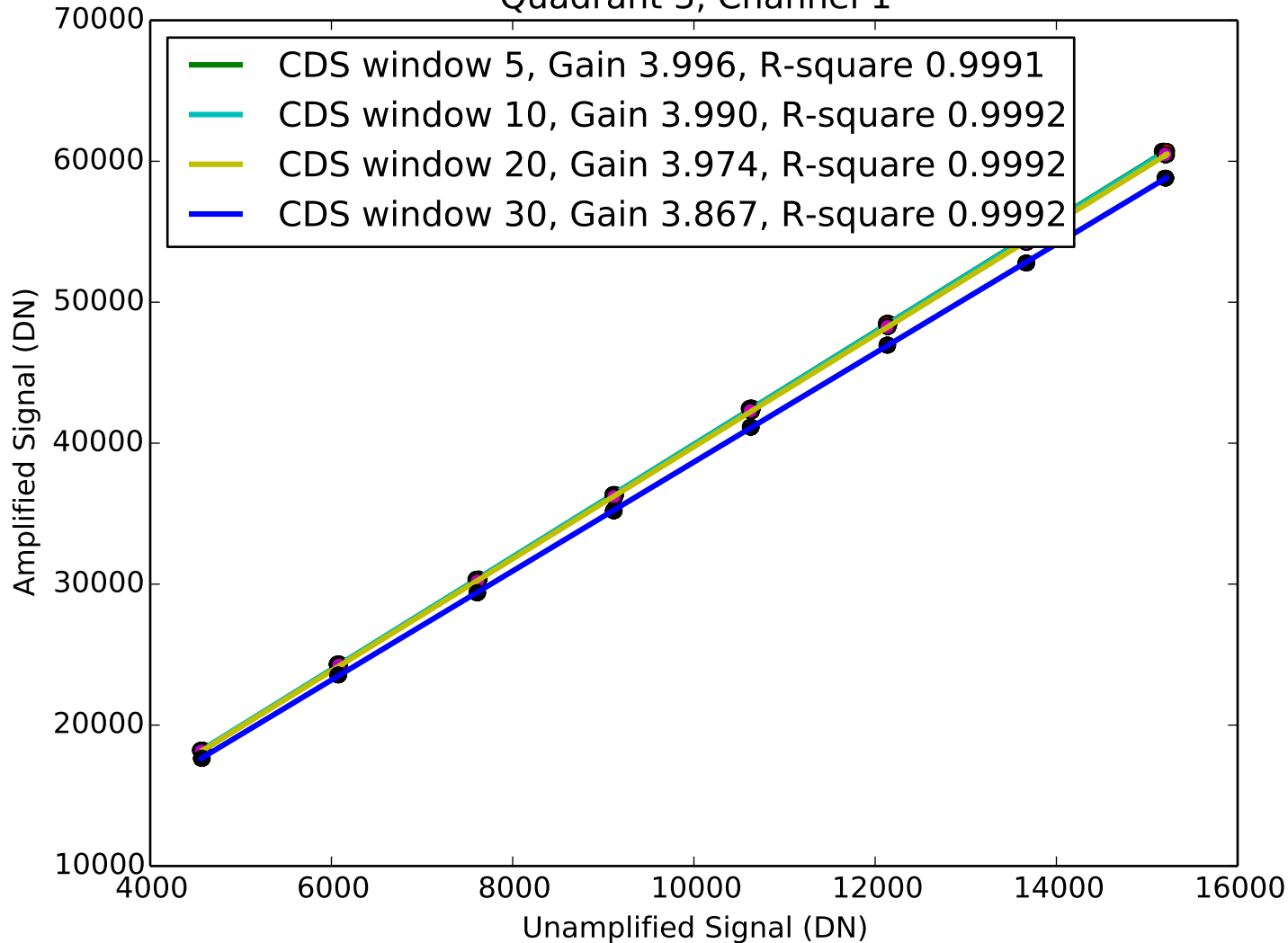
Signal vs Amplified Signal Quadrant 3, Channel 1
