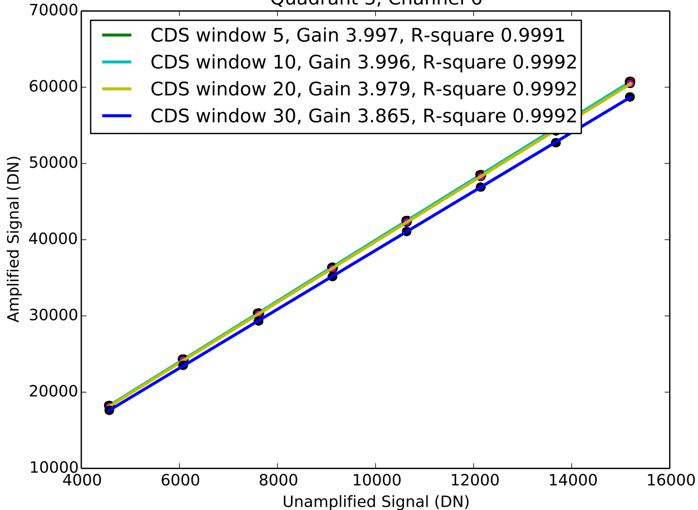
Signal vs Amplified Signal Quadrant 3, Channel 6
