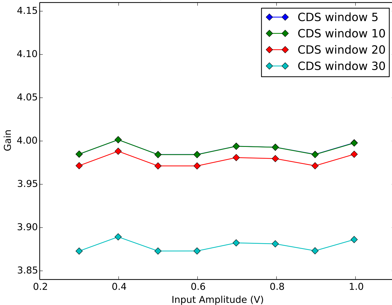
Average Amplifier Gain vs Amplifier Input Amplitude Quadrant 3, Channel 3
