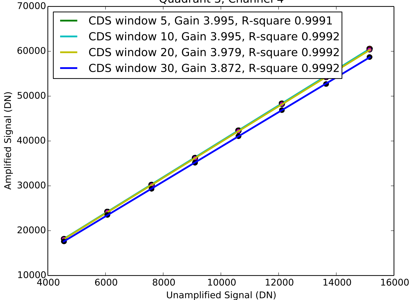
Signal vs Amplified Signal Quadrant 3, Channel 4
