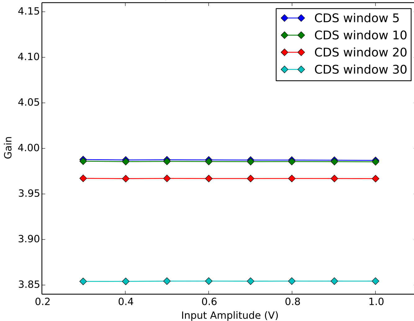
Average Amplifier Gain vs Amplifier Input Amplitude Quadrant 3, Channel 15
