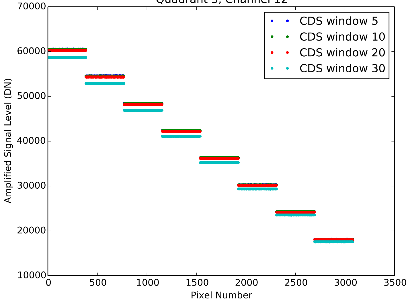
Amplified Signal Level from CDS Quadrant 3, Channel 12
