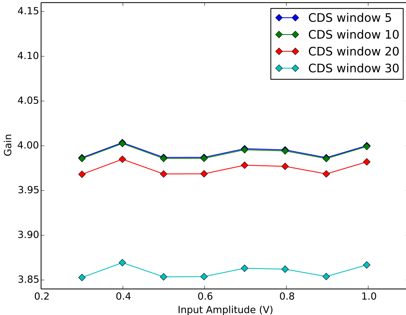
Average Amplifier Gain vs Amplifier Input Amplitude Quadrant 3, Channel 6
