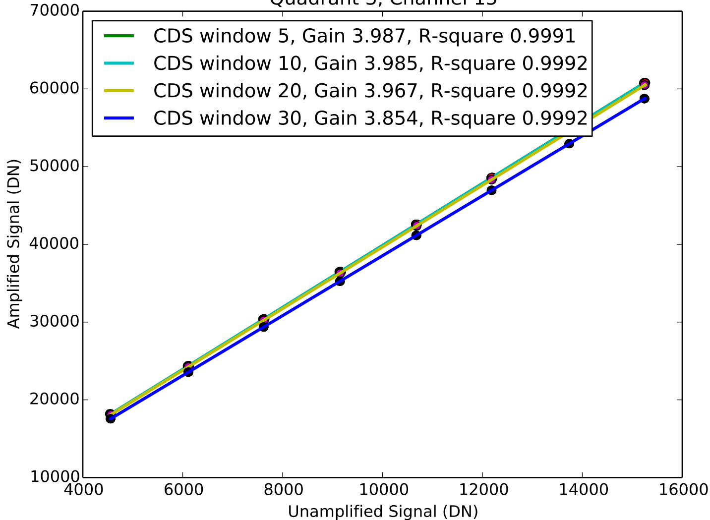
Signal vs Amplified Signal Quadrant 3, Channel 15
