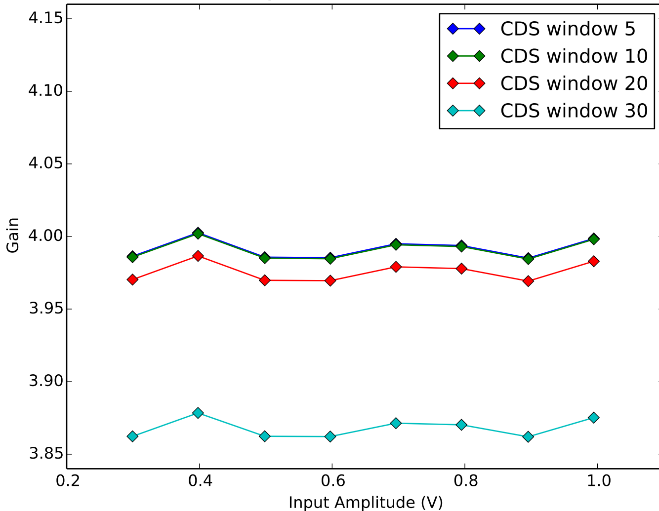
Average Amplifier Gain vs Amplifier Input Amplitude Quadrant 3, Channel 4
