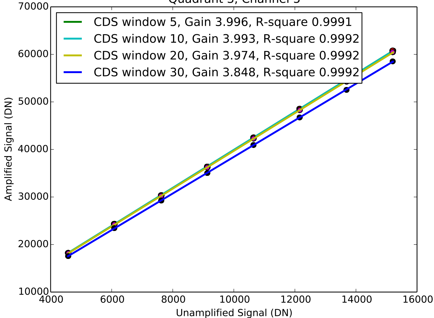
Signal vs Amplified Signal Quadrant 3, Channel 5
