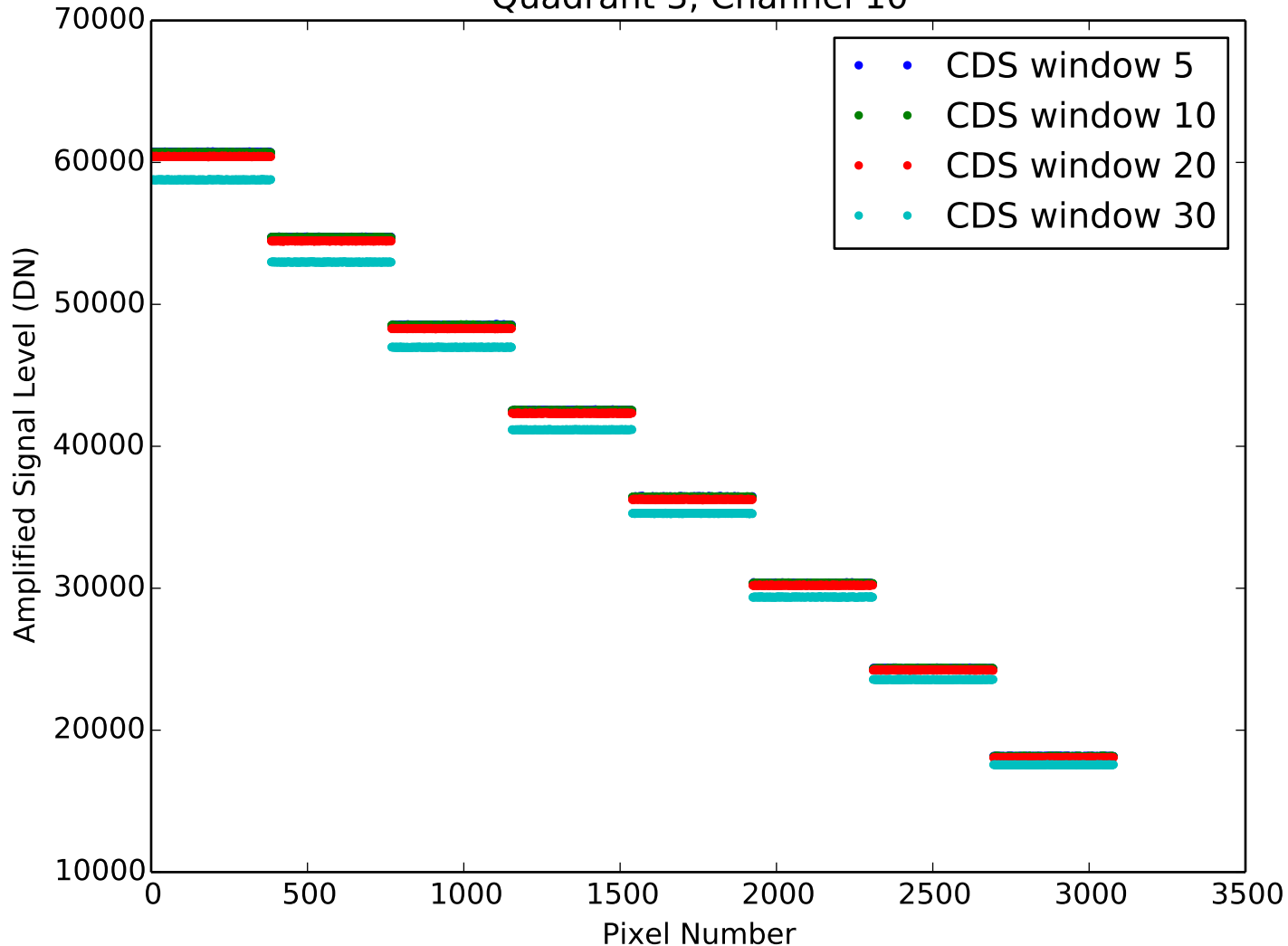
Amplified Signal Level from CDS Quadrant 3, Channel 10
