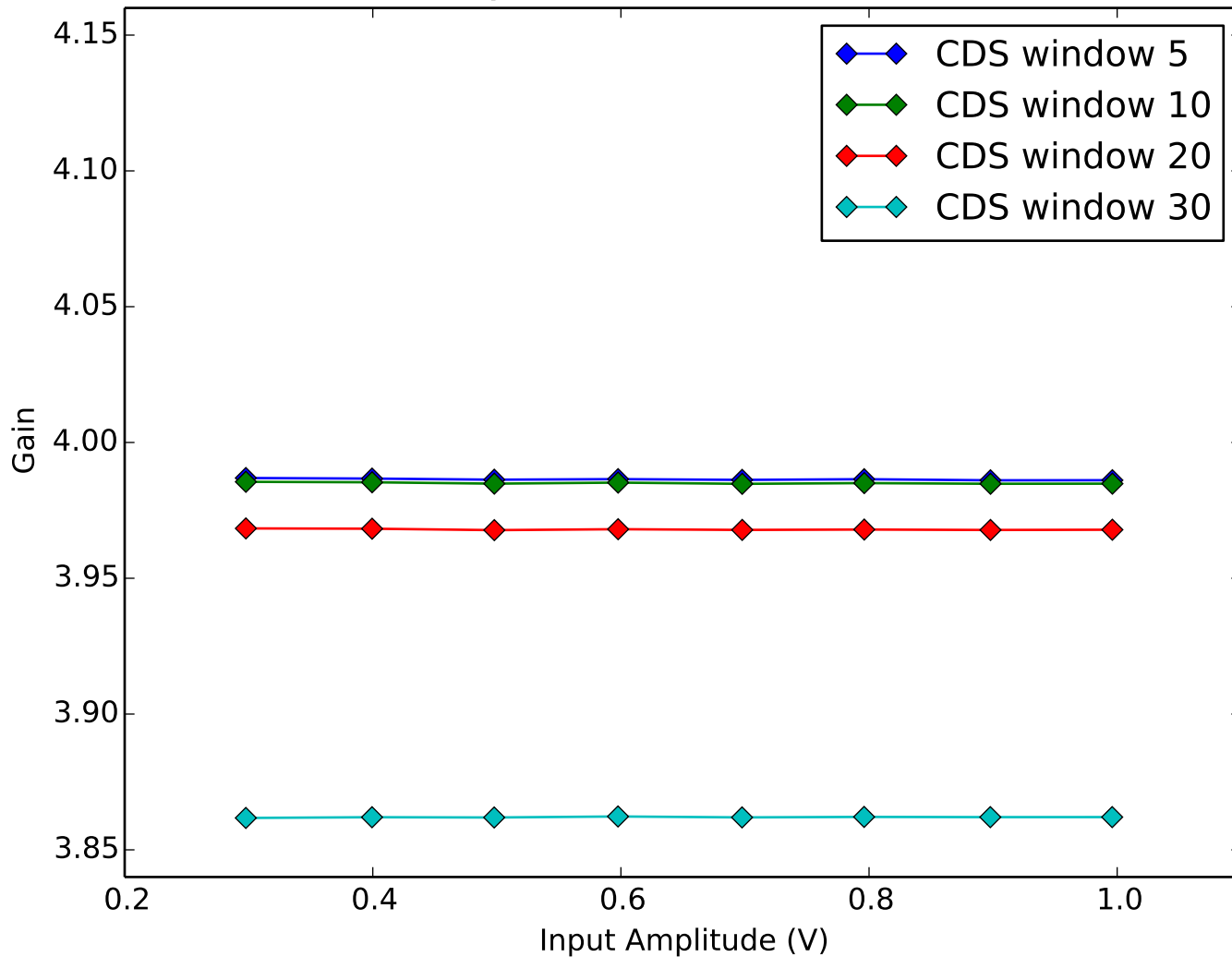
Average Amplifier Gain vs Amplifier Input Amplitude Quadrant 3, Channel 11
