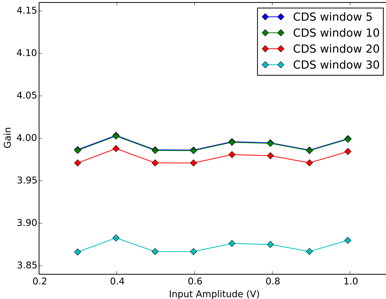
Average Amplifier Gain vs Amplifier Input Amplitude Quadrant 3, Channel 2
