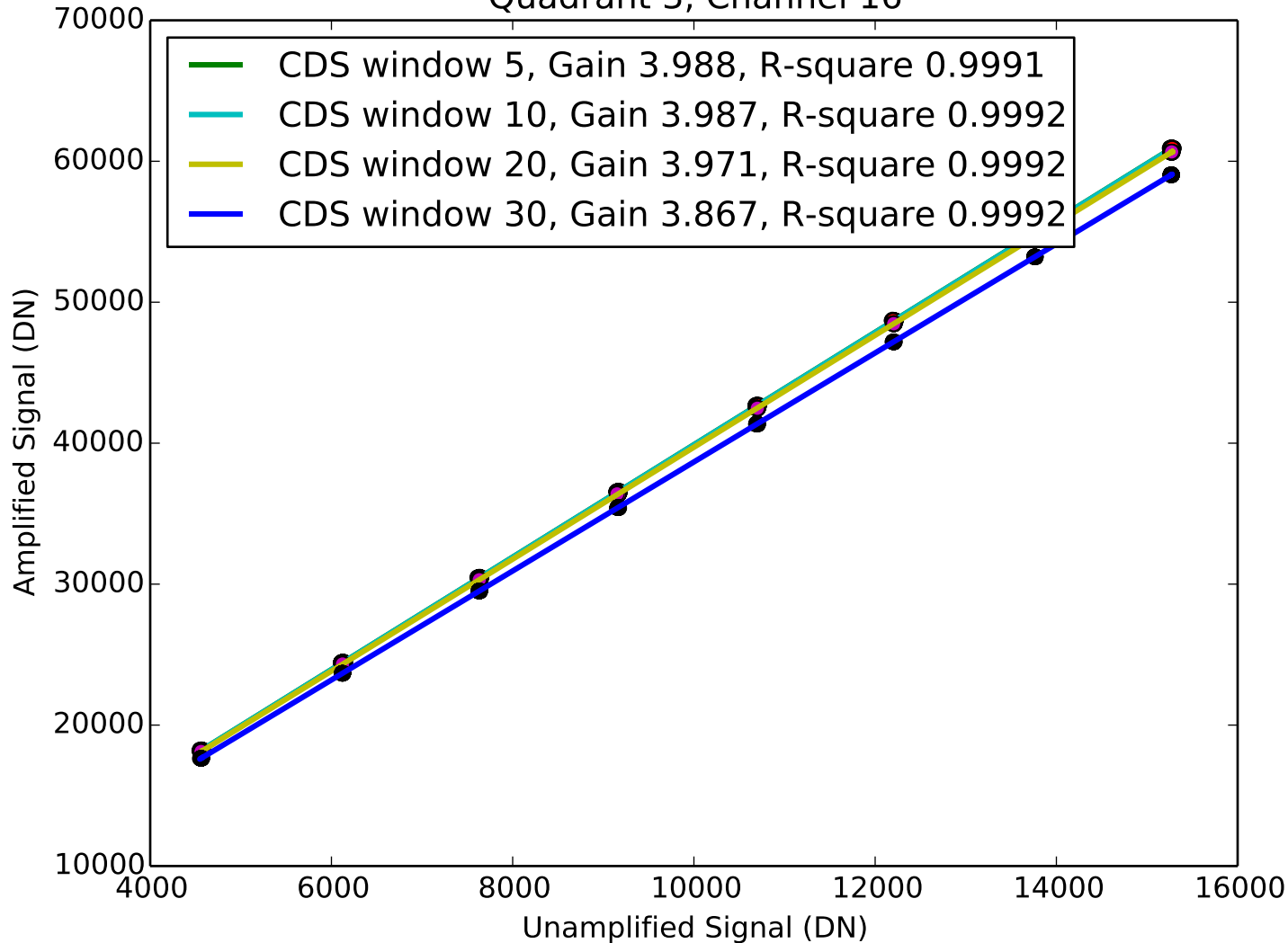
Signal vs Amplified Signal Quadrant 3, Channel 16
