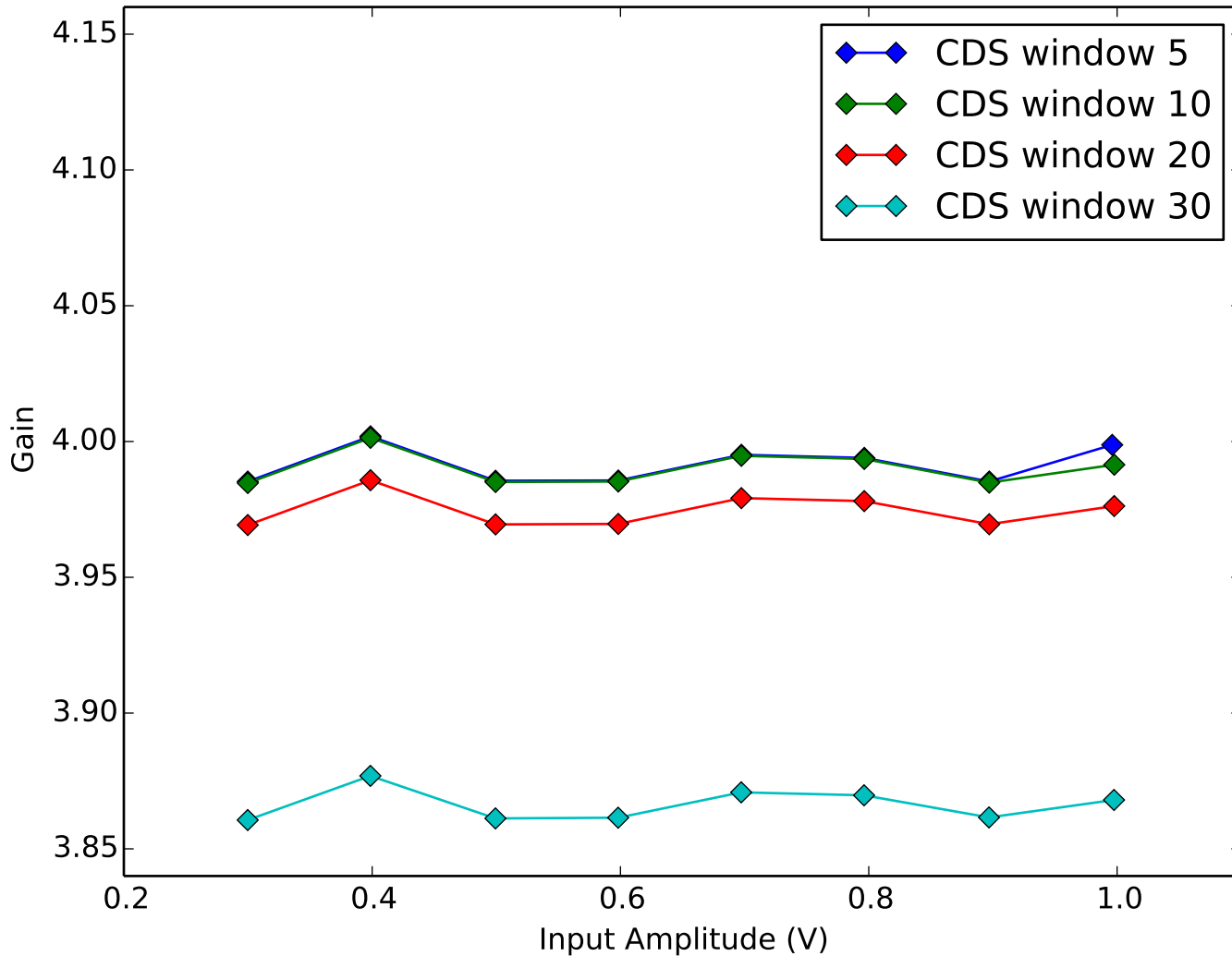
Average Amplifier Gain vs Amplifier Input Amplitude Quadrant 3, Channel 1
