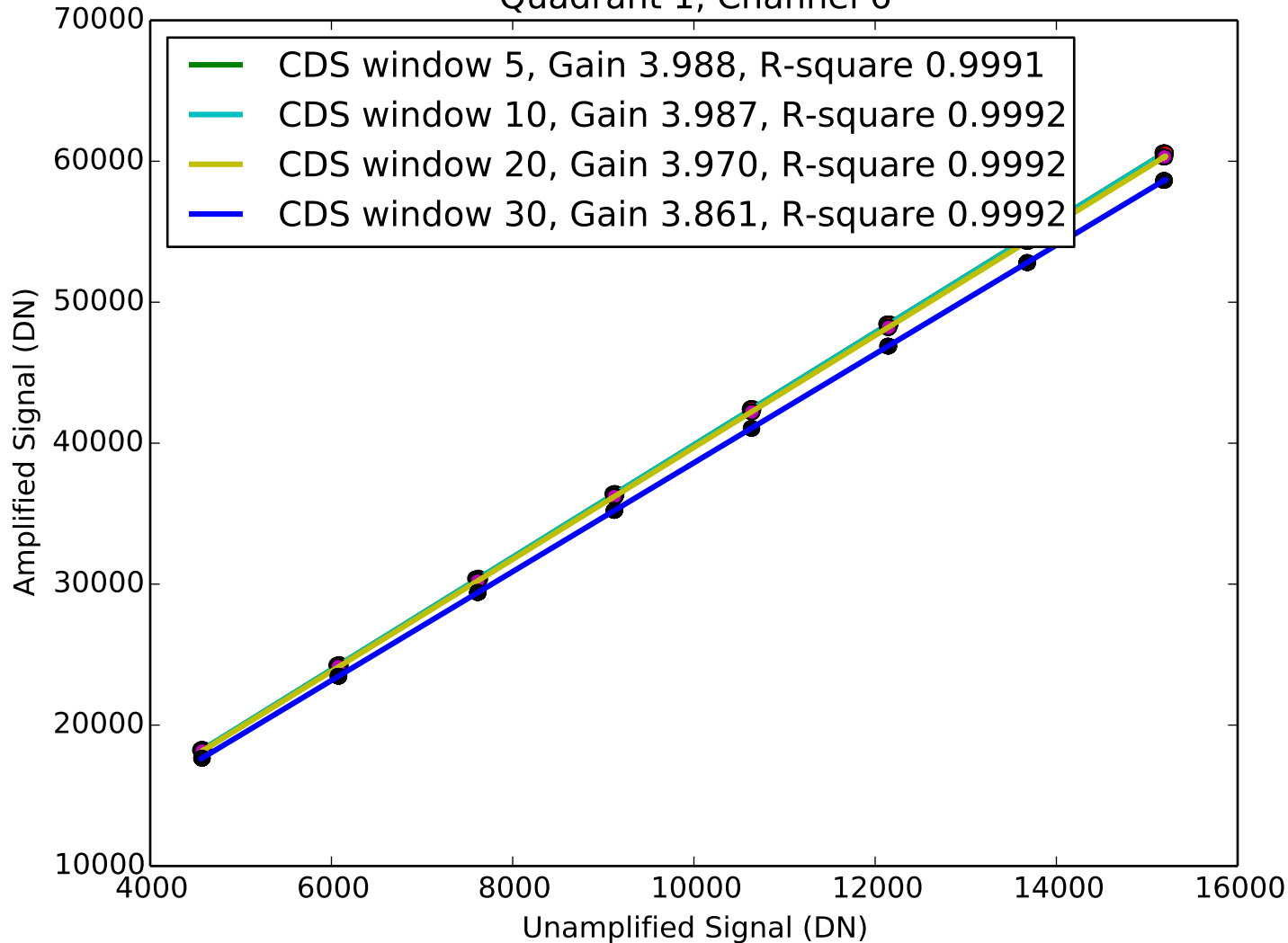
Signal vs Amplified Signal Quadrant 1, Channel 6
