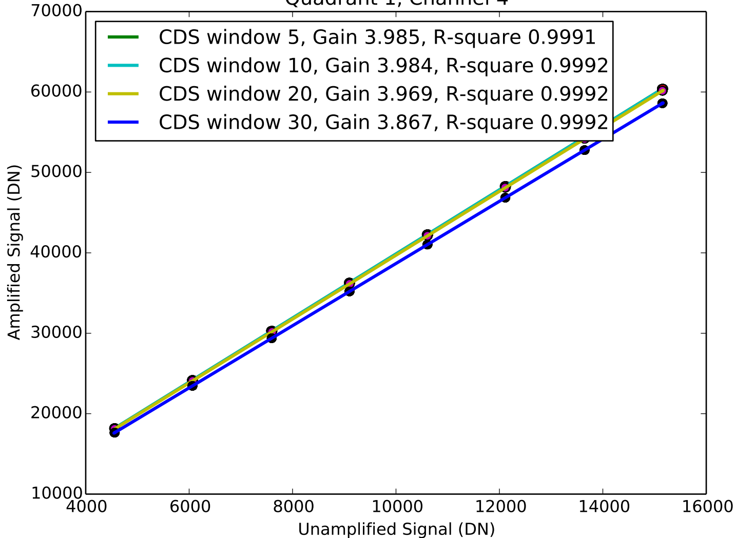
Signal vs Amplified Signal Quadrant 1, Channel 4
