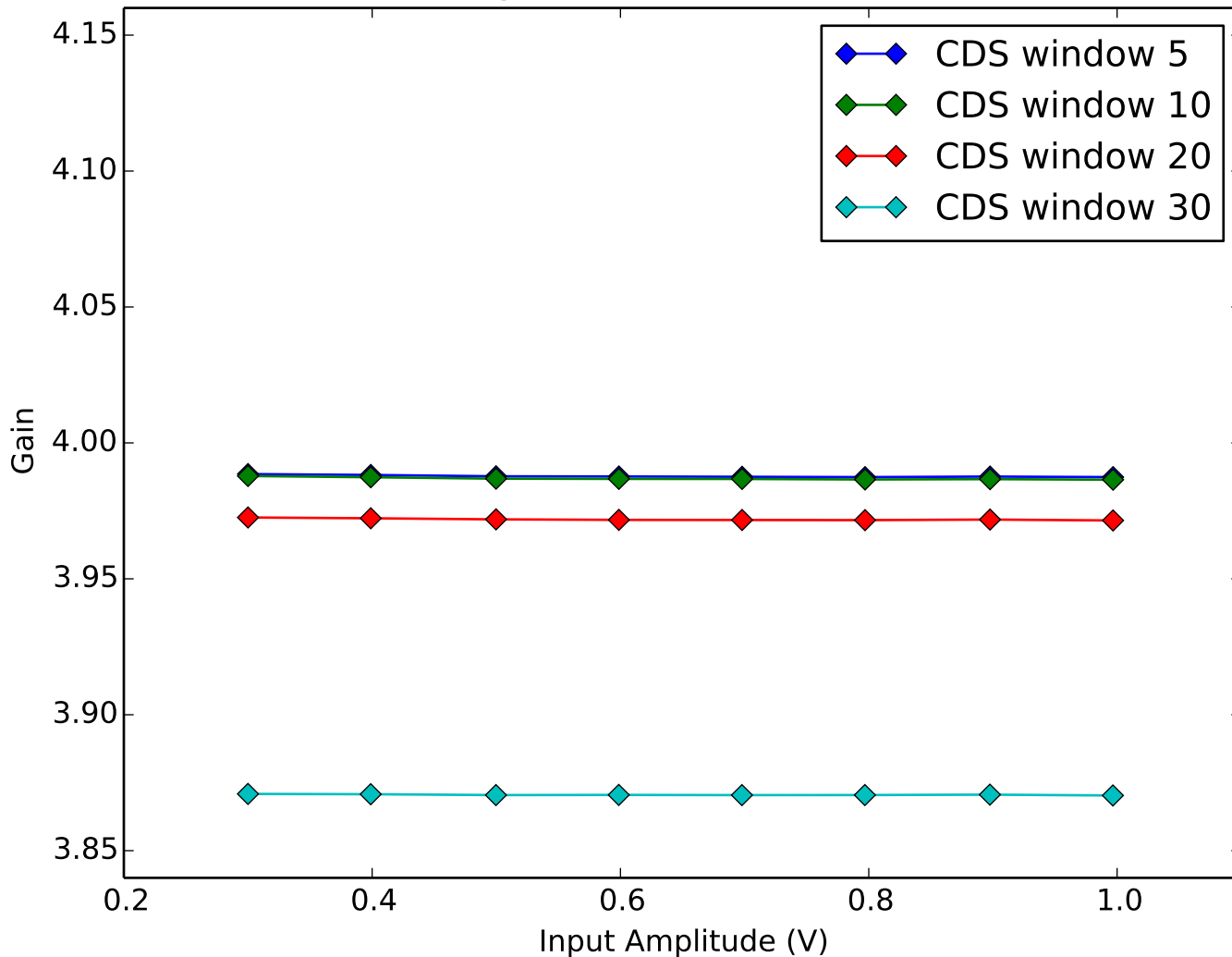
Average Amplifier Gain vs Amplifier Input Amplitude Quadrant 1, Channel 3
