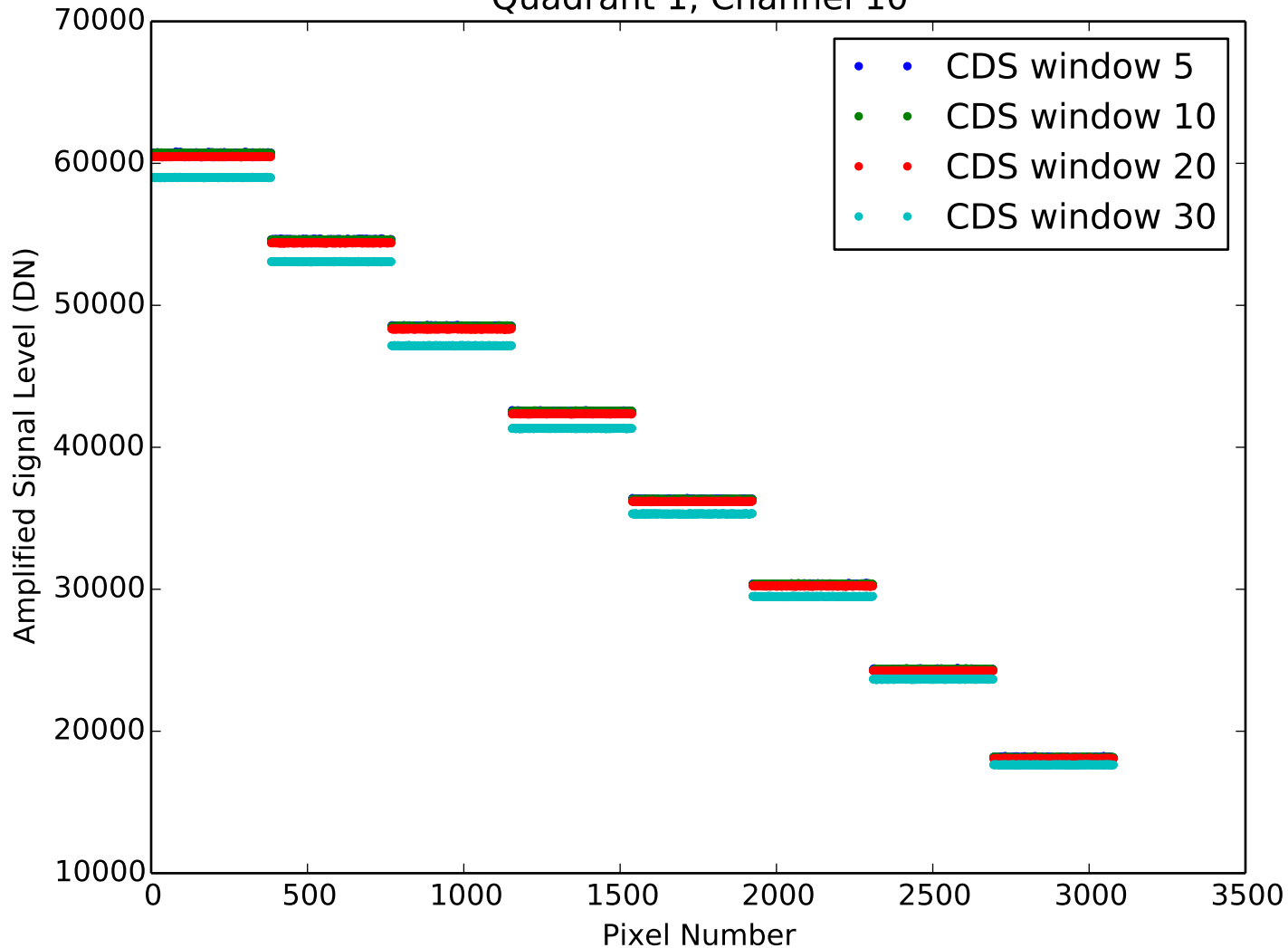
Amplified Signal Level from CDS Quadrant 1, Channel 10
