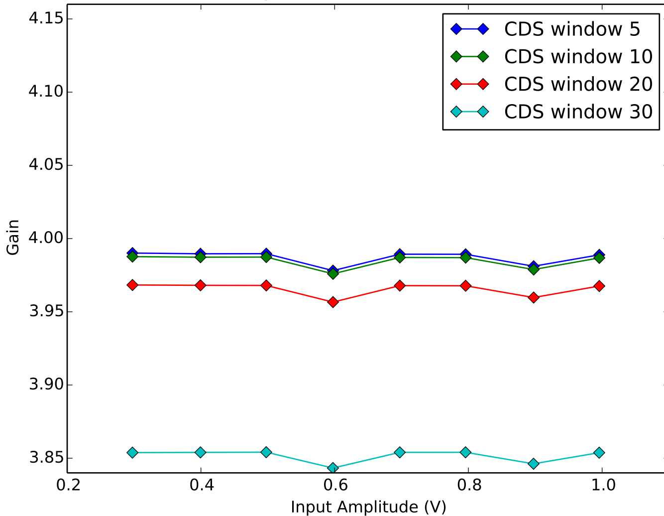
Average Amplifier Gain vs Amplifier Input Amplitude Quadrant 1, Channel 12
