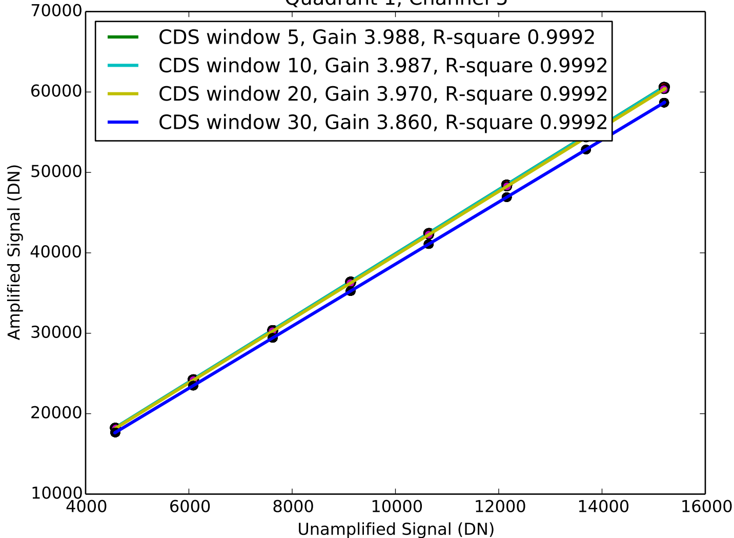
Signal vs Amplified Signal Quadrant 1, Channel 5
