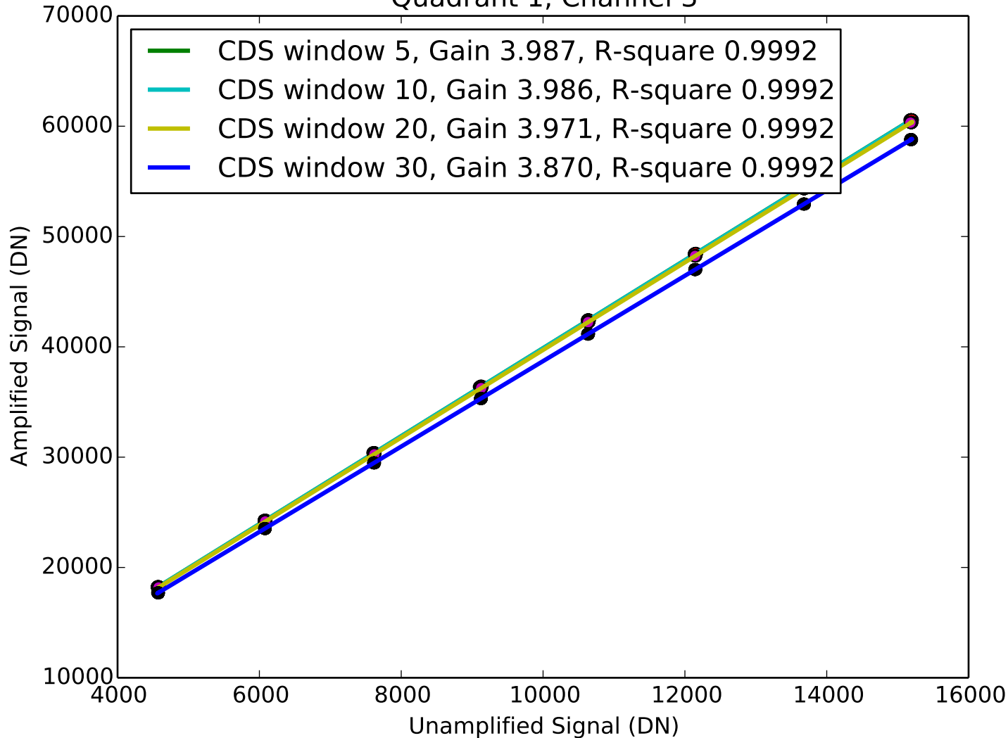
Signal vs Amplified Signal Quadrant 1, Channel 3
