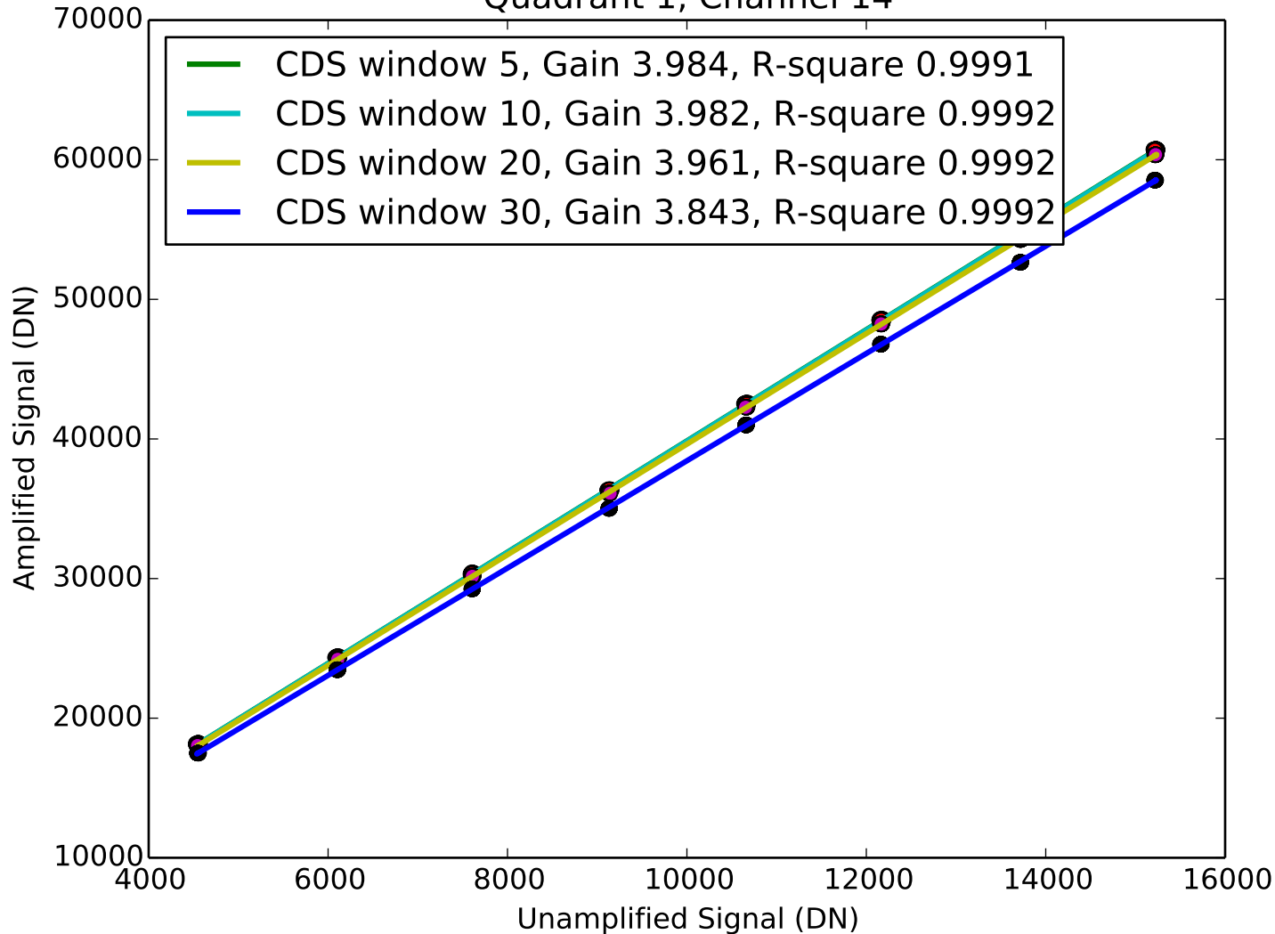
Signal vs Amplified Signal Quadrant 1, Channel 14
