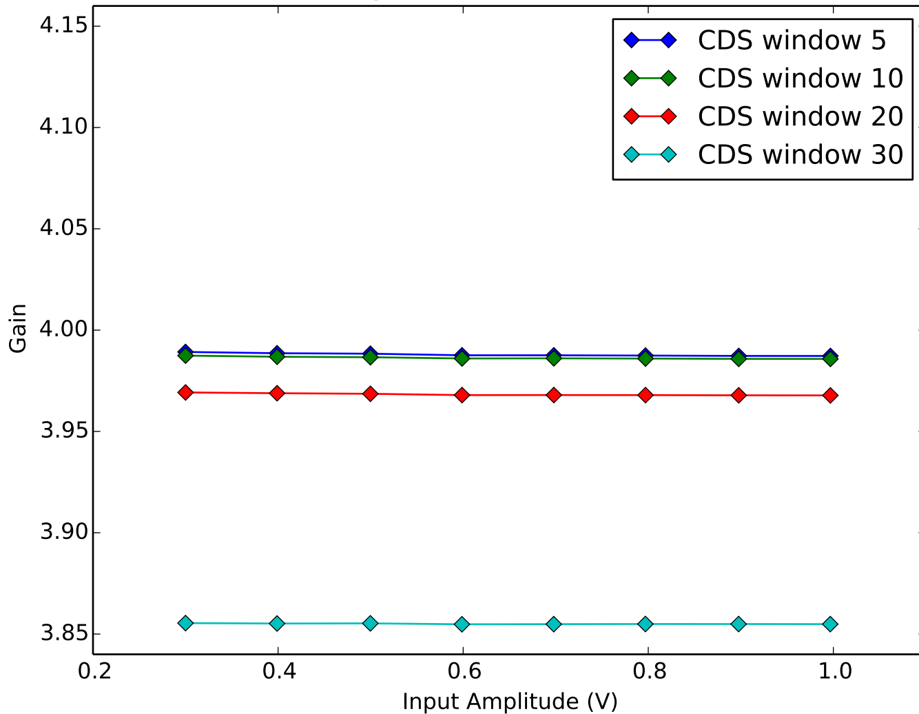
Average Amplifier Gain vs Amplifier Input Amplitude Quadrant 1, Channel 8
