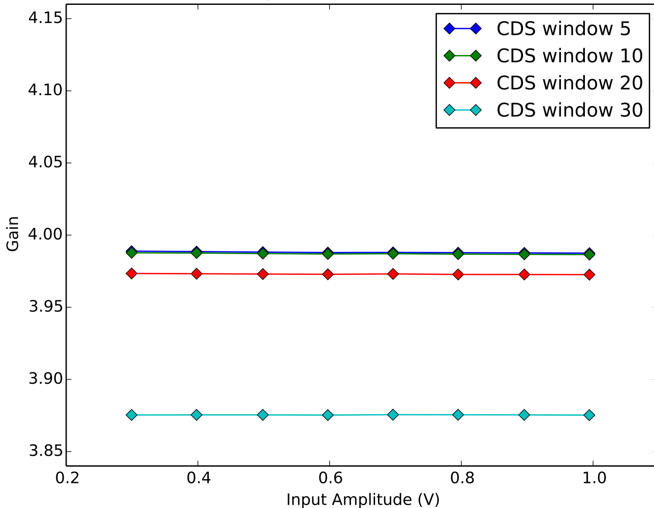
Average Amplifier Gain vs Amplifier Input Amplitude Quadrant 1, Channel 2
