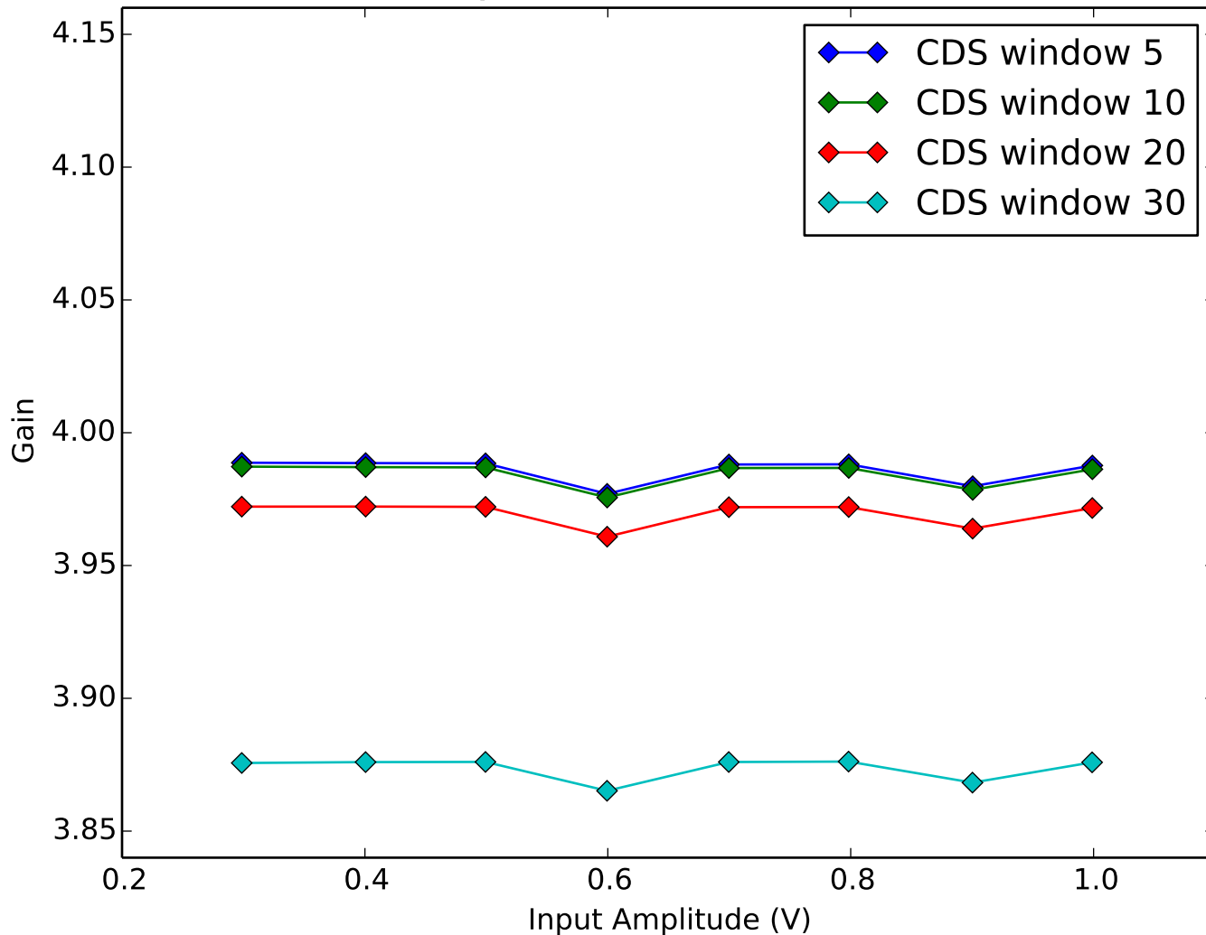
Average Amplifier Gain vs Amplifier Input Amplitude Quadrant 1, Channel 10
