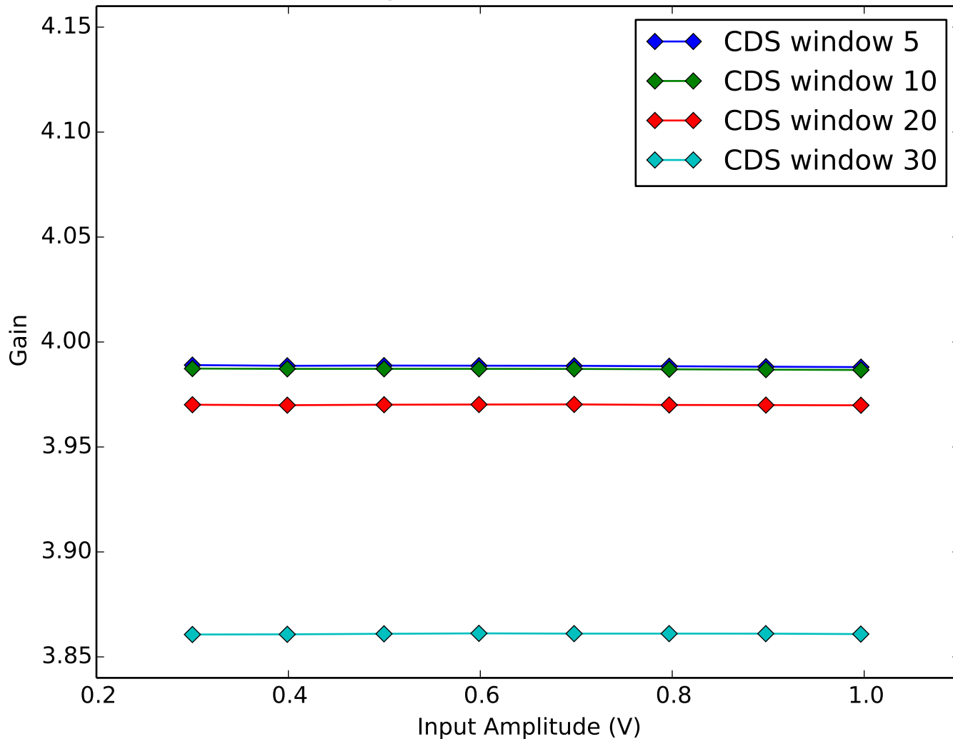
Average Amplifier Gain vs Amplifier Input Amplitude Quadrant 1, Channel 6
