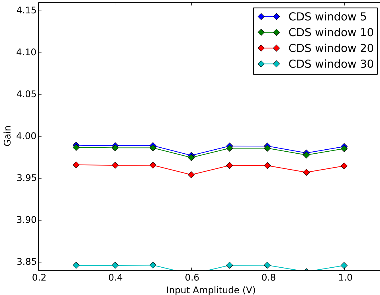
Average Amplifier Gain vs Amplifier Input Amplitude Quadrant 1, Channel 14
