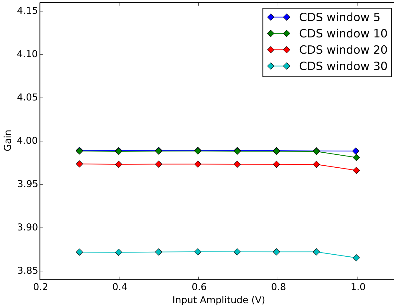
Average Amplifier Gain vs Amplifier Input Amplitude Quadrant 1, Channel 1
