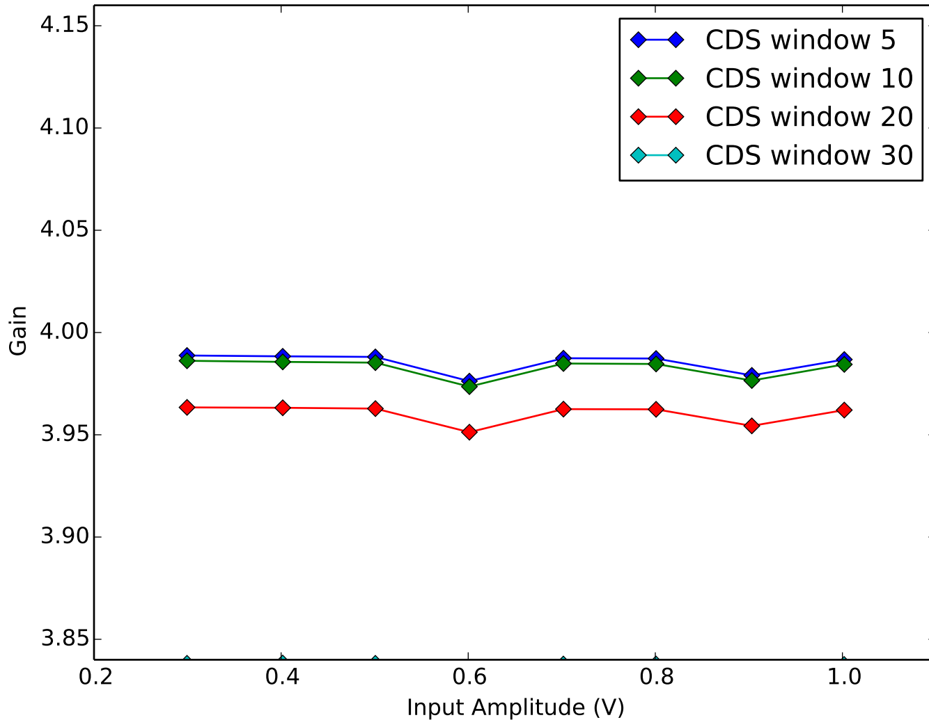
Average Amplifier Gain vs Amplifier Input Amplitude Quadrant 1, Channel 16
