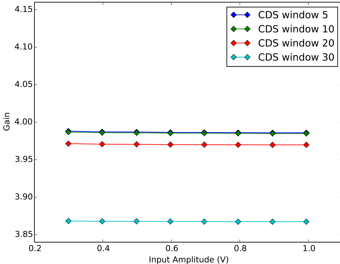
Average Amplifier Gain vs Amplifier Input Amplitude Quadrant 1, Channel 4
