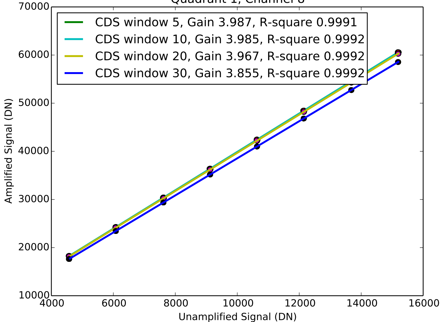
Signal vs Amplified Signal Quadrant 1, Channel 8
