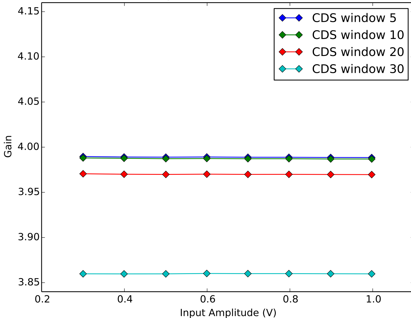
Average Amplifier Gain vs Amplifier Input Amplitude Quadrant 1, Channel 5
