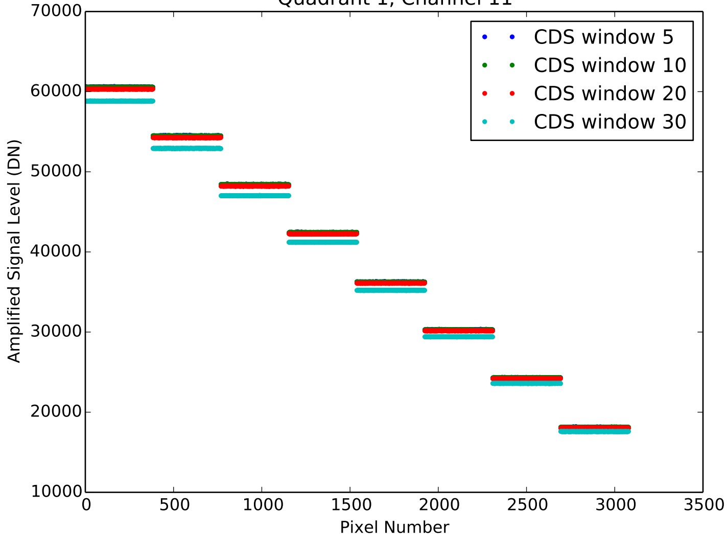
Amplified Signal Level from CDS Quadrant 1, Channel 11
