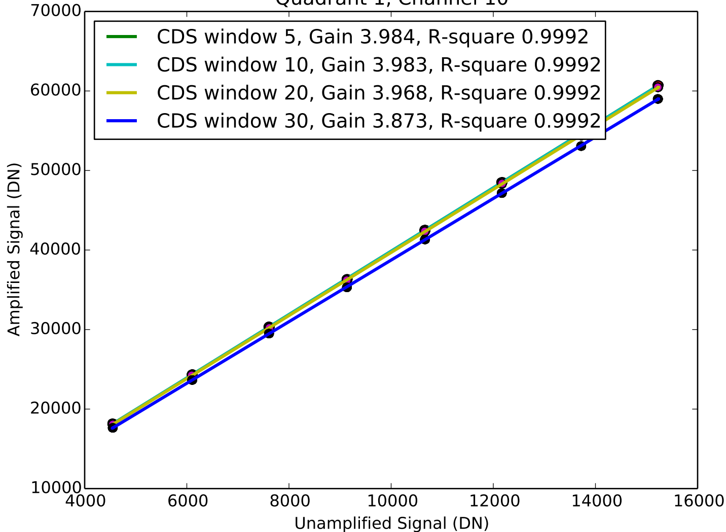
Signal vs Amplified Signal Quadrant 1, Channel 10
