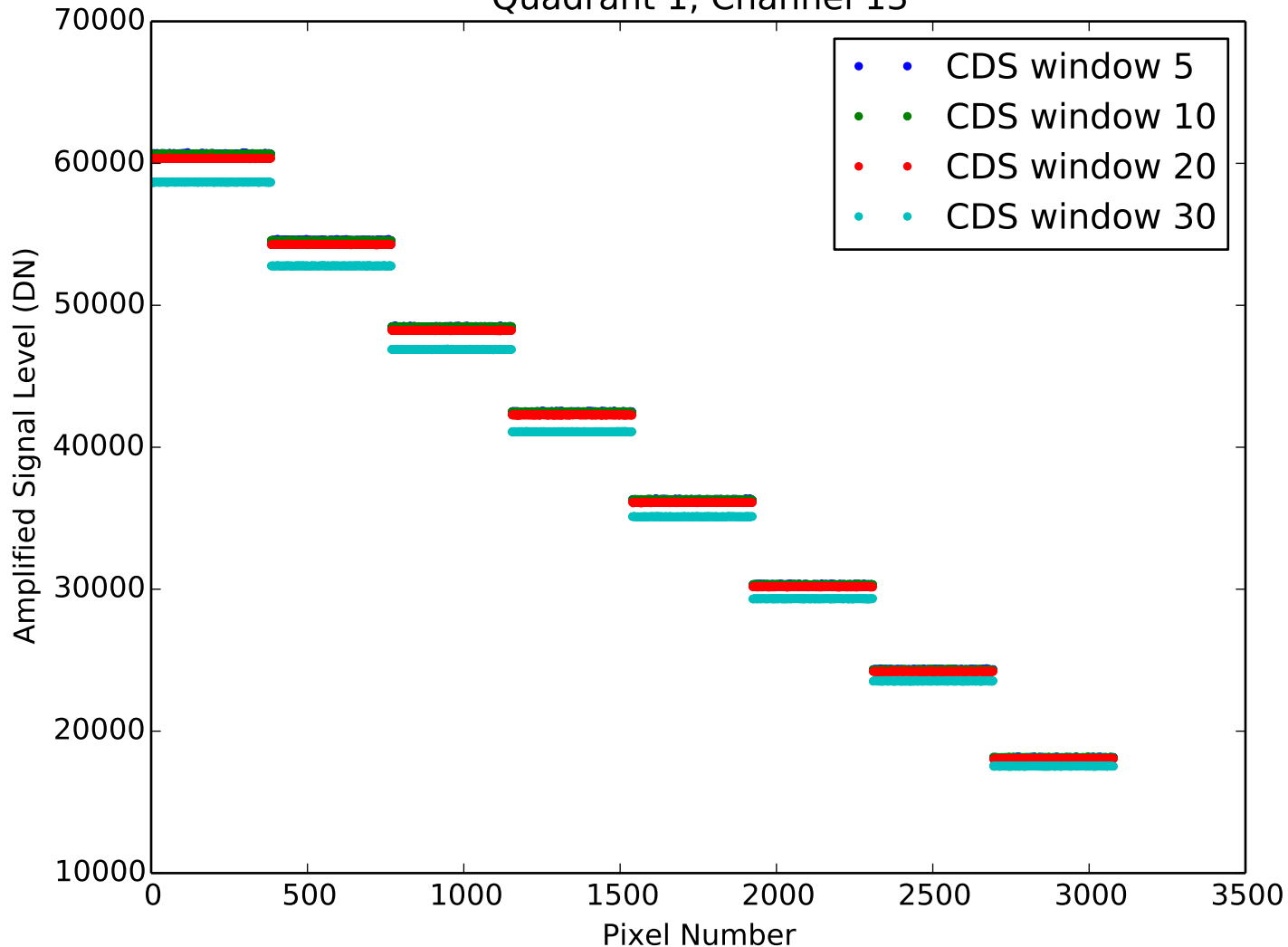
Amplified Signal Level from CDS Quadrant 1, Channel 13
