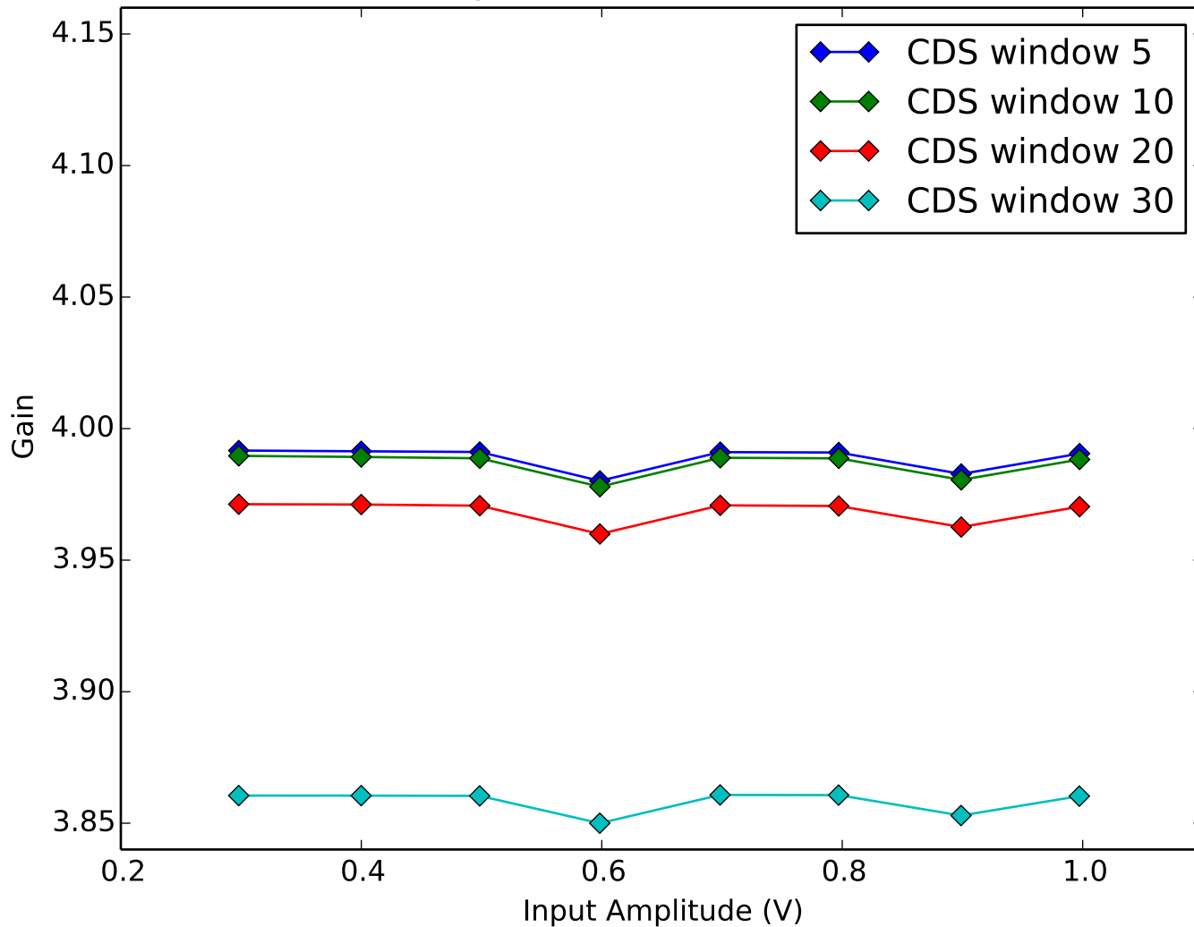
Average Amplifier Gain vs Amplifier Input Amplitude Quadrant 1, Channel 13
