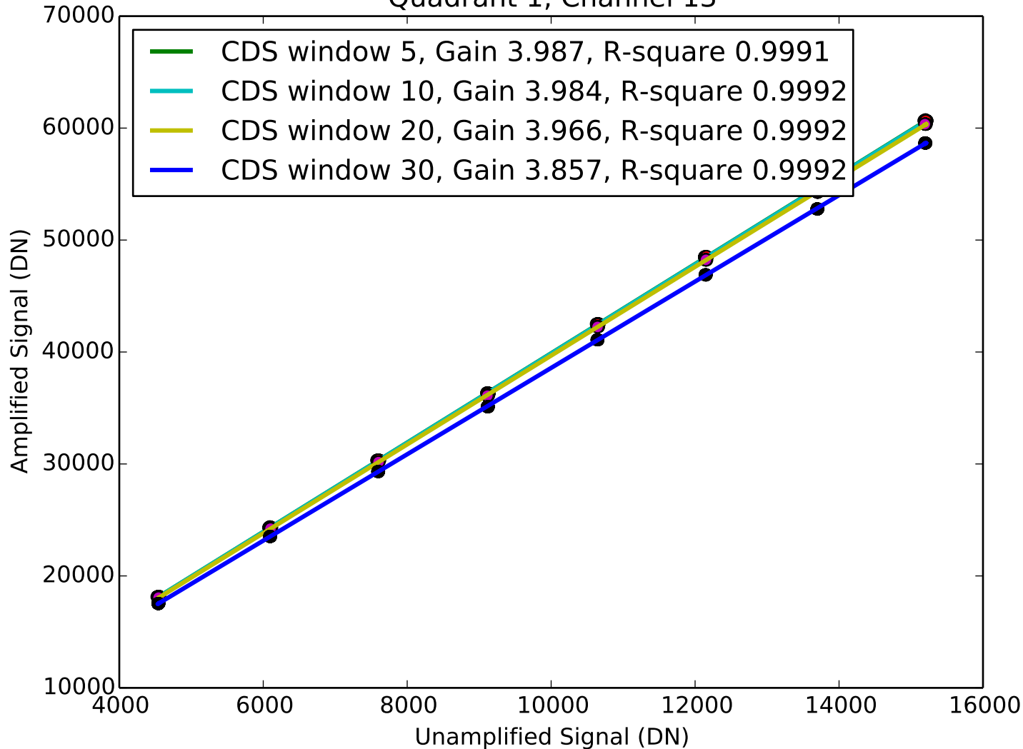
Signal vs Amplified Signal Quadrant 1, Channel 13
