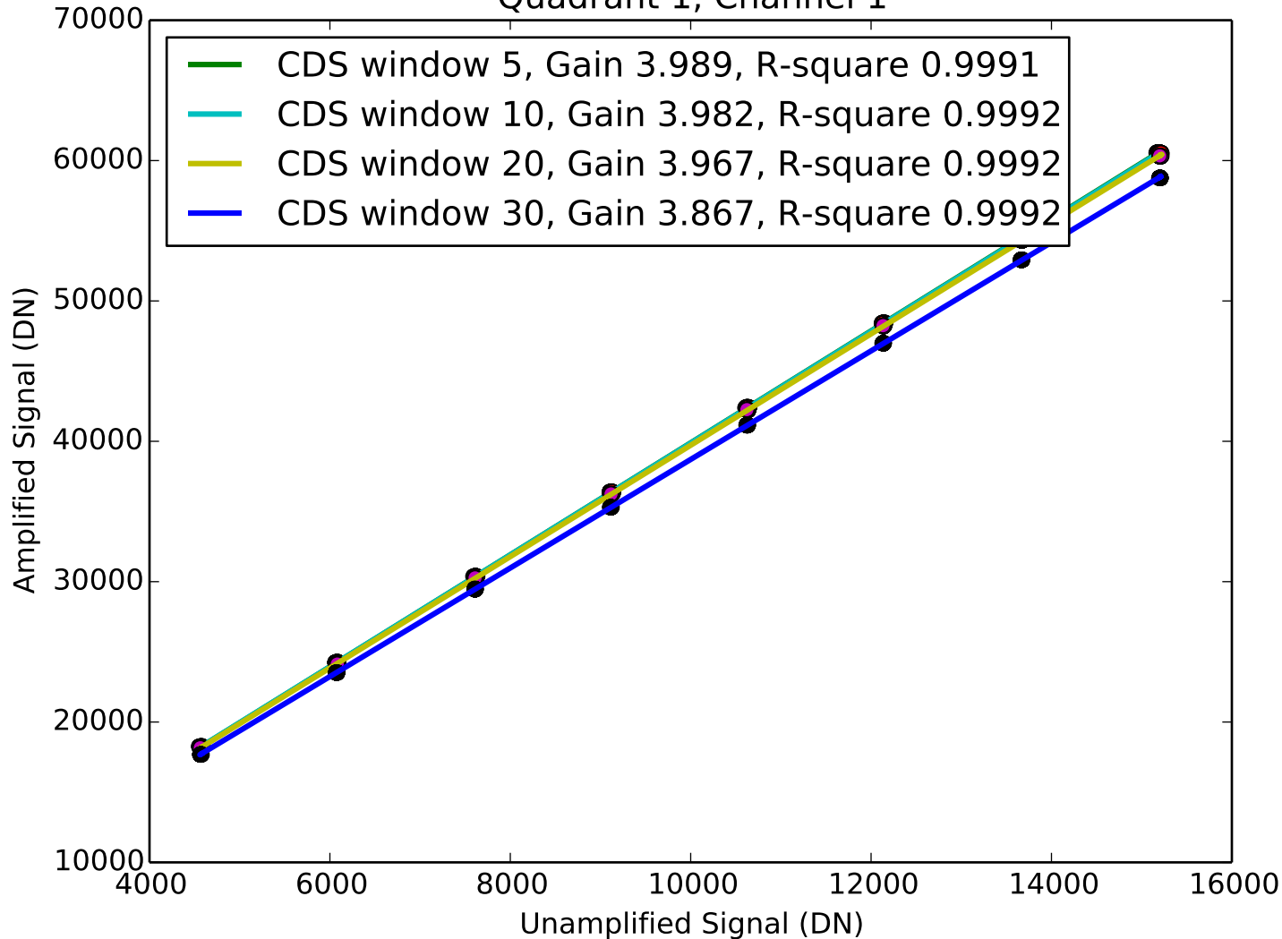
Signal vs Amplified Signal Quadrant 1, Channel 1
