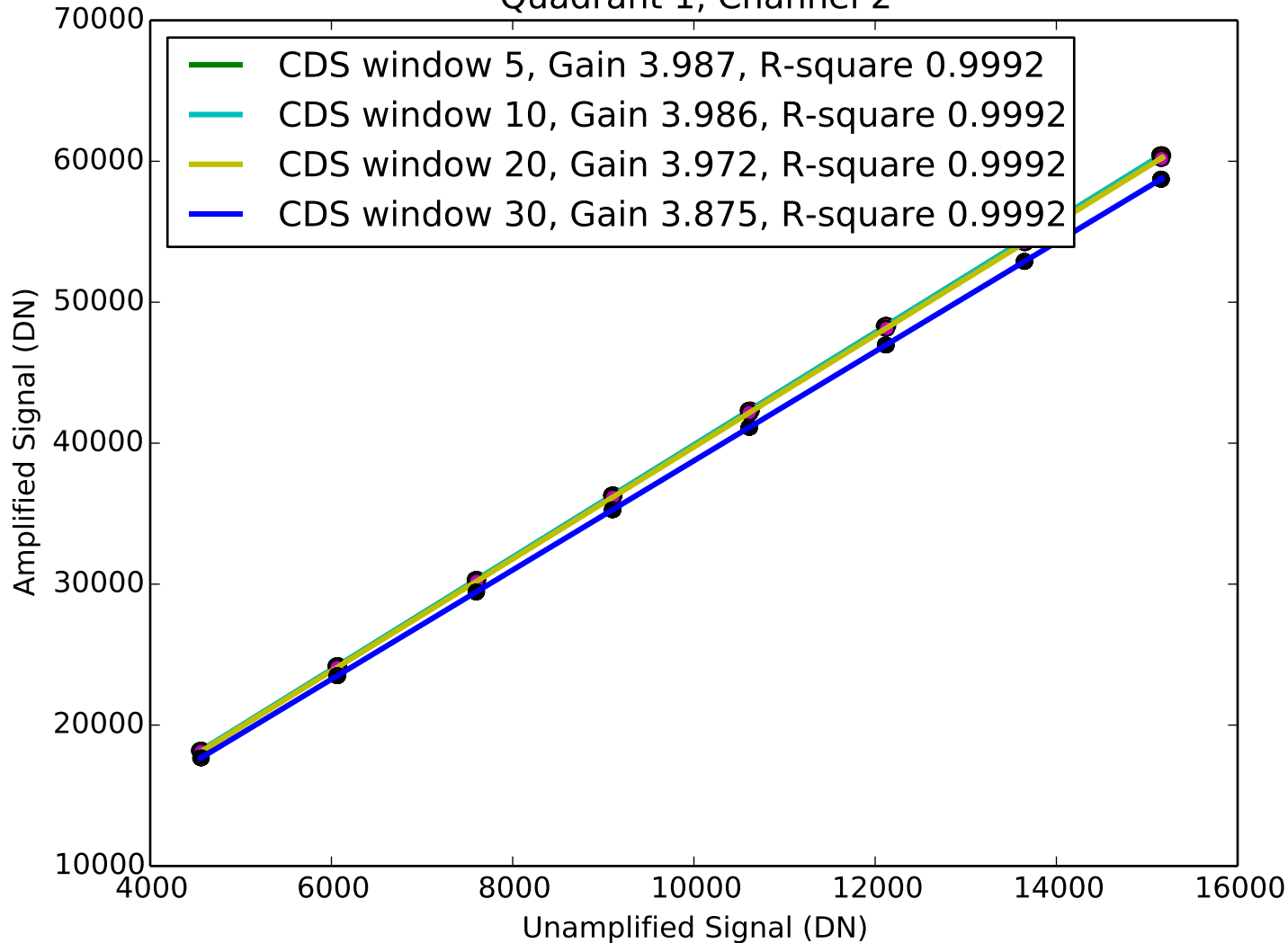
Signal vs Amplified Signal Quadrant 1, Channel 2
