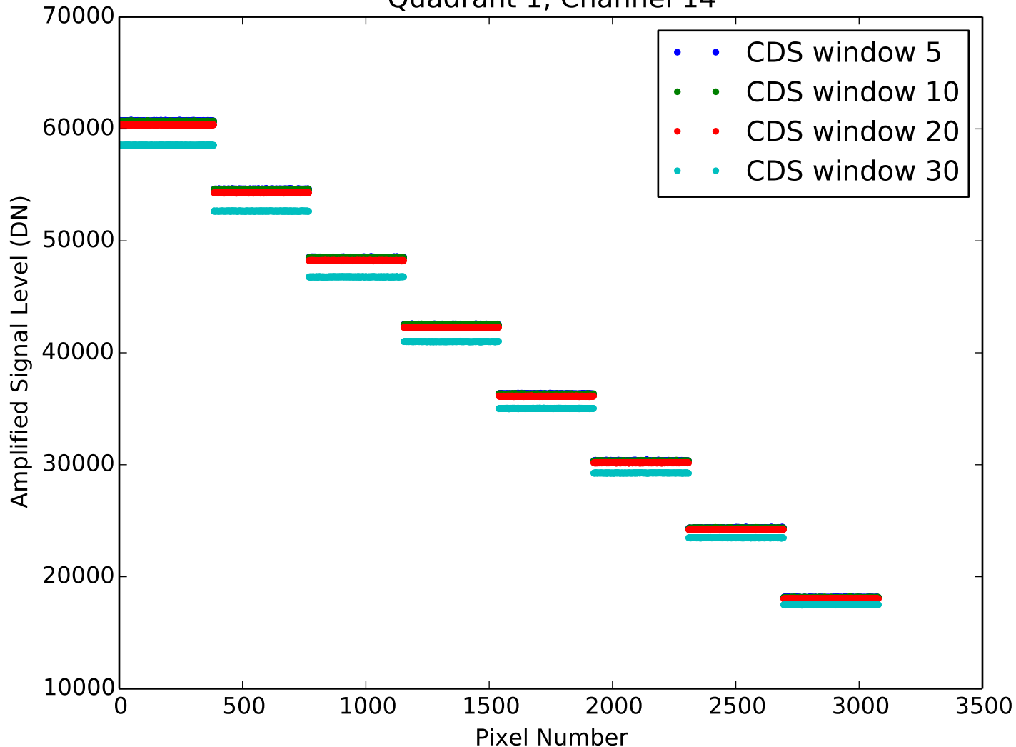
Amplified Signal Level from CDS Quadrant 1, Channel 14
