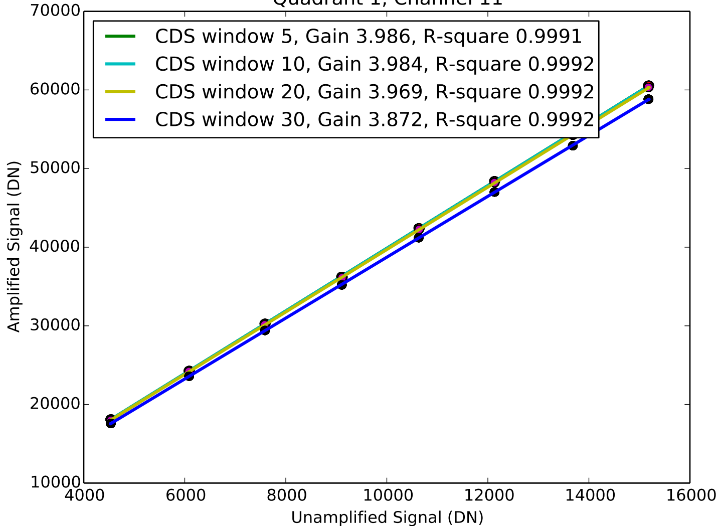
Signal vs Amplified Signal Quadrant 1, Channel 11
