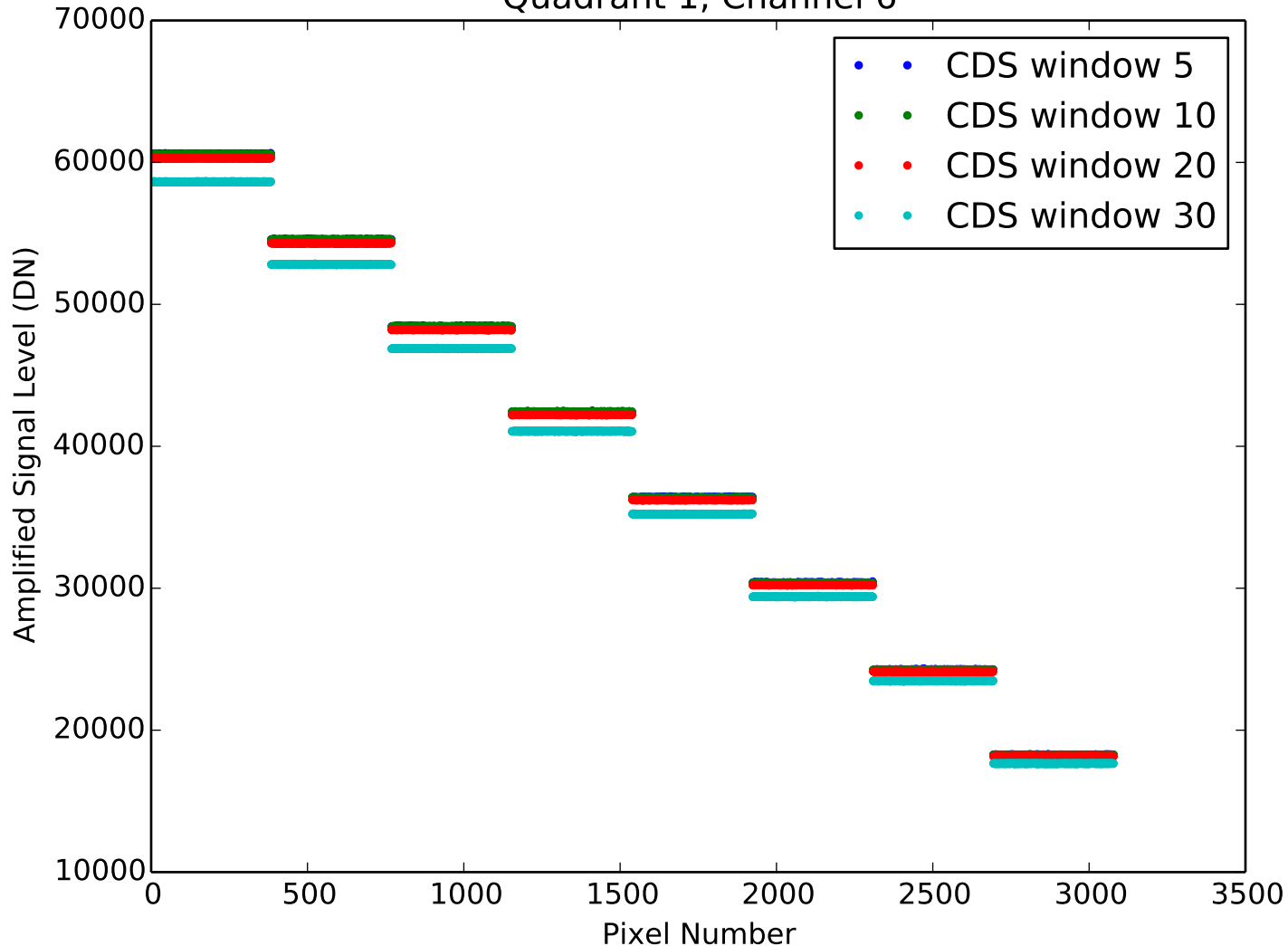
Amplified Signal Level from CDS Quadrant 1, Channel 6
