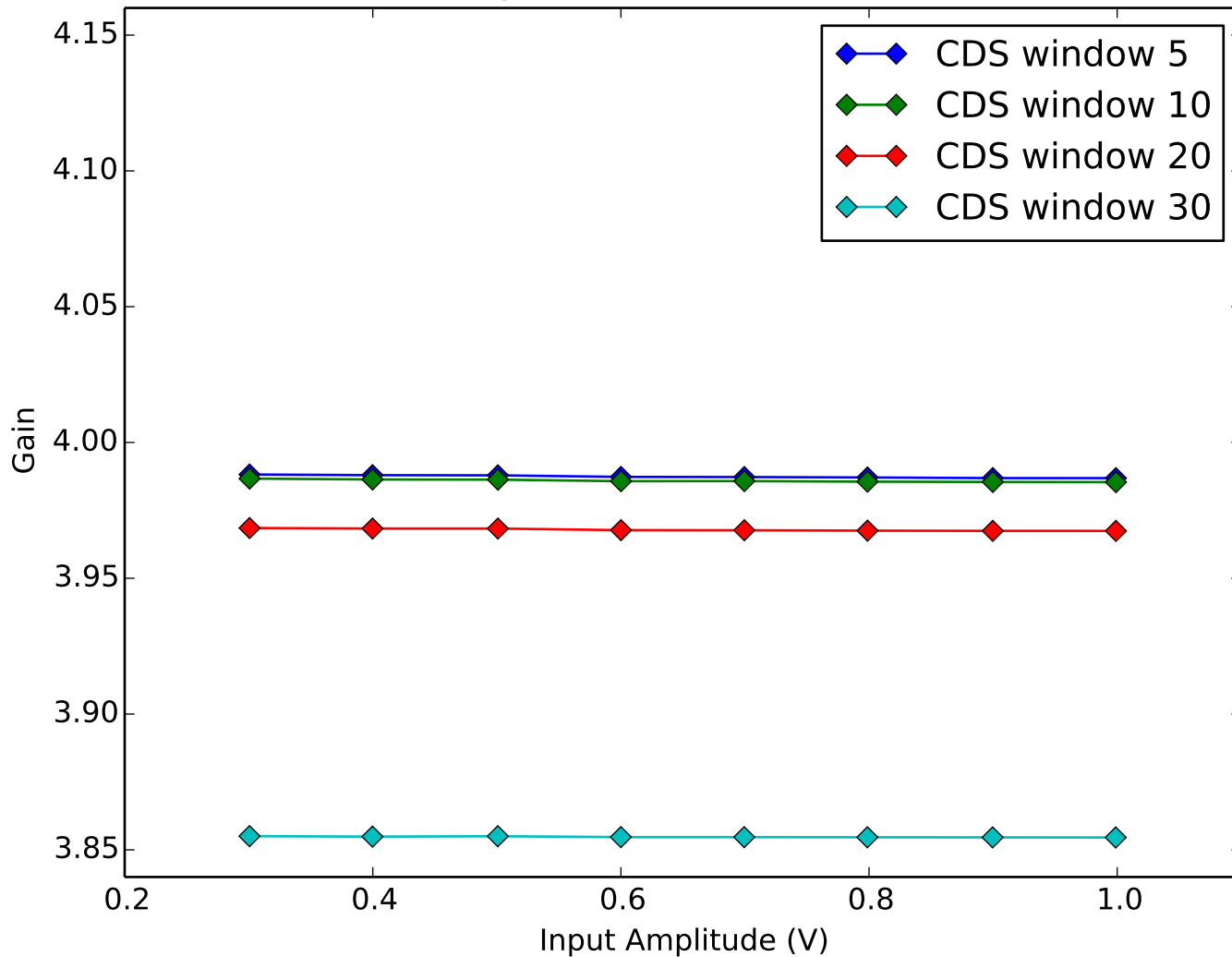
Average Amplifier Gain vs Amplifier Input Amplitude Quadrant 1, Channel 7
