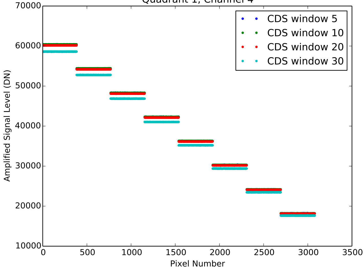
Amplified Signal Level from CDS Quadrant 1, Channel 4
