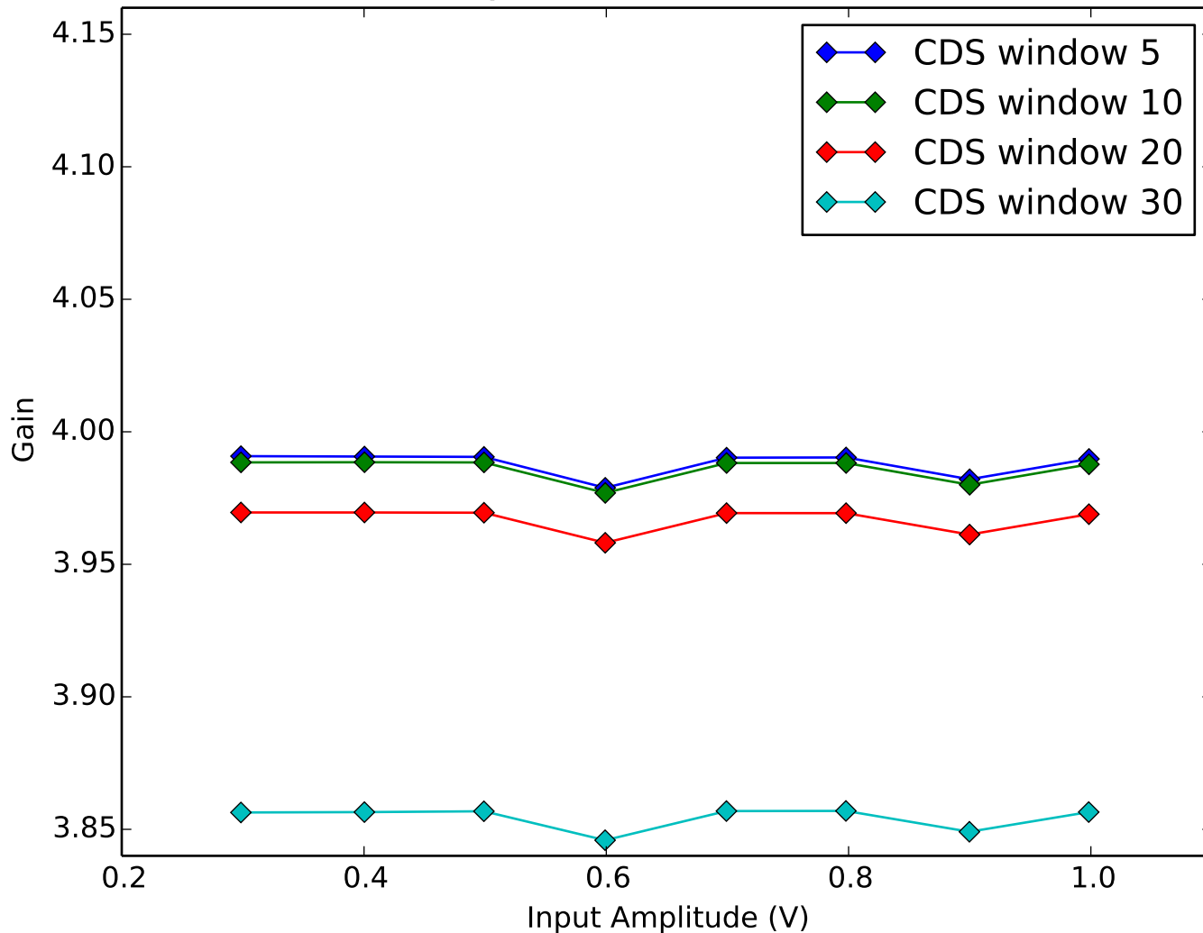
Average Amplifier Gain vs Amplifier Input Amplitude Quadrant 1, Channel 9
