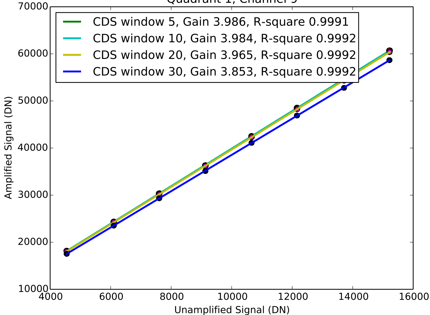
Signal vs Amplified Signal Quadrant 1, Channel 9
