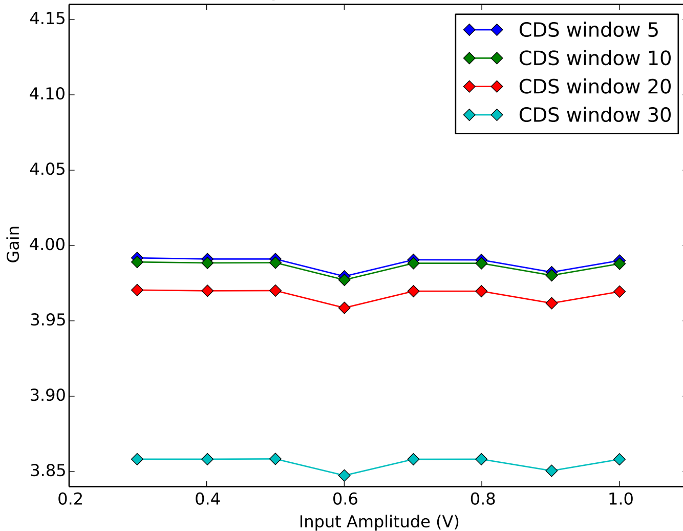
Average Amplifier Gain vs Amplifier Input Amplitude Quadrant 1, Channel 15
