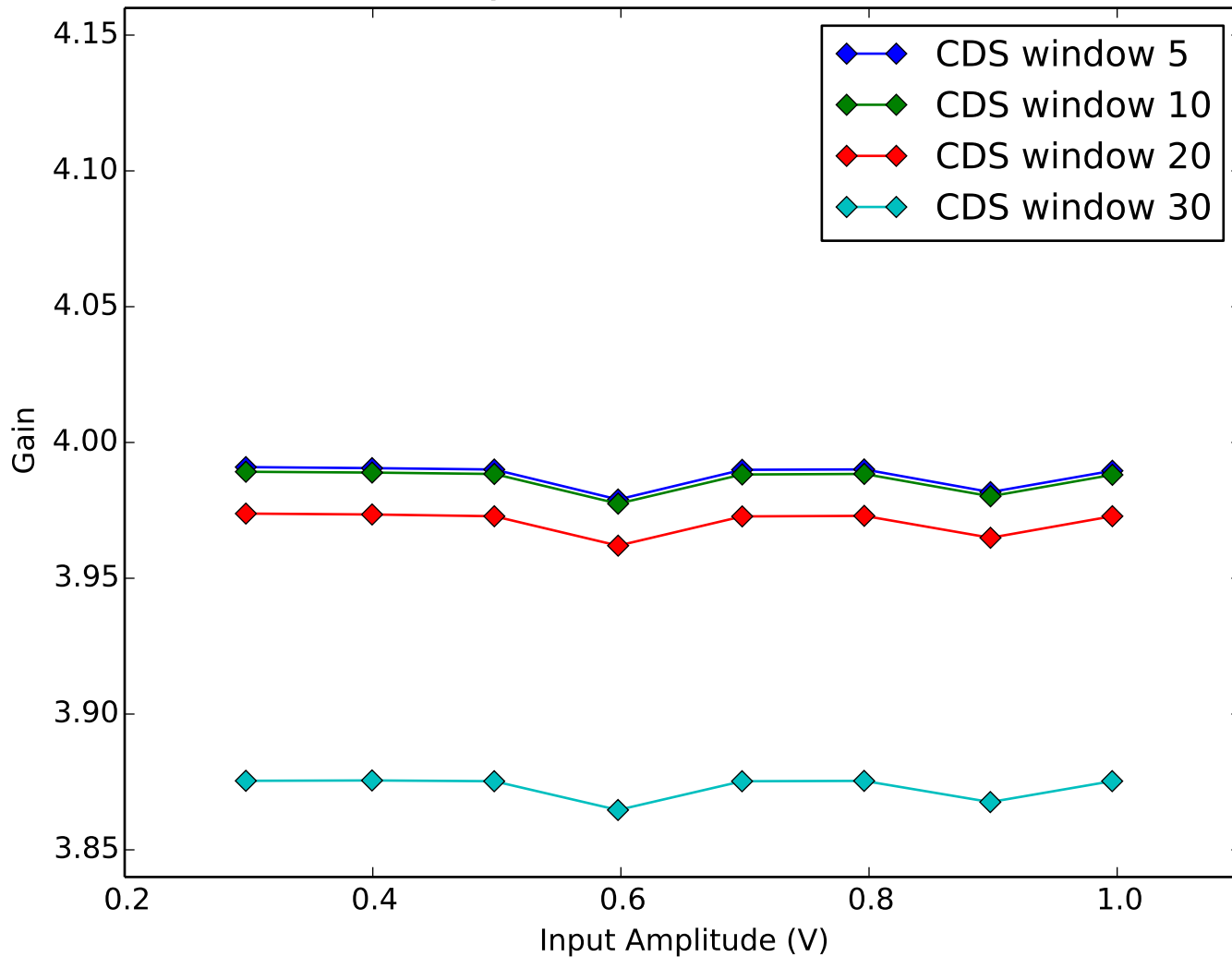
Average Amplifier Gain vs Amplifier Input Amplitude Quadrant 1, Channel 11
