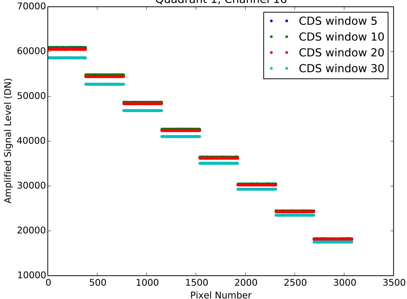
Amplified Signal Level from CDS Quadrant 1, Channel 16
