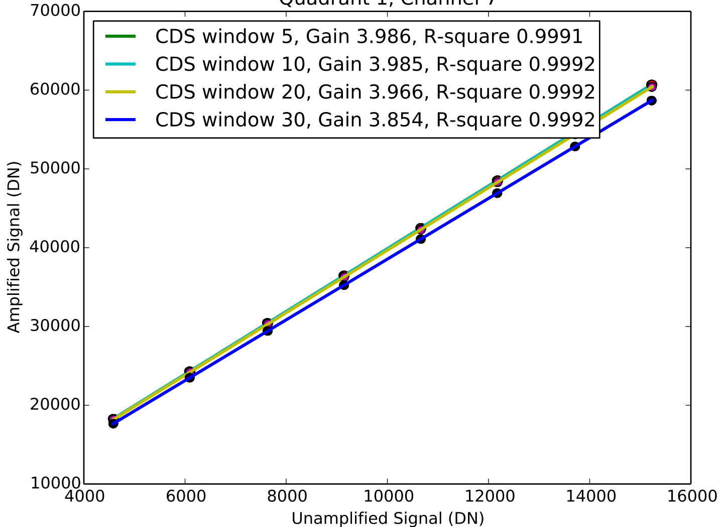
Signal vs Amplified Signal Quadrant 1, Channel 7
