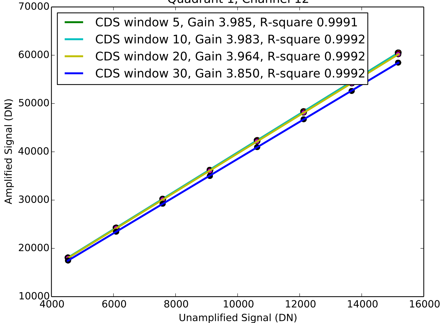
Signal vs Amplified Signal Quadrant 1, Channel 12
