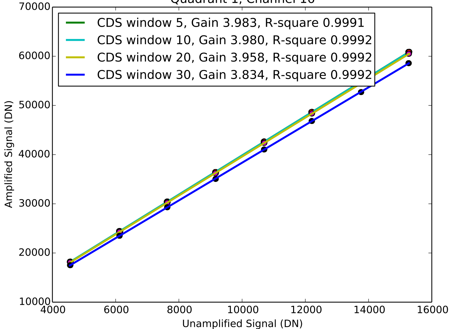
Signal vs Amplified Signal Quadrant 1, Channel 16
