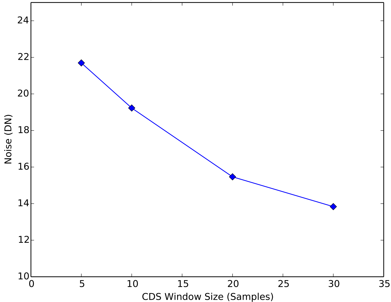
Amplifier Noise vs CDS Window Quadrant 1, Channel 1
