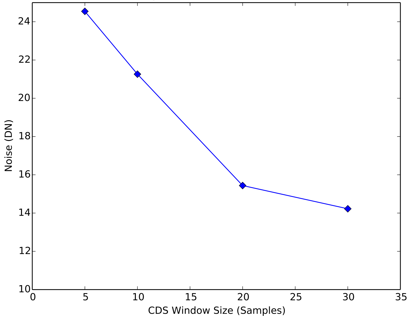
Amplifier Noise vs CDS Window Quadrant 1, Channel 13
