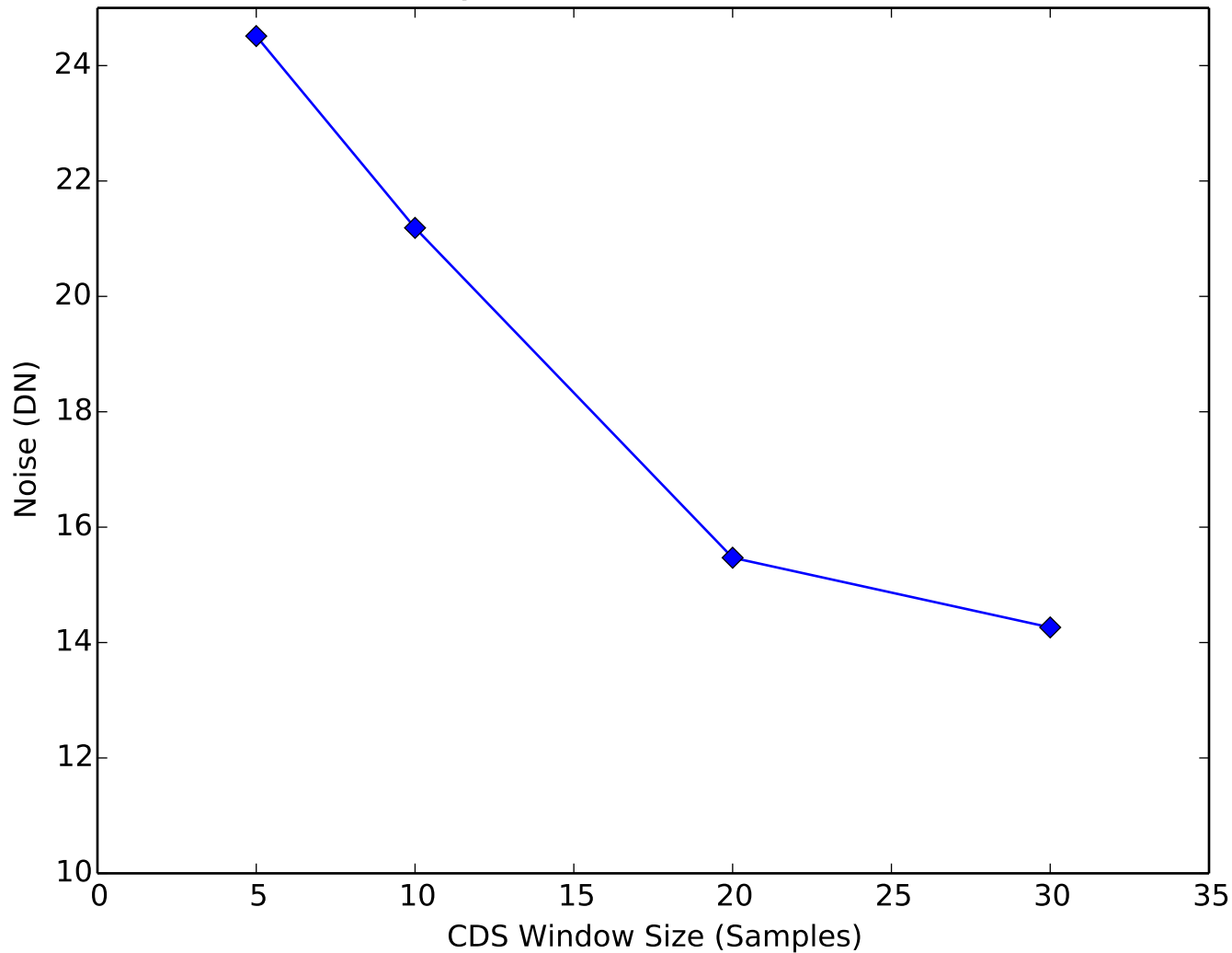
Amplifier Noise vs CDS Window Quadrant 1, Channel 15
