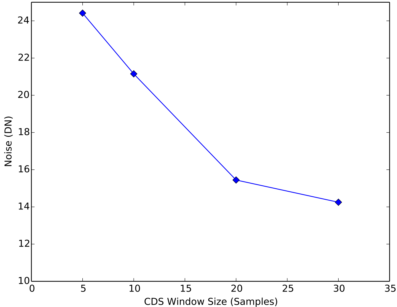
Amplifier Noise vs CDS Window Quadrant 1, Channel 9
