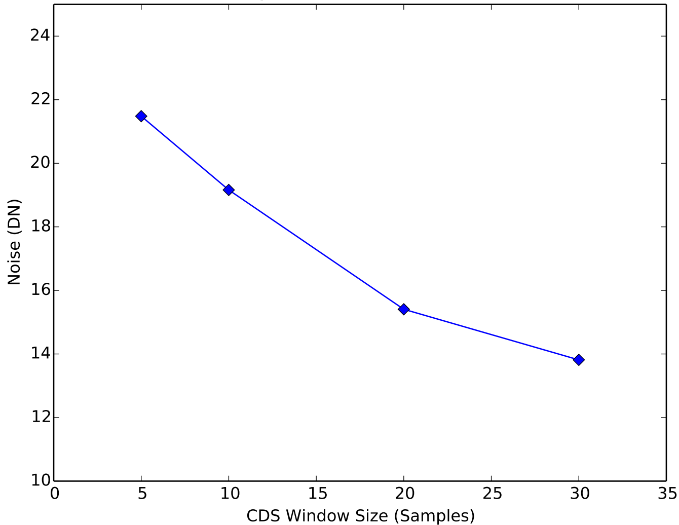
Amplifier Noise vs CDS Window Quadrant 1, Channel 4
