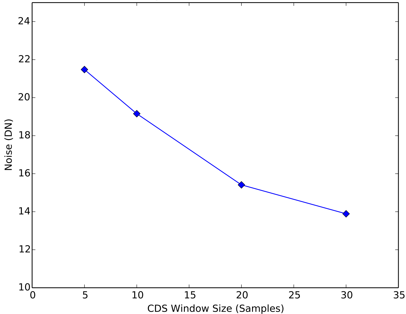
Amplifier Noise vs CDS Window Quadrant 1, Channel 5
