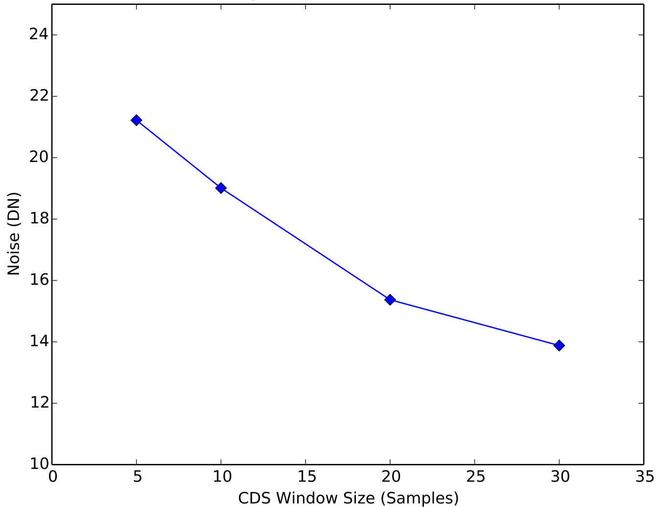
Amplifier Noise vs CDS Window Quadrant 1, Channel 8
