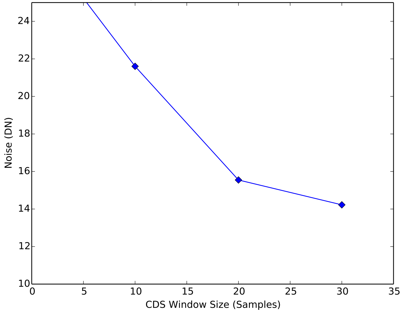
Amplifier Noise vs CDS Window Quadrant 1, Channel 10
