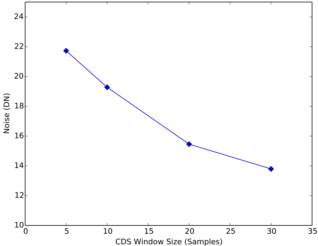
Amplifier Noise vs CDS Window Quadrant 1, Channel 2
