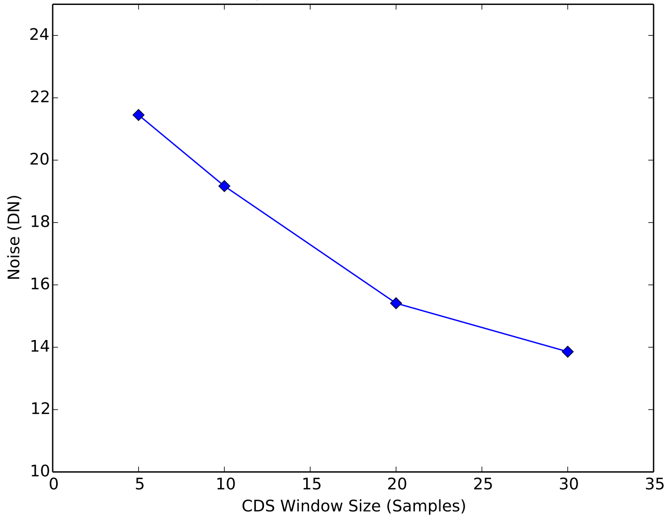
Amplifier Noise vs CDS Window Quadrant 1, Channel 6
