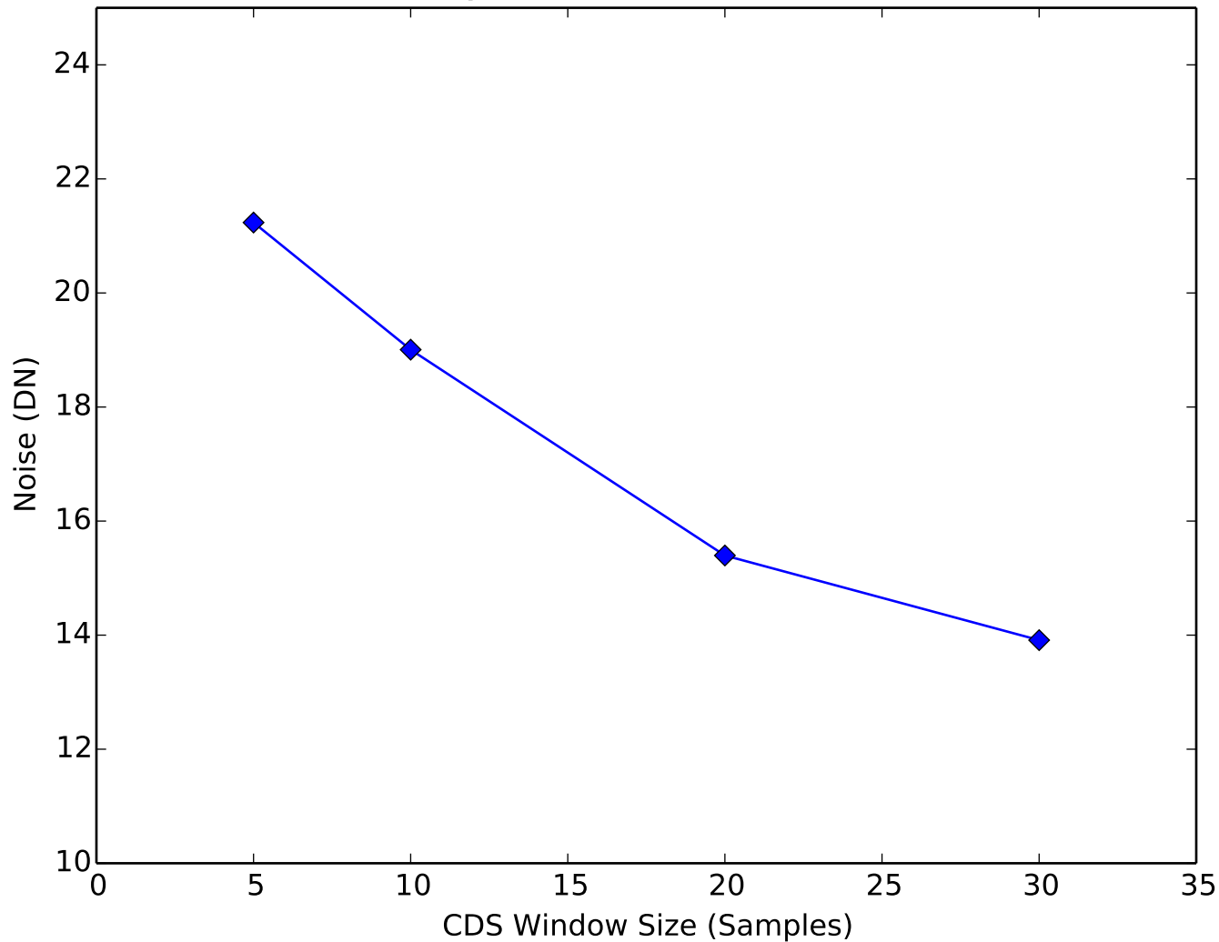
Amplifier Noise vs CDS Window Quadrant 1, Channel 7
