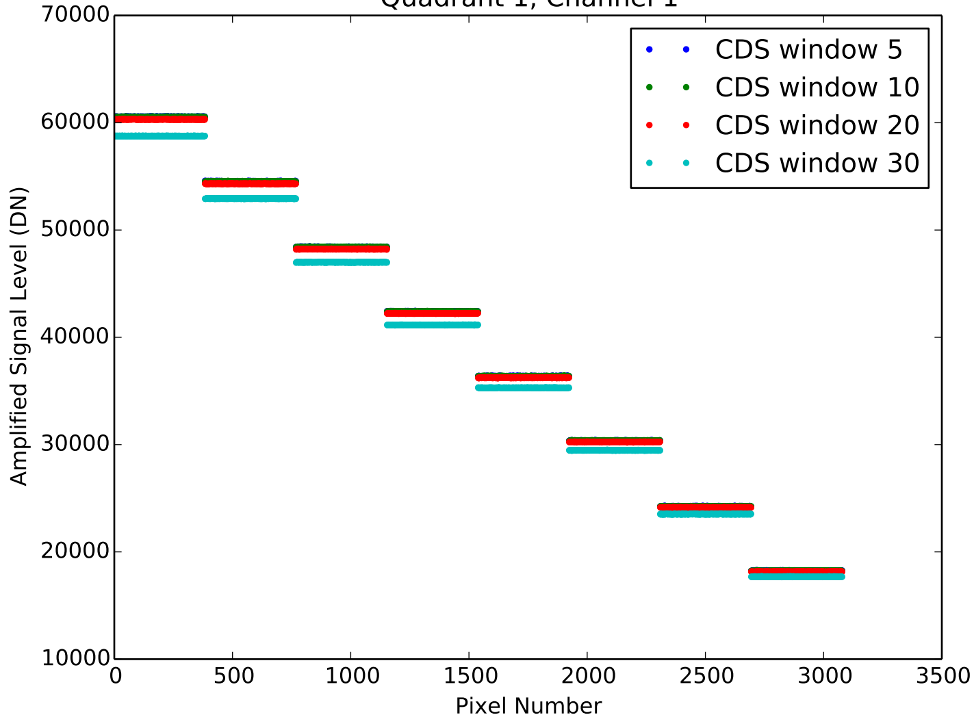
Amplified Signal Level from CDS Quadrant 1, Channel 1
