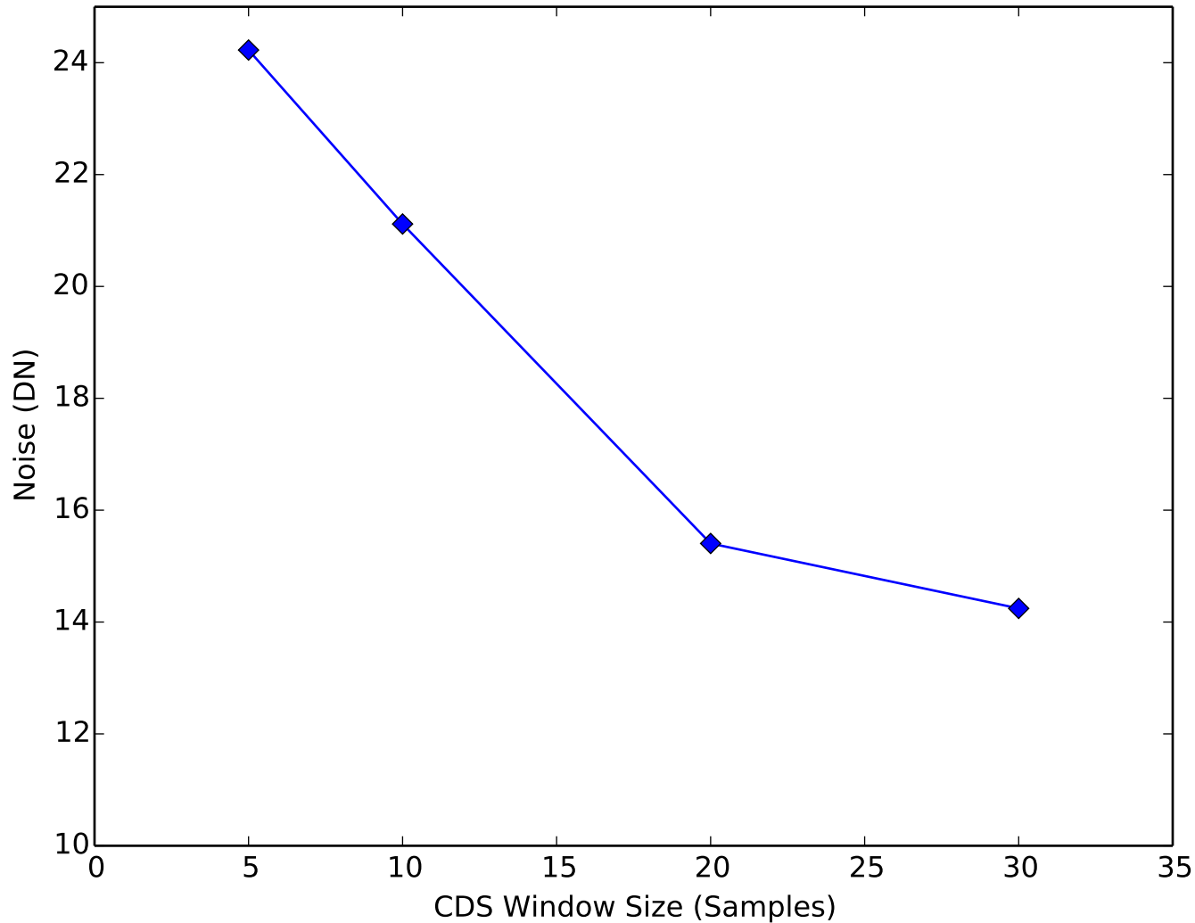
Amplifier Noise vs CDS Window Quadrant 1, Channel 14
