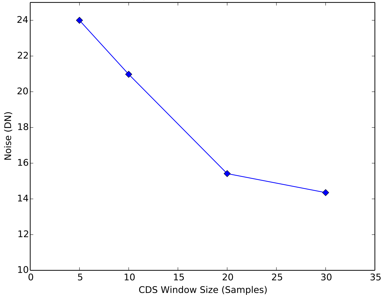
Amplifier Noise vs CDS Window Quadrant 1, Channel 16
