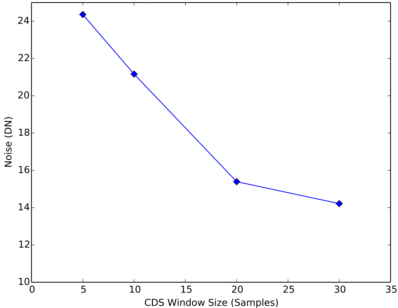
Amplifier Noise vs CDS Window Quadrant 1, Channel 12
