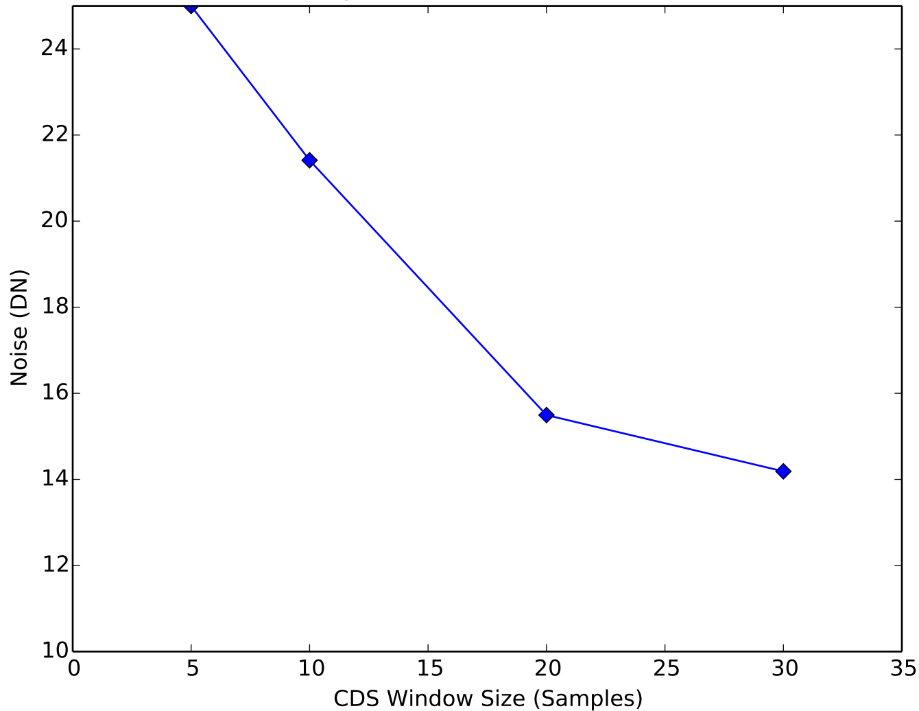
Amplifier Noise vs CDS Window Quadrant 1, Channel 11
