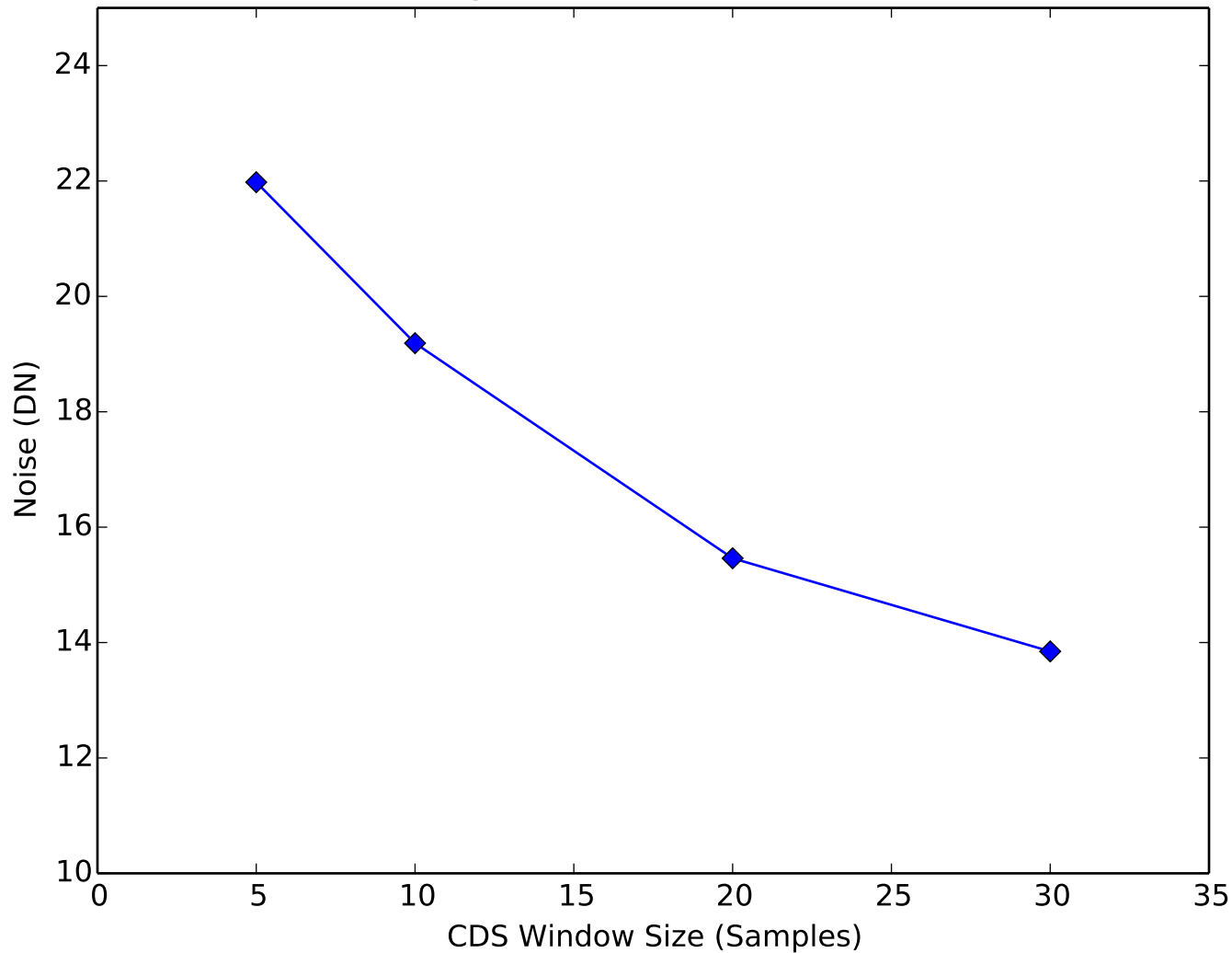
Amplifier Noise vs CDS Window Quadrant 1, Channel 3
