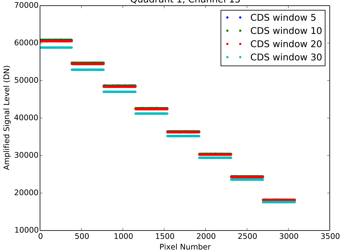
Amplified Signal Level from CDS Quadrant 1, Channel 15
