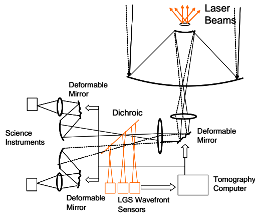
Figure 2 Hybrid MCAO/MOAO configuration.
