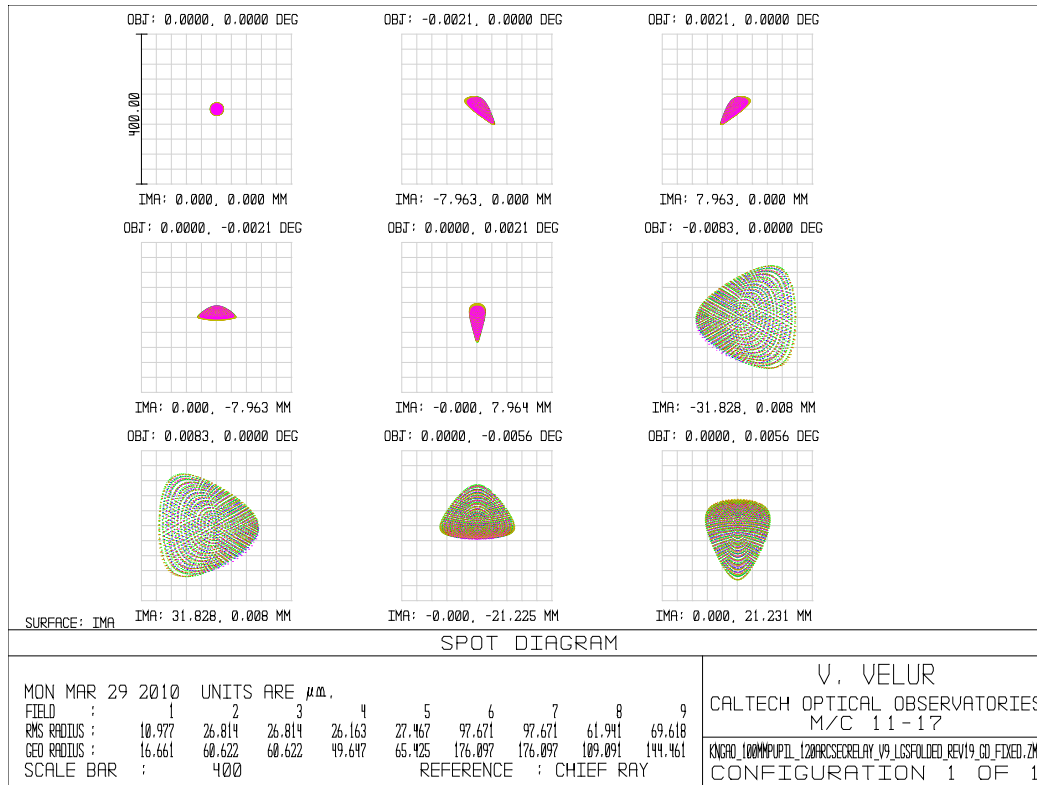
Figure 6 Spot diagram at the NGSWFS pick off focus showing 97 \mu\text{m} RMS(worst case) radius spots at a focal plane with 1.06 mm/'' plate scale.
