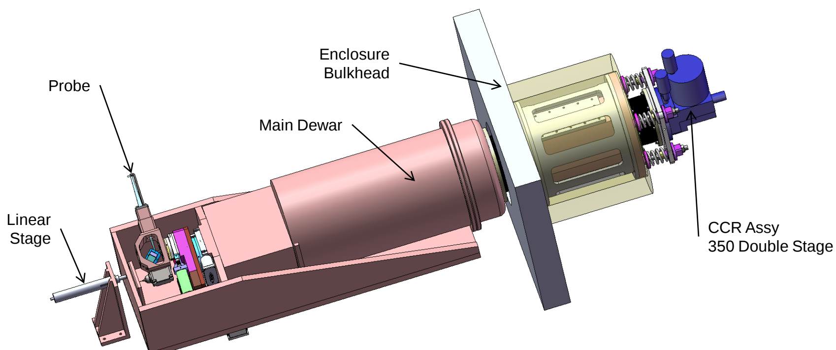
Top View
