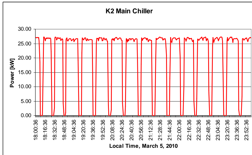
Figure 4: Keck II Main Chiller Usage
