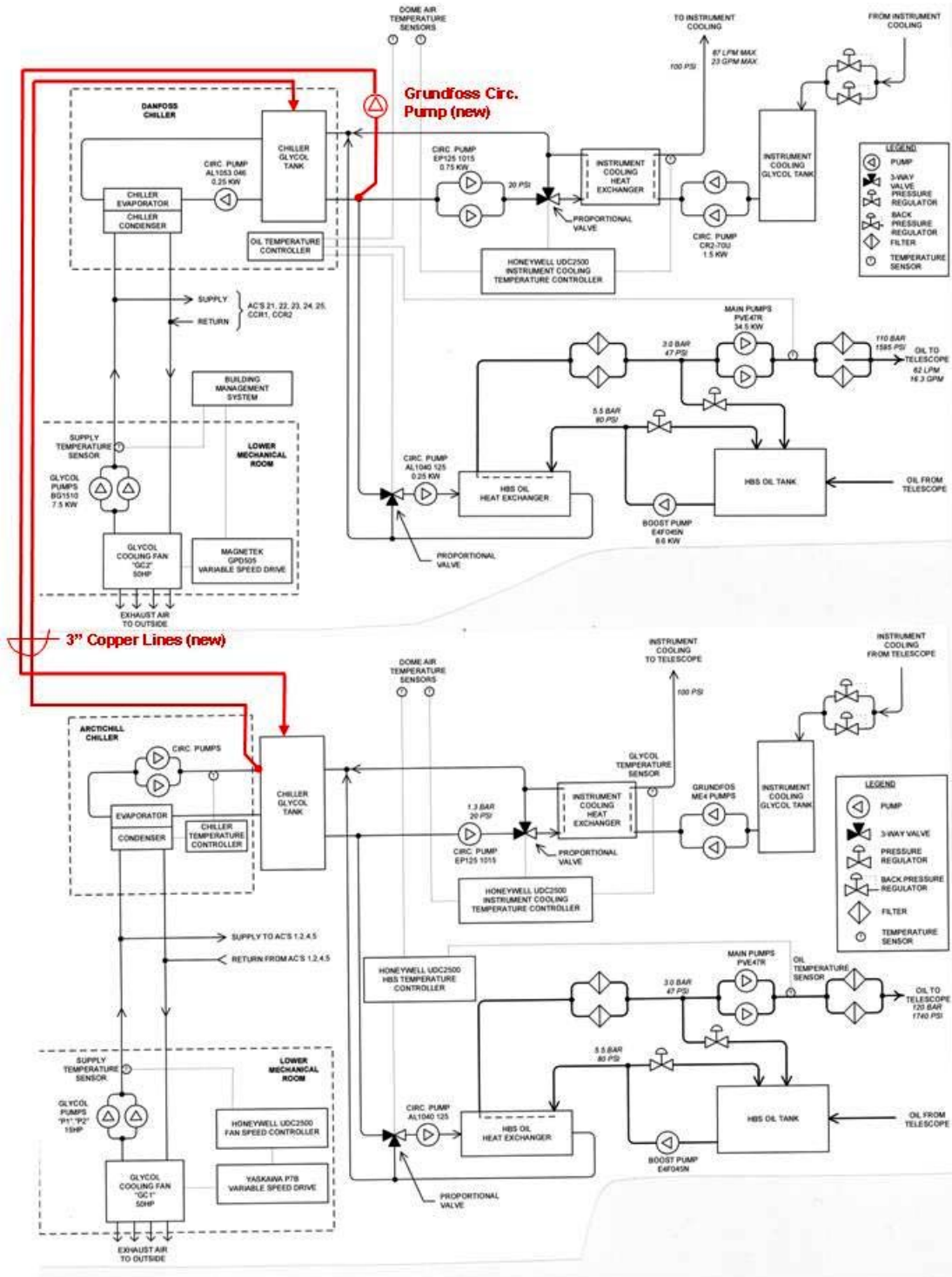
Figure 3: Proposal to Interconnect Keck I and Keck II Glycol Systems
