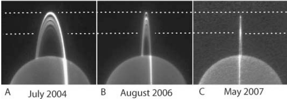
Figure 18. Comparison of the lit and unlit sides of the rings of Uranus. (A) The lit side in early July 2004. (B) The lit side on 1 August 2006. (C) The unlit side on 28 May 2007. The planet was scaled to the same size in all three images. The dotted lines show the position of the \epsilon ring (upper line) and \zeta ring (lower line). From de Pater et al. (2007).
