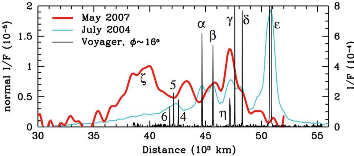
Figure 19. Temporal evolution of the Uranus rings. Comparison of the 2007 deconvolved ( i.e. , onion-peeled) radial profile averaged over both north and south sides (red; smoothed radially over \sim 650 km), with the northern profile from 2004 (cyan), and the Voyager profile in backscattered light (black). We shifted the Voyager \epsilon ring to match the Keck profile, compensating for its large eccentricity. The left axis shows the I/F normal to the ring plane of the 2007 profile. The axis on the right side shows the measured I/F for the 2004 data. The scale for the Voyager data is arbitrary (and off-scale for \epsilon ). The Voyager data were smoothed to match the Keck pixel size. From de Pater et al. (2007).
