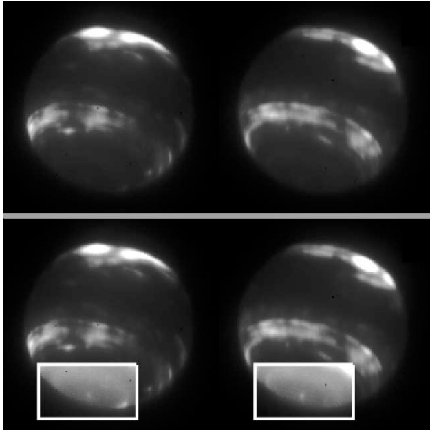
Figure 16. Neptune with Keck in 2005. The planet's disk subtends only 2.3 arcseconds. Upper pair: these H-band images of Neptune were obtained with the Keck NGS AO system and NIRC2 on 5 July (11:16 UT, left; 13:34 UT, right). They show tropospheric clouds at midlatitudes in both hemispheres. Lower pair: The south polar regions of the images were enhanced by a factor of 2.6 to show that the zonal circulation pattern continues right to the pole. Similar images, taken in 2001, were used by Martin et al. (2007) to study the detailed structure of the zonal wind profile by tracking dozens of the tiny discrete features. From Hammel et al. (2007).
