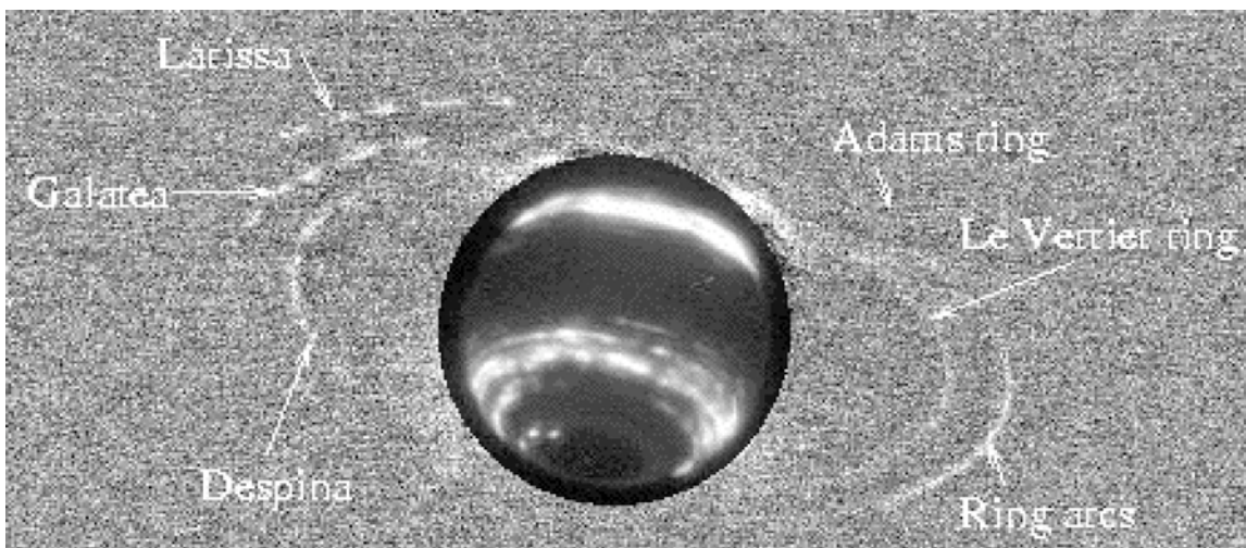
Figure 20. Keck observations of Neptune's rings. This composite image of July 2002 Keck AO data (K' band, total integration time of 33 minutes) shows satellites, ring arcs, and the complete Adams and Le Verrier rings. The images have been high-pass filtered by subtracting the same image median-smoothed with a width of 50 pixels. This procedure removes diffuse scattered light, and brings out small-scale features. Neptune is highly saturated in this composite exposure; here the saturated planet has been cropped and a 1-minute exposure of Neptune itself is shown in its place. From de Pater et al. (2005).
