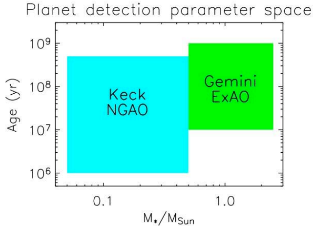
Figure 6 Schematic illustration of the parameter space of Keck NGAO and of the Gemini Planet Imager for direct imaging of extrasolar planets.
