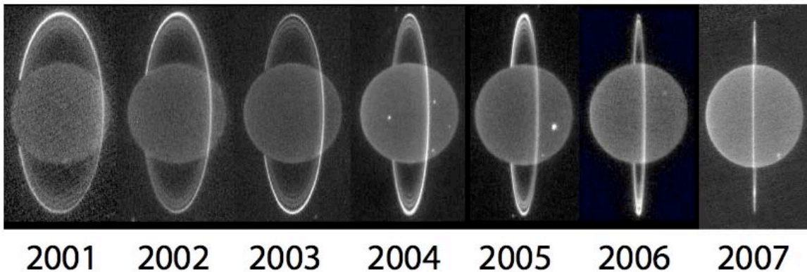
Figure 17. Annual images of the rings of Uranus from Keck. The last RPX was in 1965, and the next will occur in 2049. White spots in these K'-band images are high-altitude cloud features. Adapted and updated from de Pater et al. (2006).
