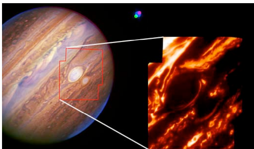
Figure 11. Jupiter's Great Red Spot and new Red Oval with the Keck AO system. Left: This false-color near-infrared composite of Jupiter and Io was taken in July 2006. The AO system used Io as its reference star. Io itself is visible as the green, blue, and red dots, corresponding to 1.29, 1.65 and 1.58 \mu\text{m} , respectively (Io's blue dot looks larger). The motion of the satellite with respect to Jupiter during the observing sequence is clearly seen. The red outline shows the area covered by the mosaic shown on the right. Right: The two spots were also imaged with AO through a 5- \mu\text{m} filter that samples thermal radiation from below the main cloud deck. Both spots appear dark because clouds block heat emanating from lower elevations, though narrow regions around the spots that are cloud-free show leakage of heat into space.
