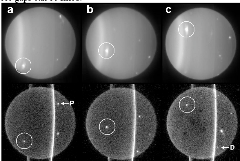
Figure 15. Keck images of Uranus in 2004. These images of the 3.7"-diameter disk of Uranus were obtained on 4 July (a, b, and c). For each pair, the upper image is H (1.6 \mu\text{m} ) and the lower image is K' (2.2 \mu\text{m} ). The south pole of Uranus is to the left. An unusual bright feature is circled in each image; tracking such features yields the zonal atmospheric velocity at that latitude. At K', images are dominated by ring flux, and uranian moons masquerade as northern cloud features (P = Portia; D = Desdemona); unarrowed white spots are small-scale cloud features. Dark splotches in (c) at K' are an artifact caused by residual charge. From Hammel et al. (2005a).
