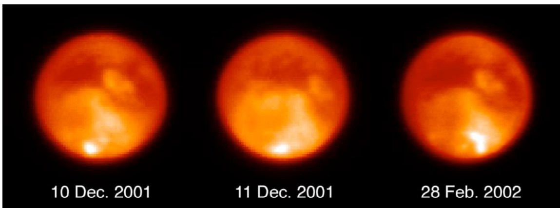
Figure 12. Keck imaging of Titan's Clouds. These K'-band images of changing methane clouds near Titan's south pole were taken using the Keck AO system in December 2001 and February 2002. Nearly the same face of the moon is viewed in all three images; the disk of Titan subtends just 0.8 arcseconds. The large storm in the Feb. 28 image is over 1400 km (870 miles) long. From Brown et al. 2002.
