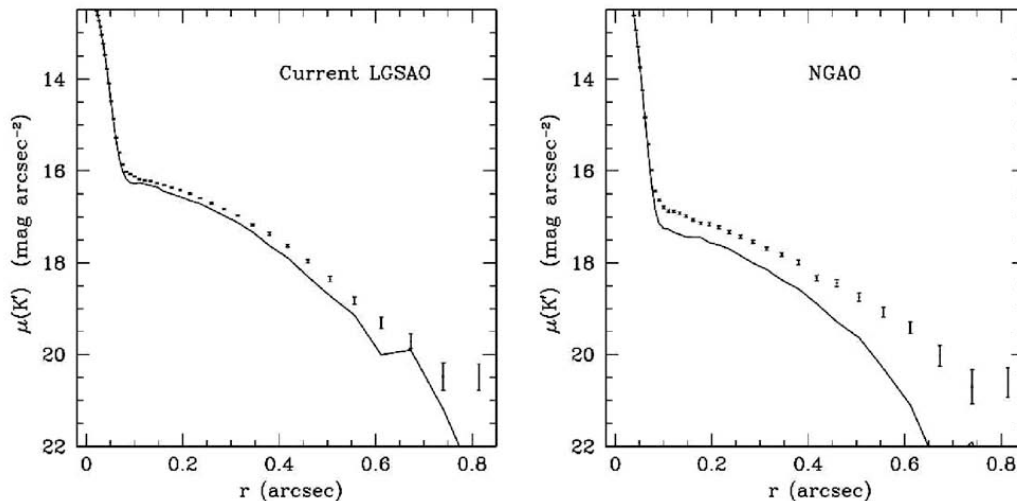
Figure 9 Simulated K' observation of a z = 2 quasar with current LGS AO and with NGAO, both for a 1 hour exposure with NIRC2 and assuming the same background level. The solid curve is the PSF profile measured from a simulated PSF image with noise added, and scaled to the same peak flux as the quasar nucleus, and the points with error bars are the radial profile of the quasar plus host galaxy. The host galaxy is nearly undetectable with current LGS AO but can be significantly detected with NGAO.
