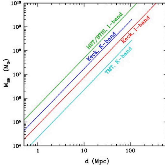
Figure 2 Minimum detectable black hole mass as a function of galaxy distance, under the assumption that the black holes follow the local M - \sigma relation, and assuming a minimum of two resolution elements across the black hole's radius of influence. For Keck NGAO, this figure assumes a PSF core with FWHM = 0.053'' in K, and 0.035'' in I. Minimum detectable black hole mass scales approximately as (\text{distance} * \text{angular resolution})^2 . For distances beyond \sim 100 Mpc, the CO bandhead is redshifted out of the K-band and is no longer observable. The line for TMT (optimistically) assumes a diffraction-limited PSF core in the K-band.
