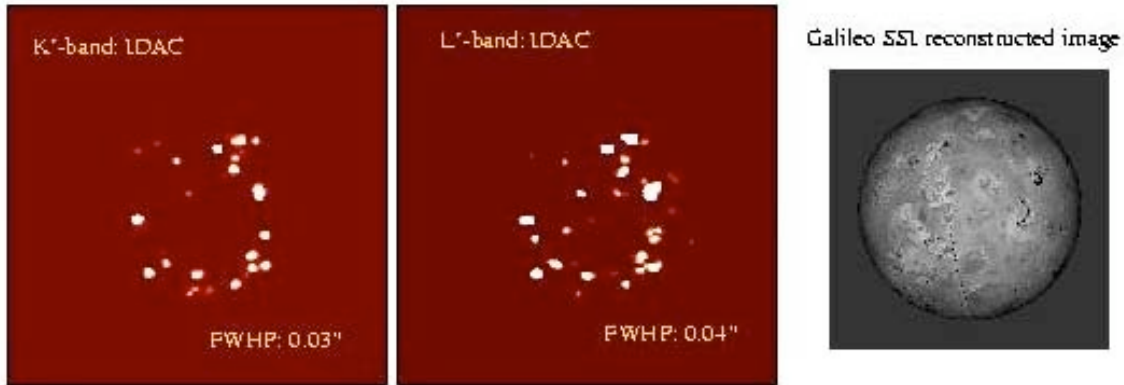
Figure 14. Keck AO images of many volcanoes on Io. Images of Io in K'- (left) and L'-bands (middle) were taken using the Keck AO system while the satellite was in eclipse; i.e., only thermal emission was detected. The images were deconvolved with the "IDAC" algorithm using a Gaussian beam with a FWHM of 0.03" at K'-, and 0.04" at L'-band. All images have been rotated so Io's north pole is up. On the right side of the figure we show a Galileo visible-light SSI reconstructed image at the time of the observations. From de Pater et al. (2004).
