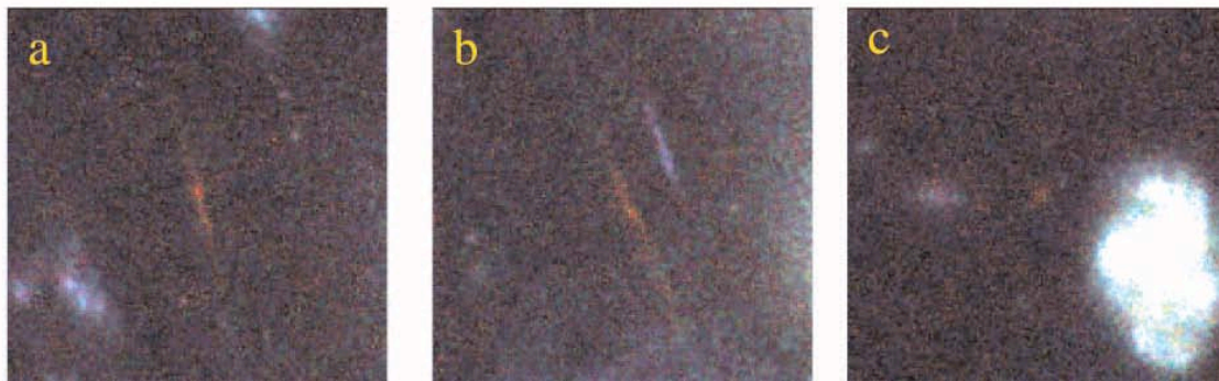
Figure 10 Pseudocolor image of highly magnified lensed sources in the Abell cluster 2218 (from Kneib et al. 2004). The red curves show the critical lines of infinite magnification for sources placed at z=5.576 and 7.0 . Images a, b, and c show a multiply imaged source at z=7 . The unlabeled circles at the top of the image mark the multiply imaged source found by Ellis et al. (2001) at z=5.576 .
