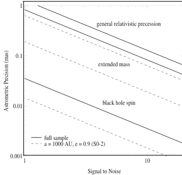
Figure 4. Required astrometric precision for detecting, from top to bottom, GR effects associated with relativistic prograde precession, extended mass within the stellar orbits, and frame-dragging effects due to BH spin (based on Weinberg et al. 2005). Estimates are based on measurements of stellar orbits and positions from Keck diffraction-limited images (thick, solid lines), and assume radial velocity measurement errors of 10 km/s. The stellar orbits include 16 stars within 0.5'' of Sgr A* with orbital fits obtained from speckle imaging measurements and 142 stars within 1'' of Sgr A* with stellar positions obtained with new, deep AO maps. For comparison, we also show estimates based on measurements from just the short-period star S0-2 (thin, dashed line). Results are for a 10-year baseline with 10 integrations per year. Low-order GR and extended matter effects are detectable at the >7\sigma level if an astrometric precision of \sim 100 \mu\text{as} can be achieved. Detection of BH spin requires either better precision or, at \sim 100 \mu\text{as} precision, improved SNR obtained by observation of multiple as-yet-undiscovered high-eccentricity, short-period stars over multiple orbits.
