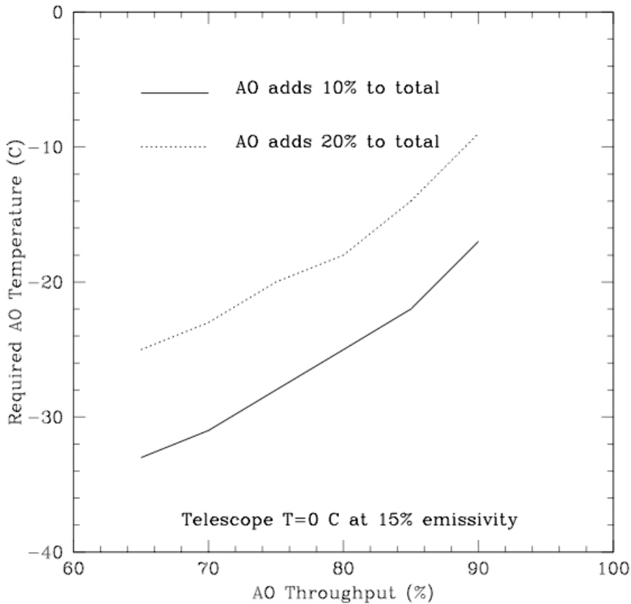
Figure 1 Required AO system temperature as a function of AO throughput to minimize impact of thermal radiation on the net K-band background.
