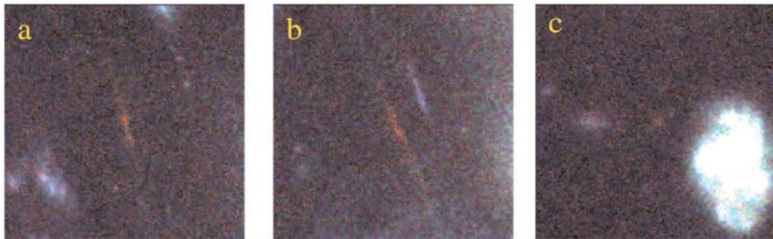
Figure 11 Pseudocolor image of highly magnified lensed sources in the Abell cluster 2218 (from Kneib et al. 2004). The red curves show the critical lines of infinite magnification for sources placed at z=5.576 and 7.0 . Images a, b, and c show a multiply imaged source at z=7 . The unlabeled circles at the top of the image mark the multiply imaged source found by Ellis et al. (2001) at z=5.576 .
