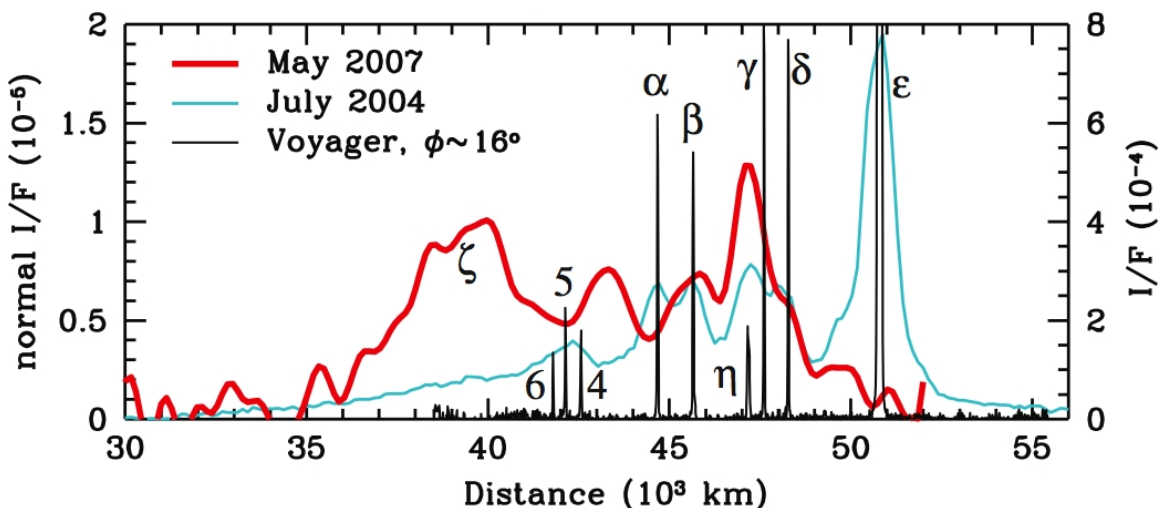
Figure 20. Temporal evolution of the Uranus rings. Comparison of the 2007 deconvolved ( i.e. , onion-peeled) radial profile averaged over both north and south sides (red; smoothed radially over \sim 650 km), with the northern profile from 2004 (cyan), and the Voyager profile in backscattered light (black). We shifted the Voyager \epsilon ring to match the Keck profile, compensating for its large eccentricity. The left axis shows the I/F normal to the ring plane of the 2007 profile. The axis on the right side shows the measured I/F for the 2004 data. The scale for the Voyager data is arbitrary (and off-scale for \epsilon ). The Voyager data were smoothed to match the Keck pixel size. From de Pater et al. (2007).
