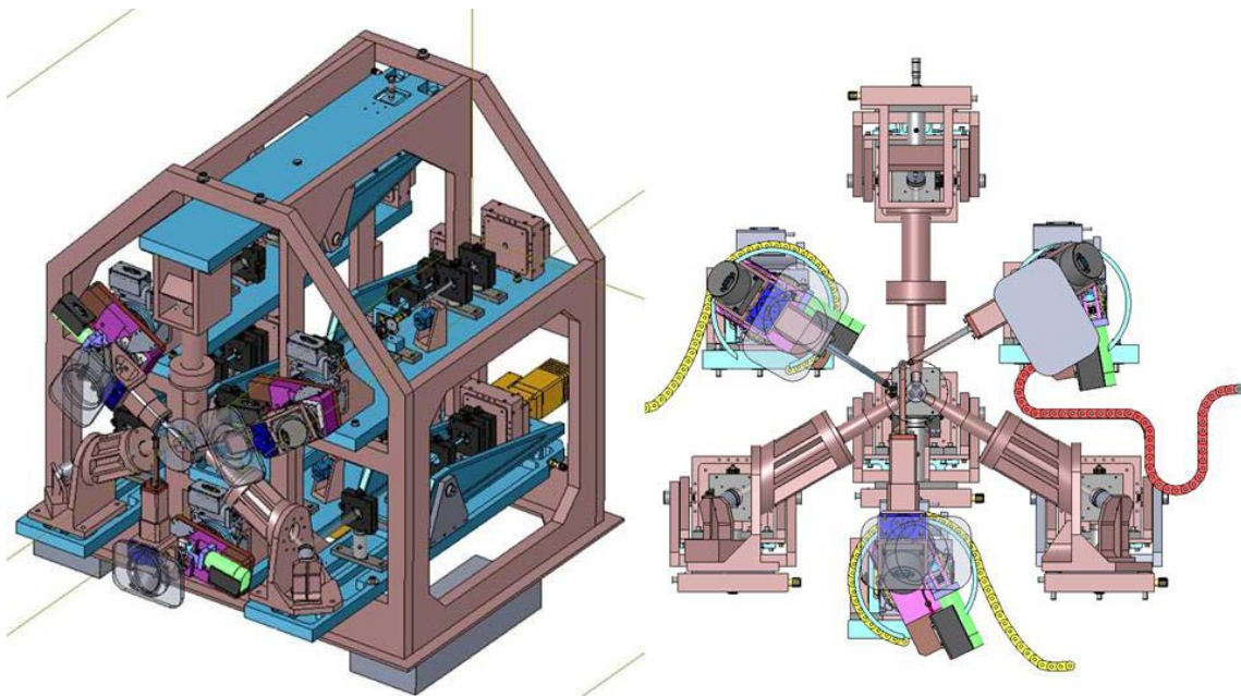
Figure 7: LGS wavefront sensor assembly perspective (left) and front view (right). Four fixed and 3 patrolling LGS WFS mounted on a common focus tracking stage.
