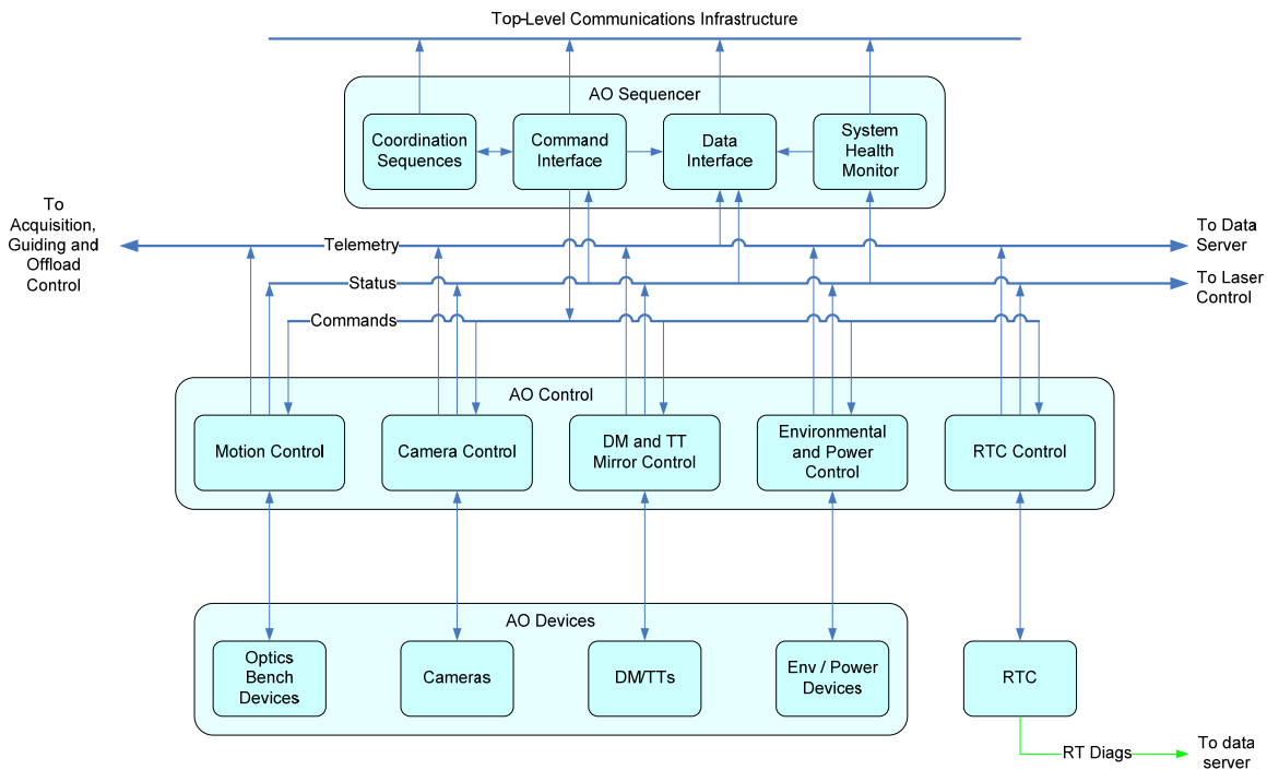
Figure 44. AO systems control hierarchy block diagram.
