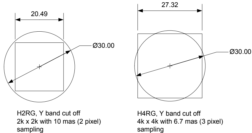
Figure 62: Near-IR imager FOV options (All dimensions in arc seconds)
