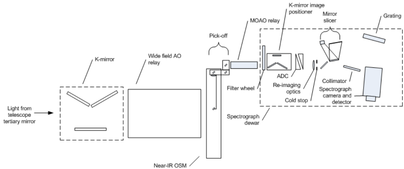
Figure 60: d-IFS block diagram
