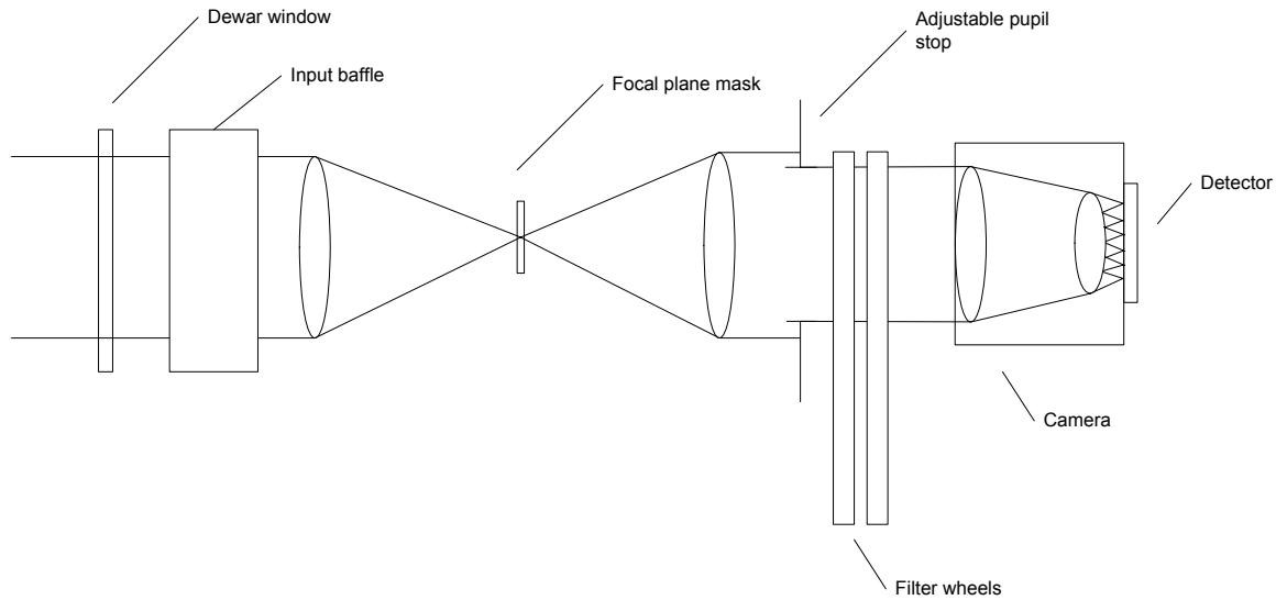
Figure 63: Near-IR imager block diagram
