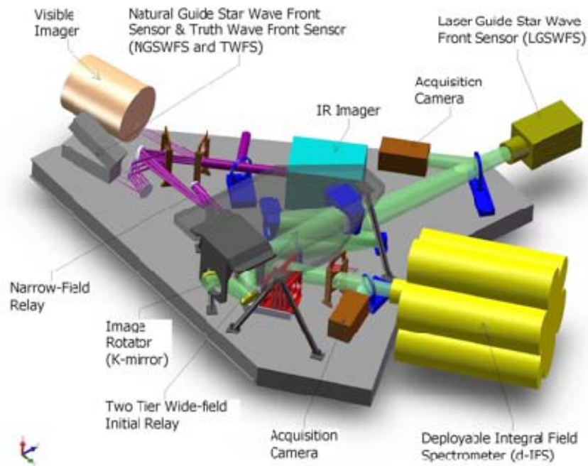
Figure 5. AO system optical layout perspective view (SolidWorks). The optical path through the low order “wide” field relay and the high order “narrow” field relay are shown in green and purple, respectively. Light from the telescope enters through the image rotator.
