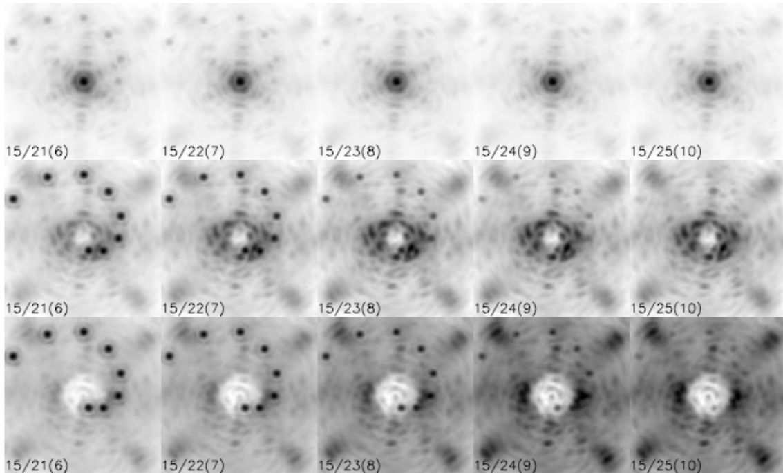
Figure 67. Simulated NGAO J-band science observations with secondary objects inserted. Top row: AO without coronagraph; middle row: AO + coronagraph with 6 \lambda/D occulation; bottom row: AO + coronagraph with 10 \lambda/D occulation. The numbers in the lower left corner of each image indicate the primary
