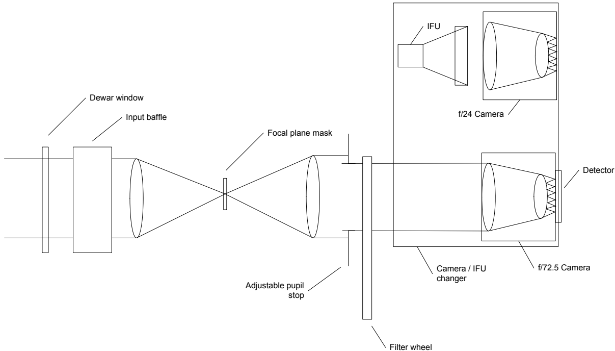
Figure 64: Visible imager block diagram
