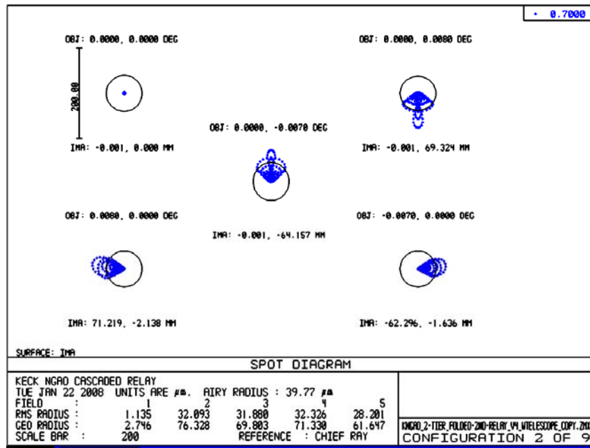
Figure 23. Spots at the on-axis and extreme field angles to the NGS WFS.
