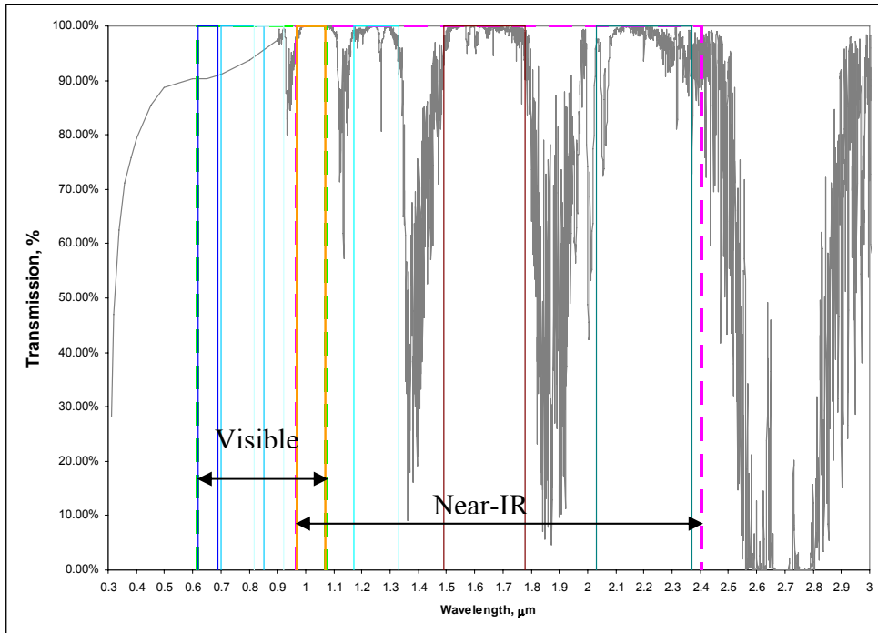
Figure 59: NGAO Passbands
