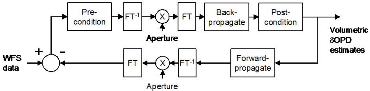
Figure 52. Tomography algorithm.
