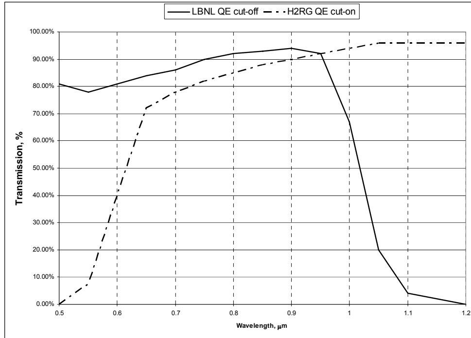
Figure 61: Detector QE cut-on and cut-off characteristics
