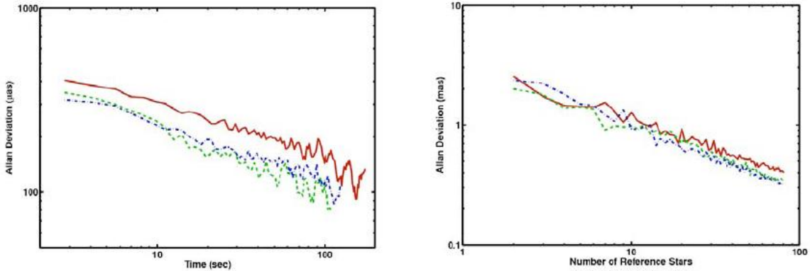
Figure 23. Astrometric Accuracy for Bright Targets
