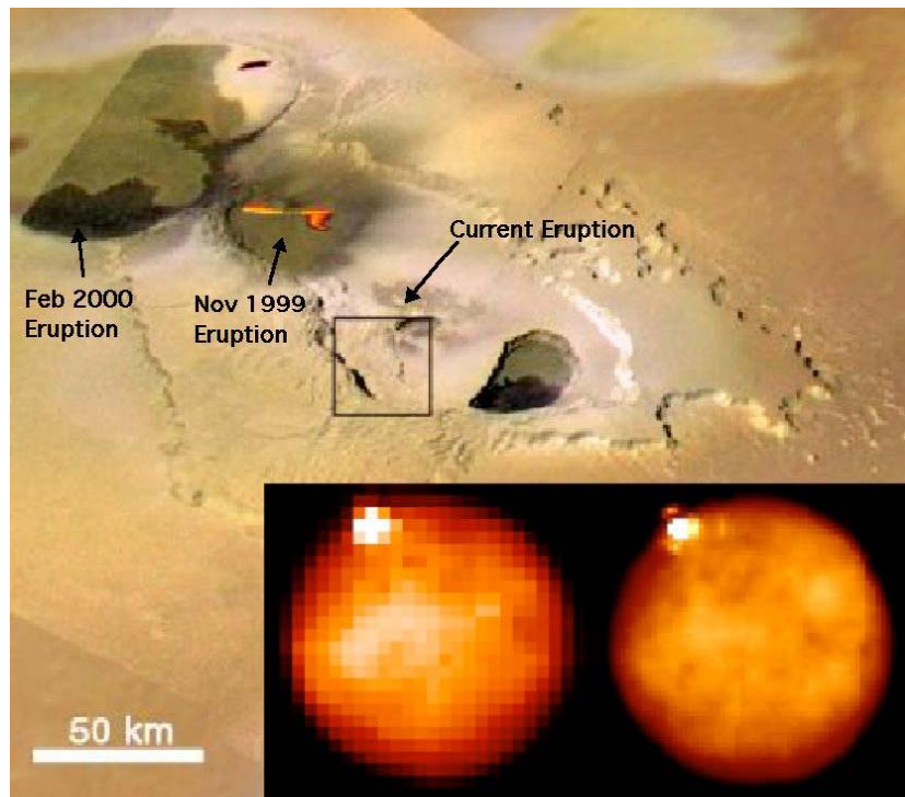
Figure 38. Keck OSIRIS images of Tvashtar erupting on Io.
