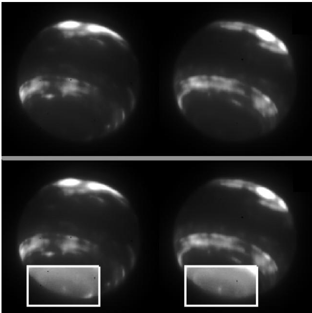
Figure 41. Neptune with Keck in 2005.
