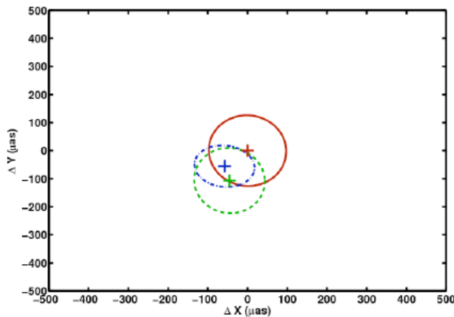
Figure 24. Astrometric precision over a 2 month time-span.
