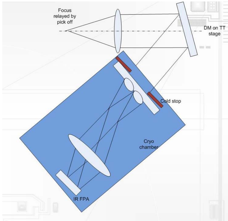
Figure 8 Schematic of the TTFA showing the cold stop and cryogenic part and the front cold end (there is a window between the cold and the cryogenic chamber).
