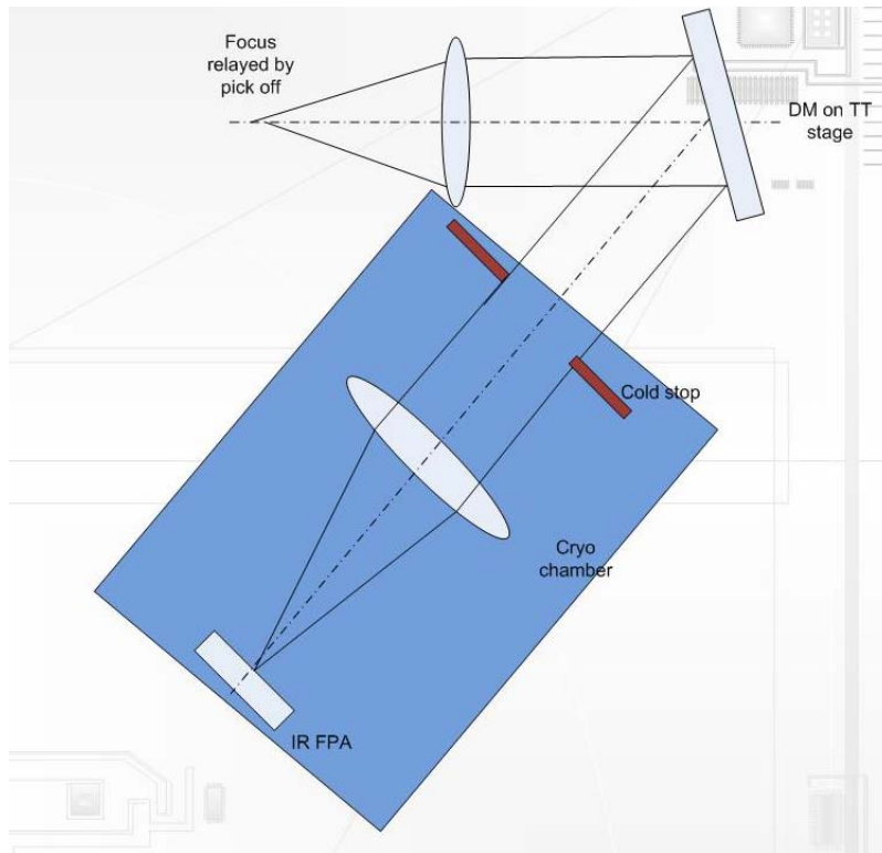
Figure 9 Schematic of the TT sensor design (there is a window between the cold and the cryogenic chamber).
