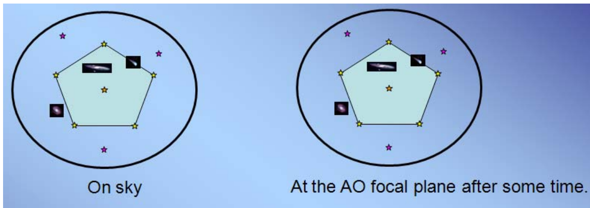
Figure 6 Wide-field observing scenario – K mirror keeps the stars fixed on the AO focal plane(s) and hence on the WFS channels. NGAO keeps the LGS stars fixed with respect to the sky and at the detector at all times when observing in WF mode.
