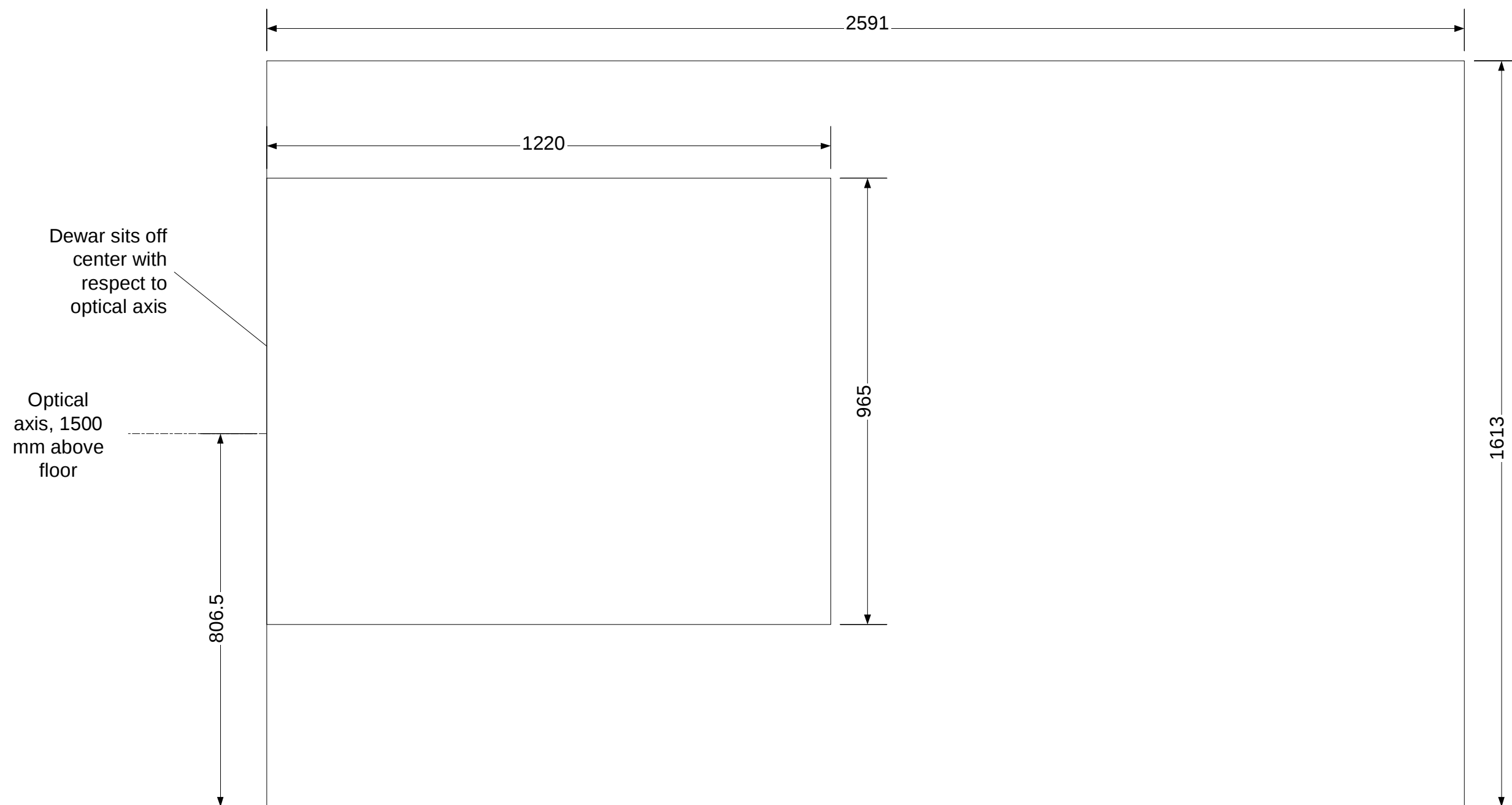
Top view
