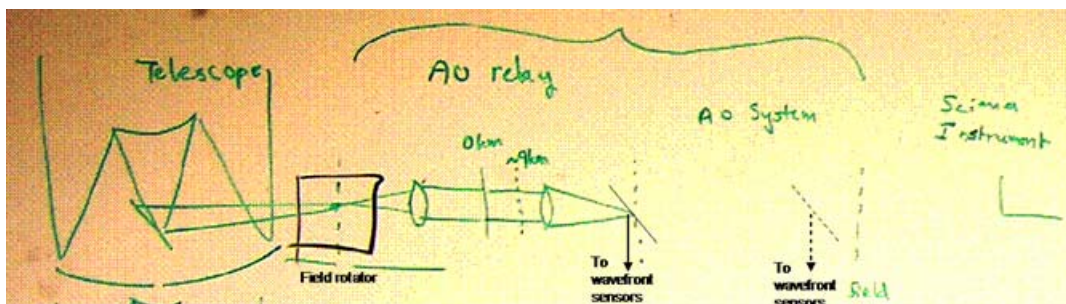
Figure xxx. Generic “conventional” architecture. The AO system is on the Nasmyth. Component blocks are the field rotation mechanism (K mirror), large AO relay which handles the largest field of regard for any downstream science instrument and containing one or more conjugate deformable mirrors, followed by the a possible secondary AO system that might be specialized to the science, e.g. MOAO units, then followed by the science instrument. The front-end relay can act as a common “woofer.”
