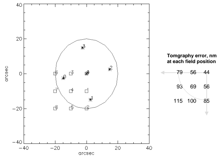
Figure xxx. Tomography error in the narrow-field AO system (5 LGS on 30 arcsecond diameter). See Figure 3c for a plot of the generalized anisoplanatism with 3 DMs.
