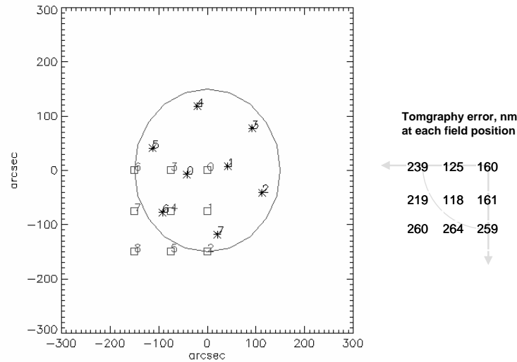
Figure xxx. Tomography error in the wide-field AO system (8 LGS on 240 arcsecond diameter).
