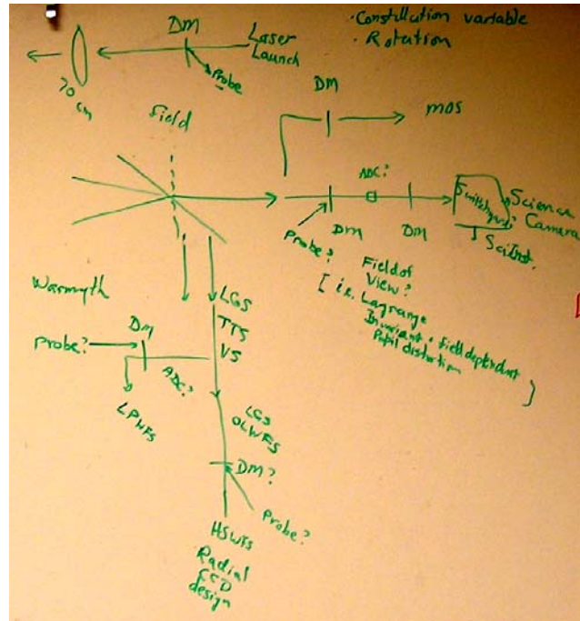
Figure xxx. Generic open loop architecture. Laser and natural guidestars are picked off at the telescope focal plane and sent to the various wavefront sensors. On the science leg are multi-conjugate or multi-object deformable mirror paths.
