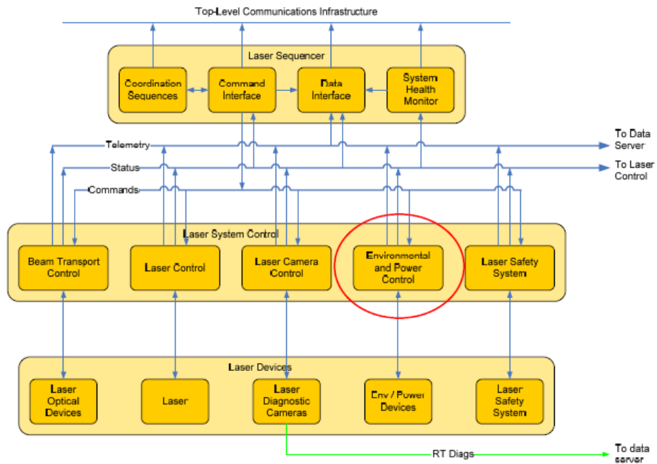
Figure 2: Laser Environmental and Power Control/Monitoring
