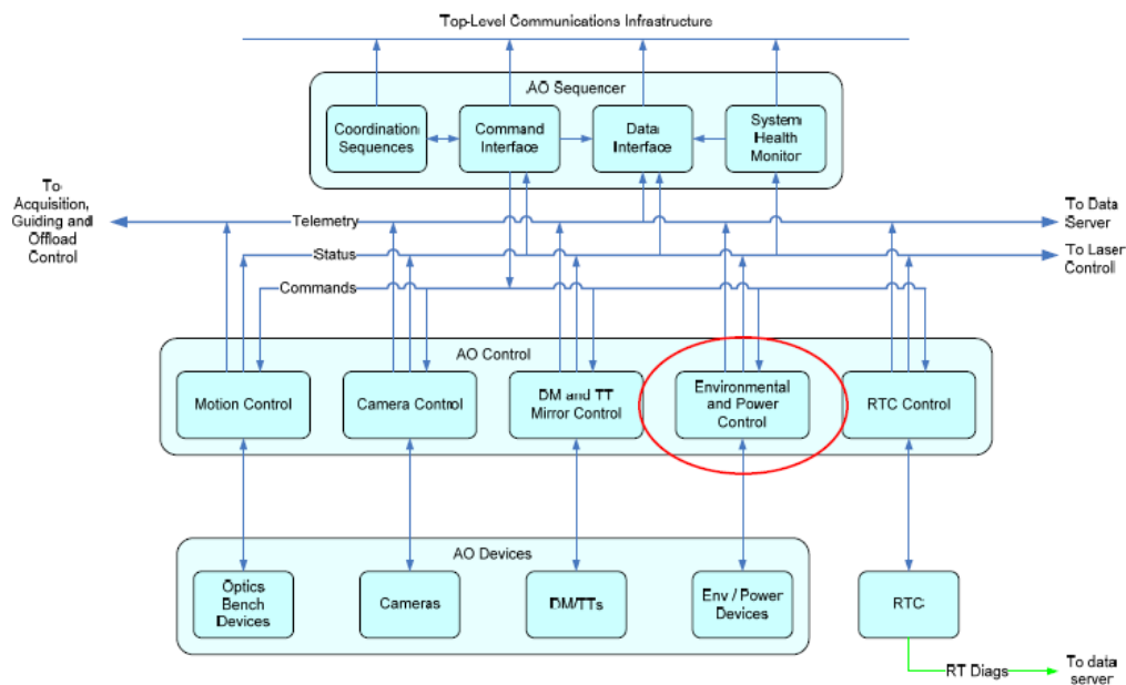
Figure 1: AO Environmental and Power Control/Monitoring
