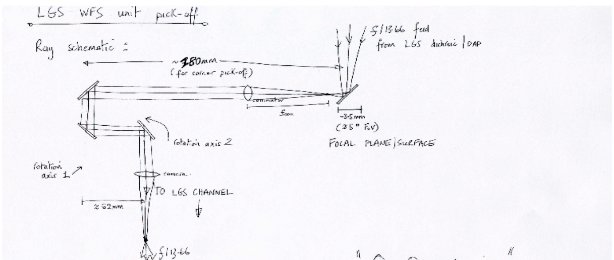
Figure 5 Schematic that unravels the theta mechanism.
